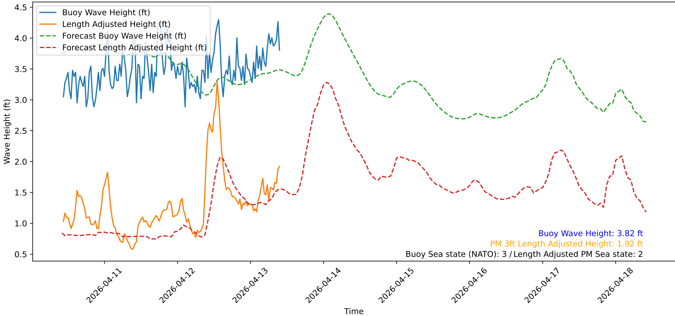
Wave Heights over Time for Red Beach at 2026-04-13 10:20:52
