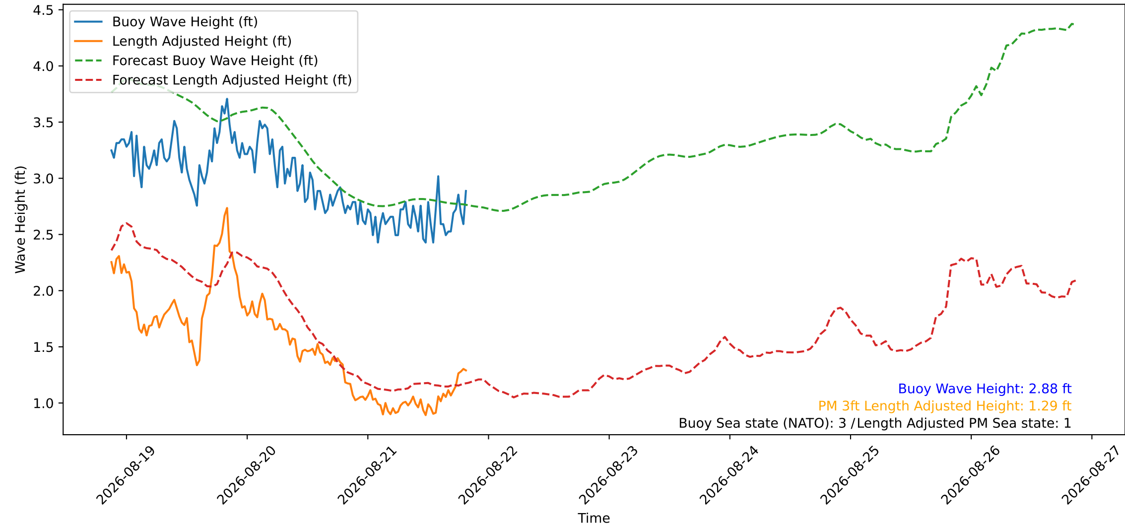
Wave Heights over Time for Green Beach at 2026-08-21 20:31:08
