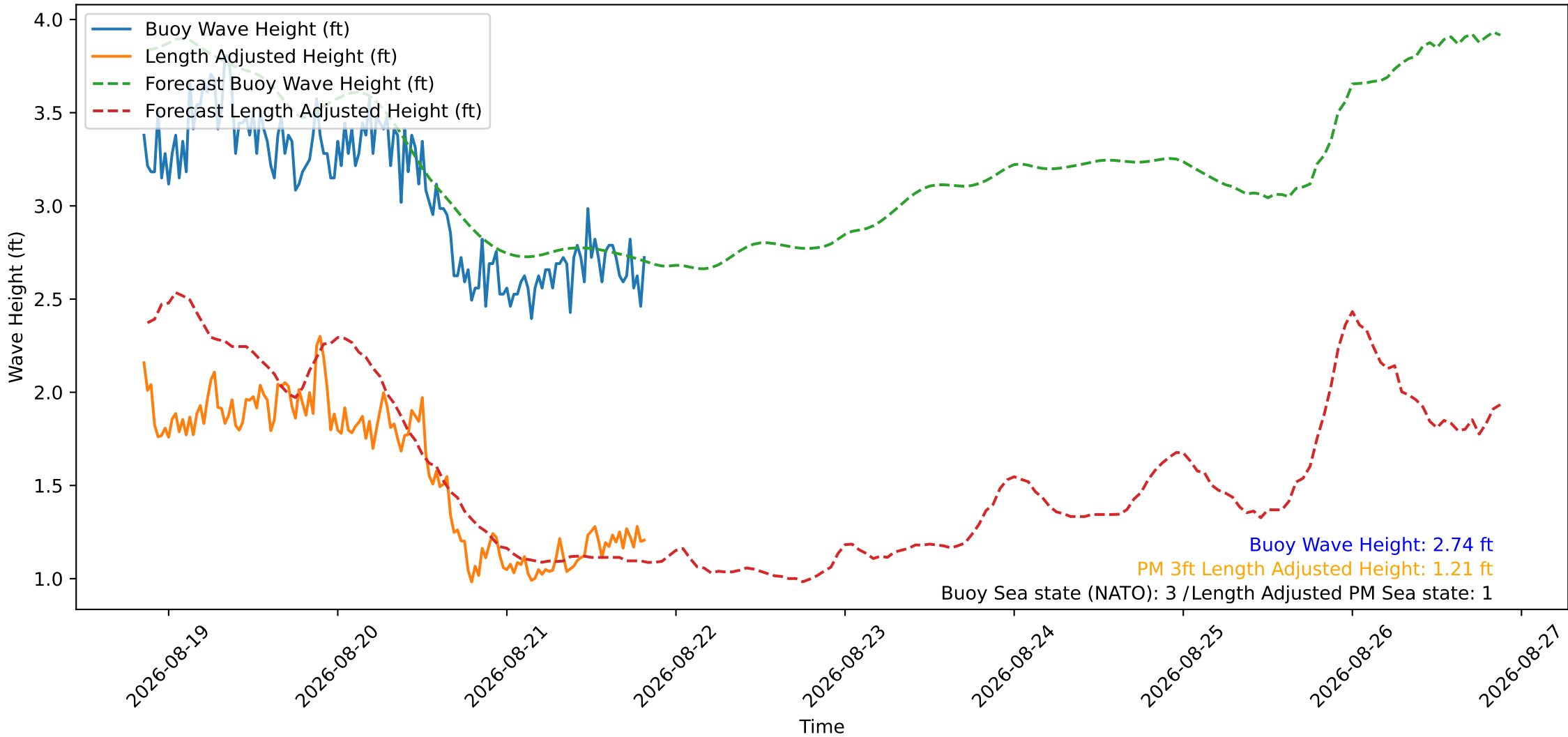
Wave Heights over Time for Oceanside Harbor at 2026-08-21 20:30:26
