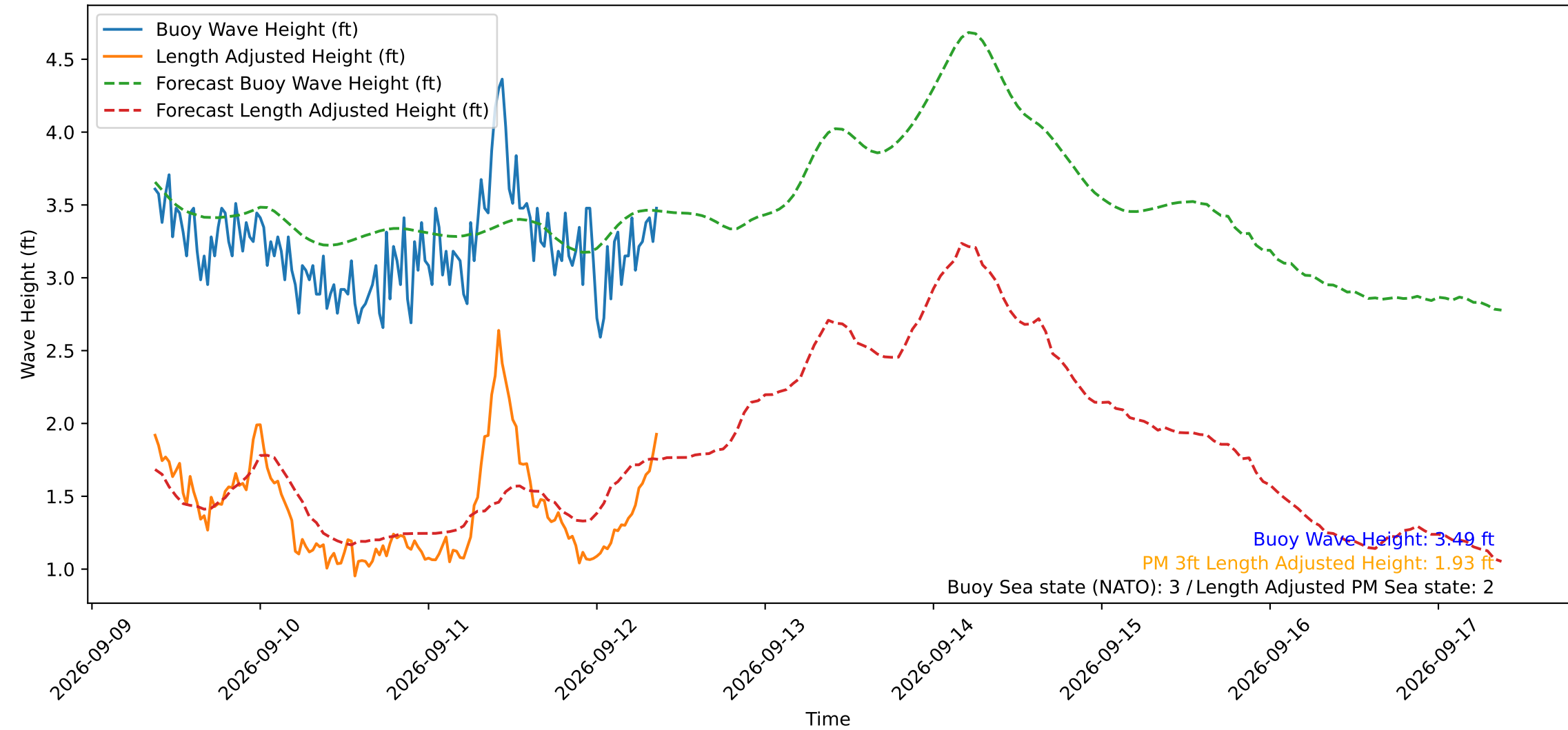
Wave Heights over Time for Oceanside Harbor at 2026-09-12 09:00:30
