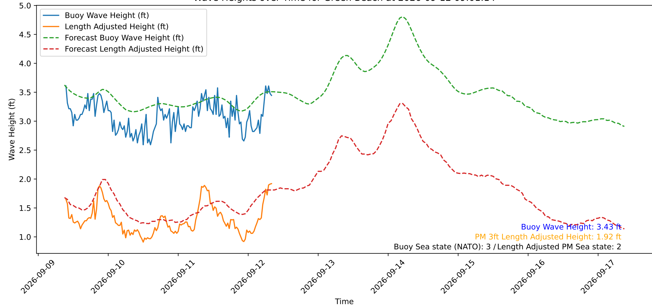
Wave Heights over Time for Green Beach at 2026-09-12 09:01:14
