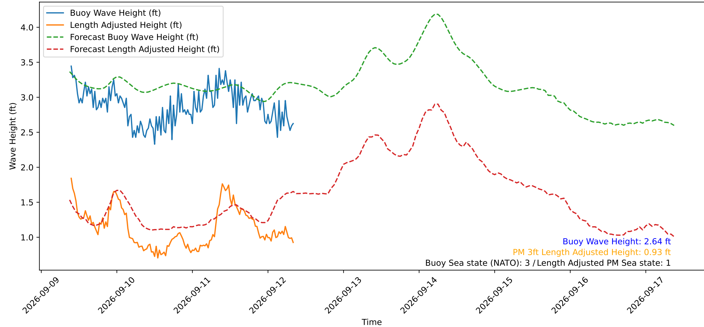
Wave Heights over Time for Red Beach at 2026-09-12 09:00:50
