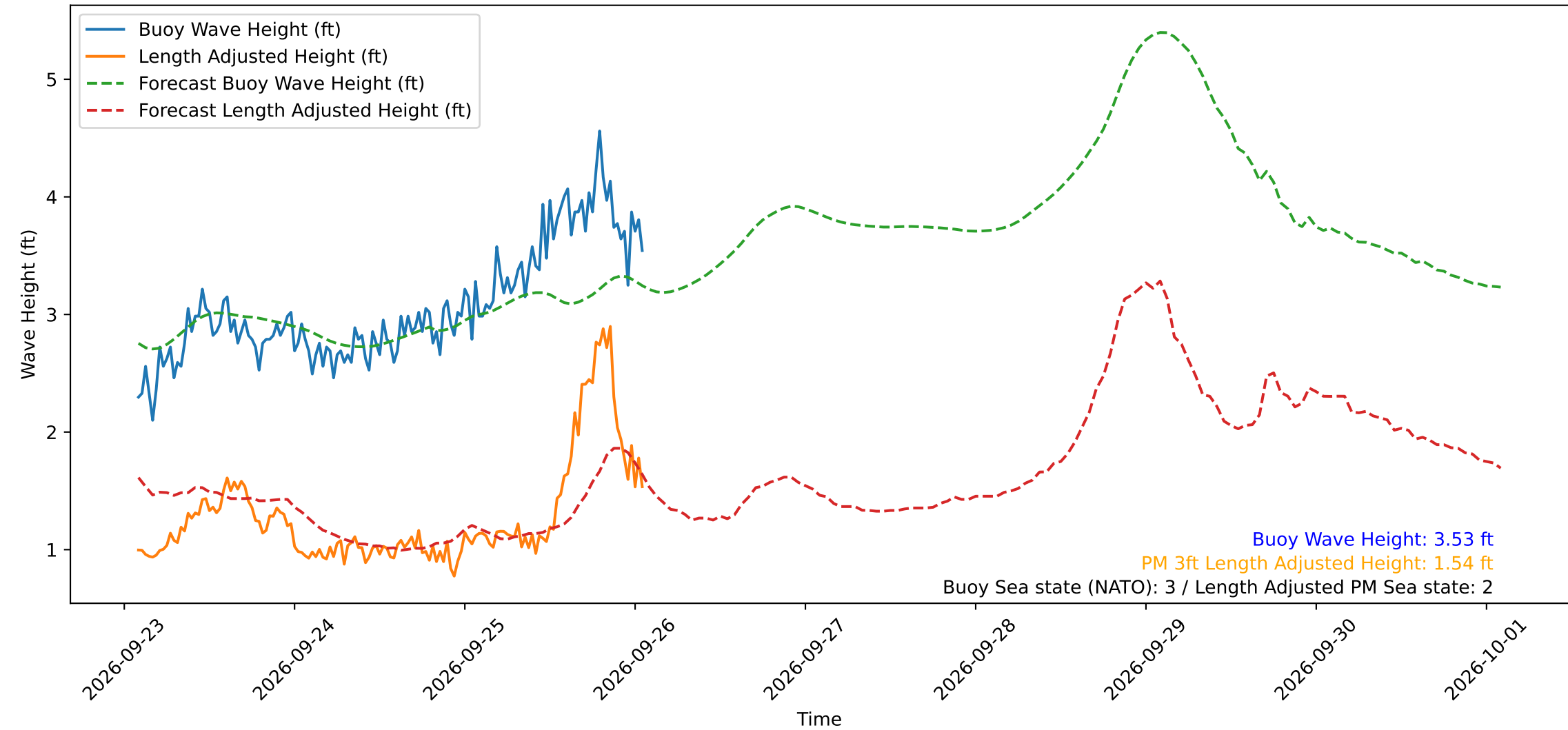
Wave Heights over Time for Green Beach at 2026-09-26 01:51:15
