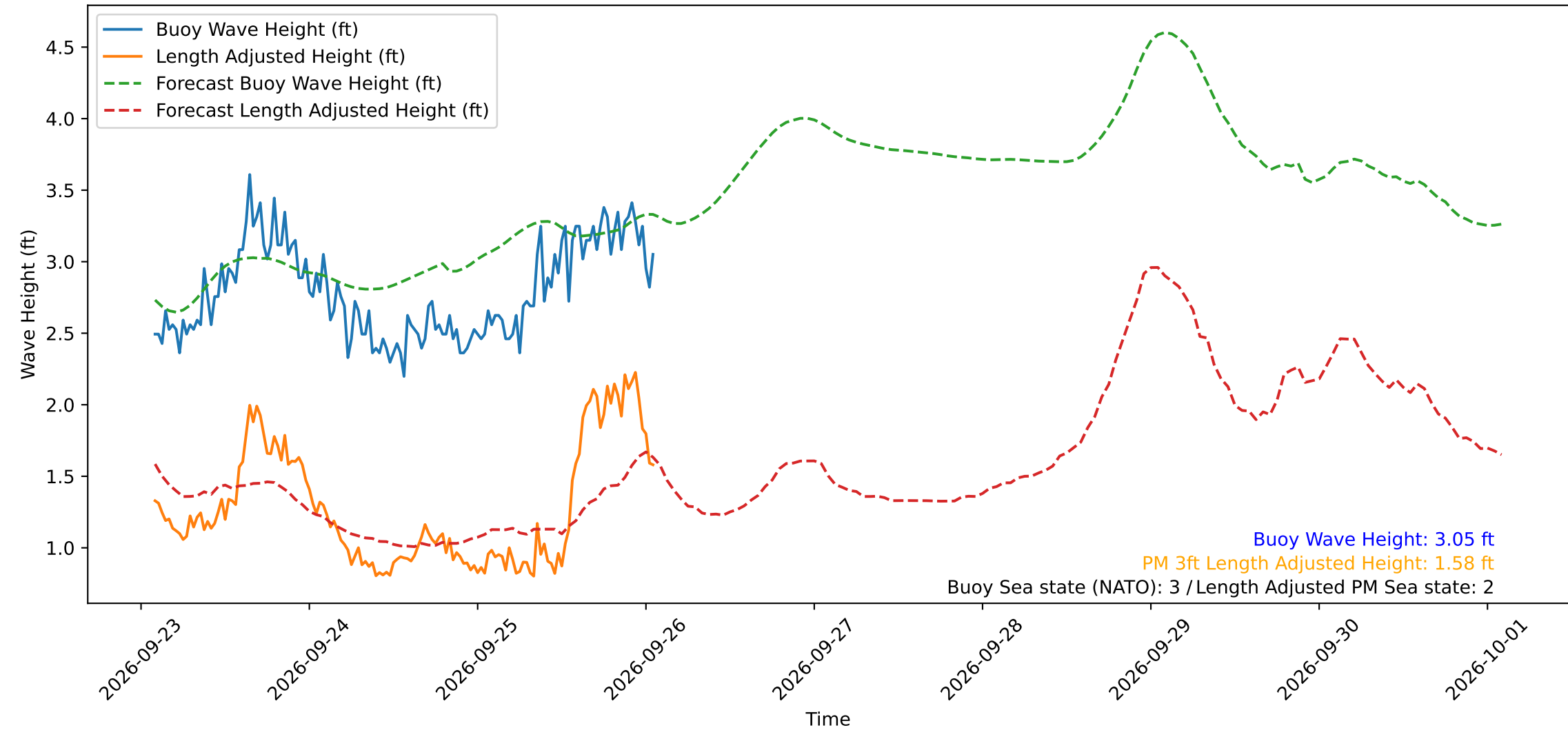
Wave Heights over Time for Oceanside Harbor at 2026-09-26 01:50:30
