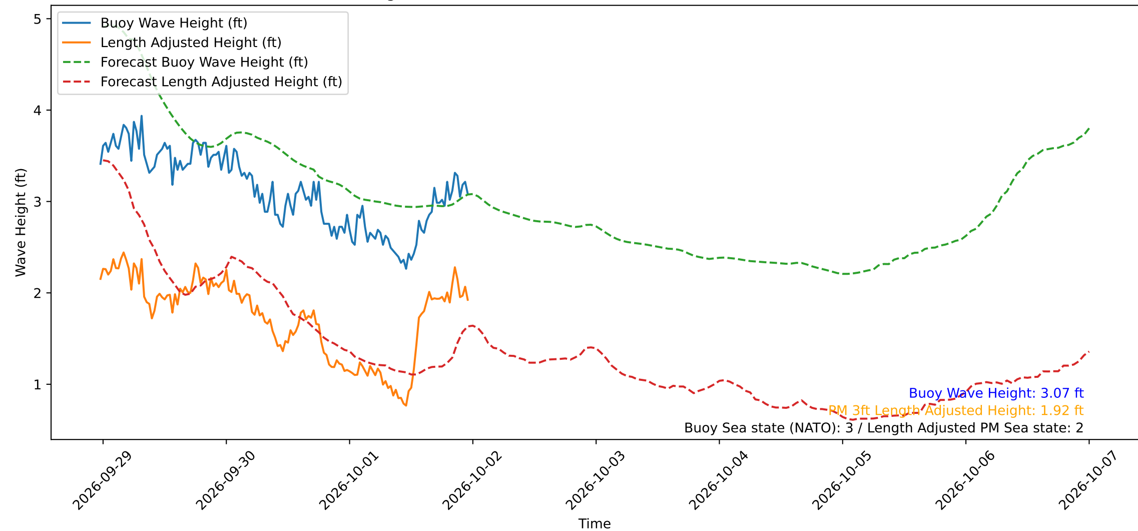
Wave Heights over Time for Oceanside Harbor at 2026-10-01 23:30:30
