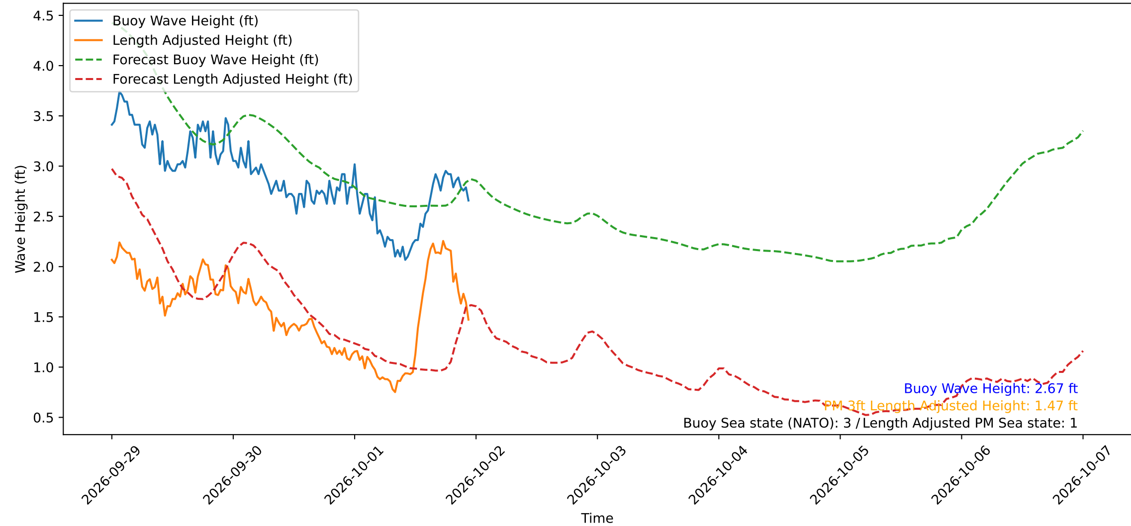
Wave Heights over Time for Red Beach at 2026-10-01 23:30:49
