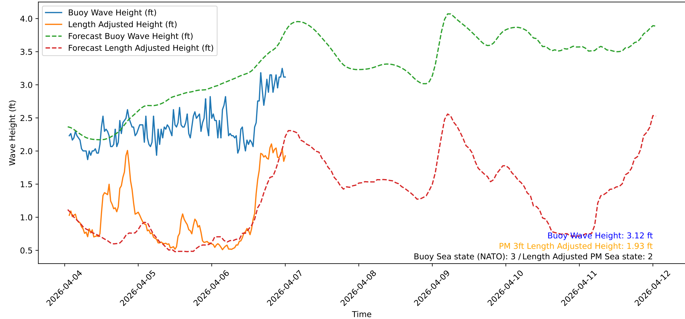
Wave Heights over Time for Red Beach at 2026-04-07 01:20:47
