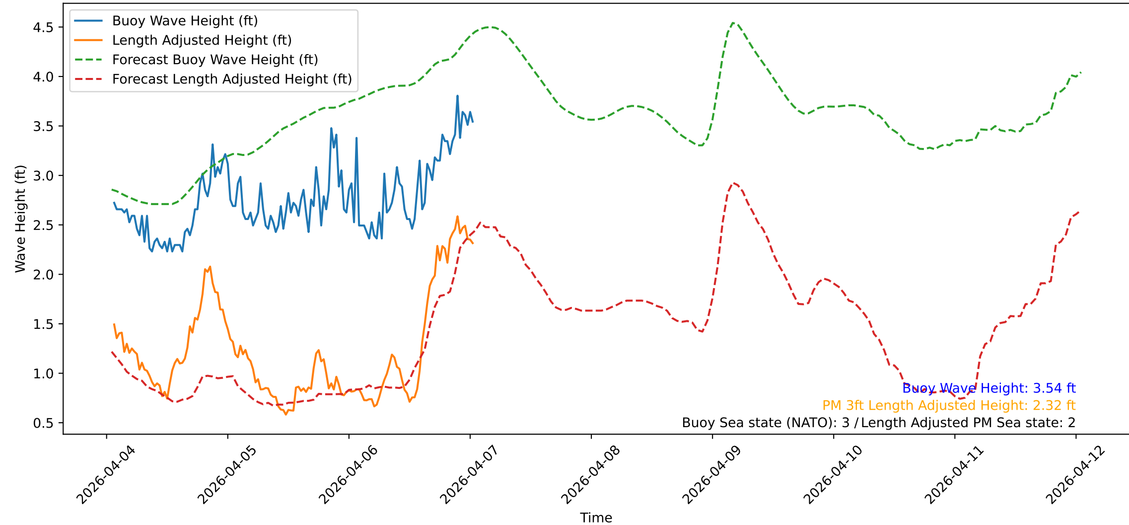
Wave Heights over Time for Green Beach at 2026-04-07 01:21:09
