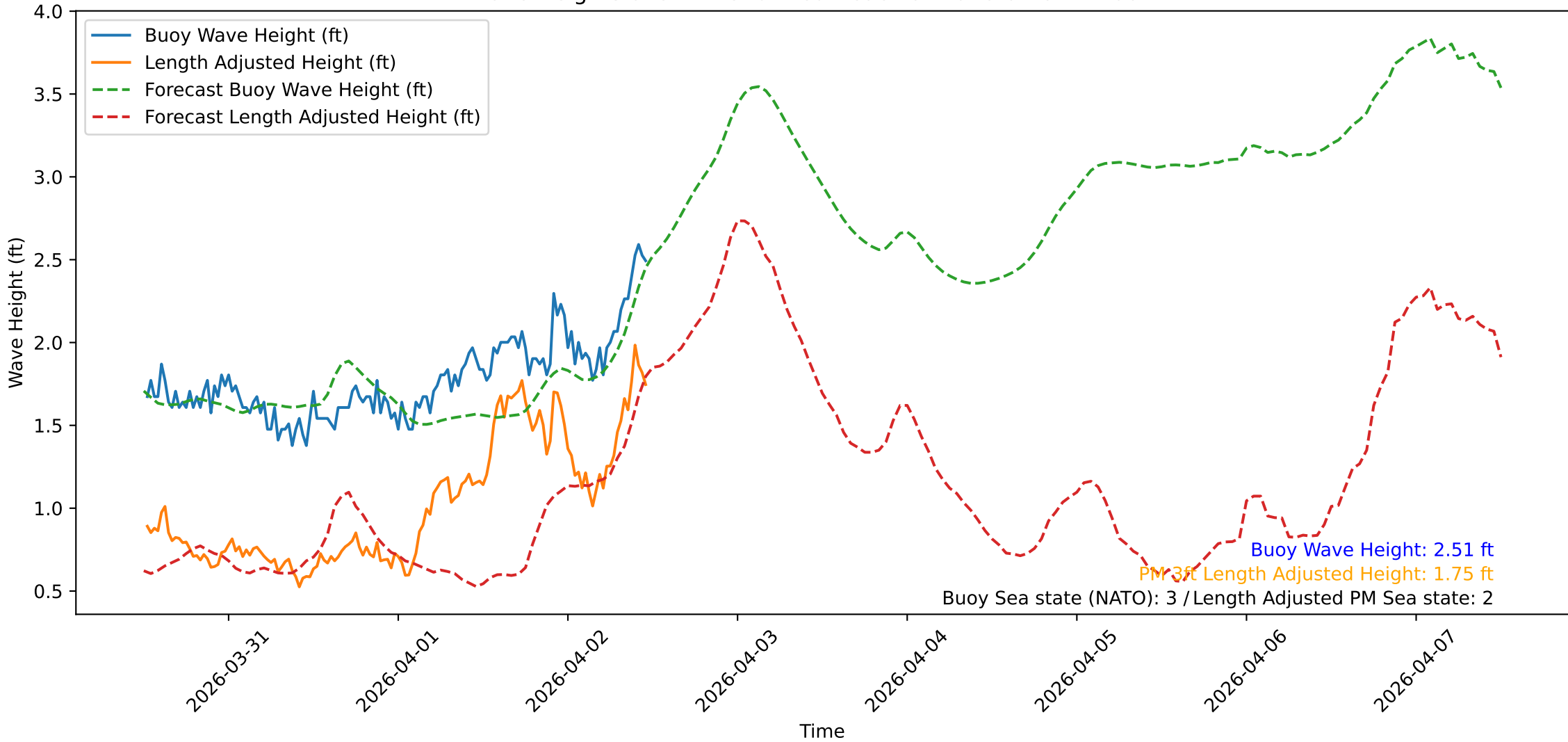
Wave Heights over Time for Red Beach at 2026-04-02 12:00:47
