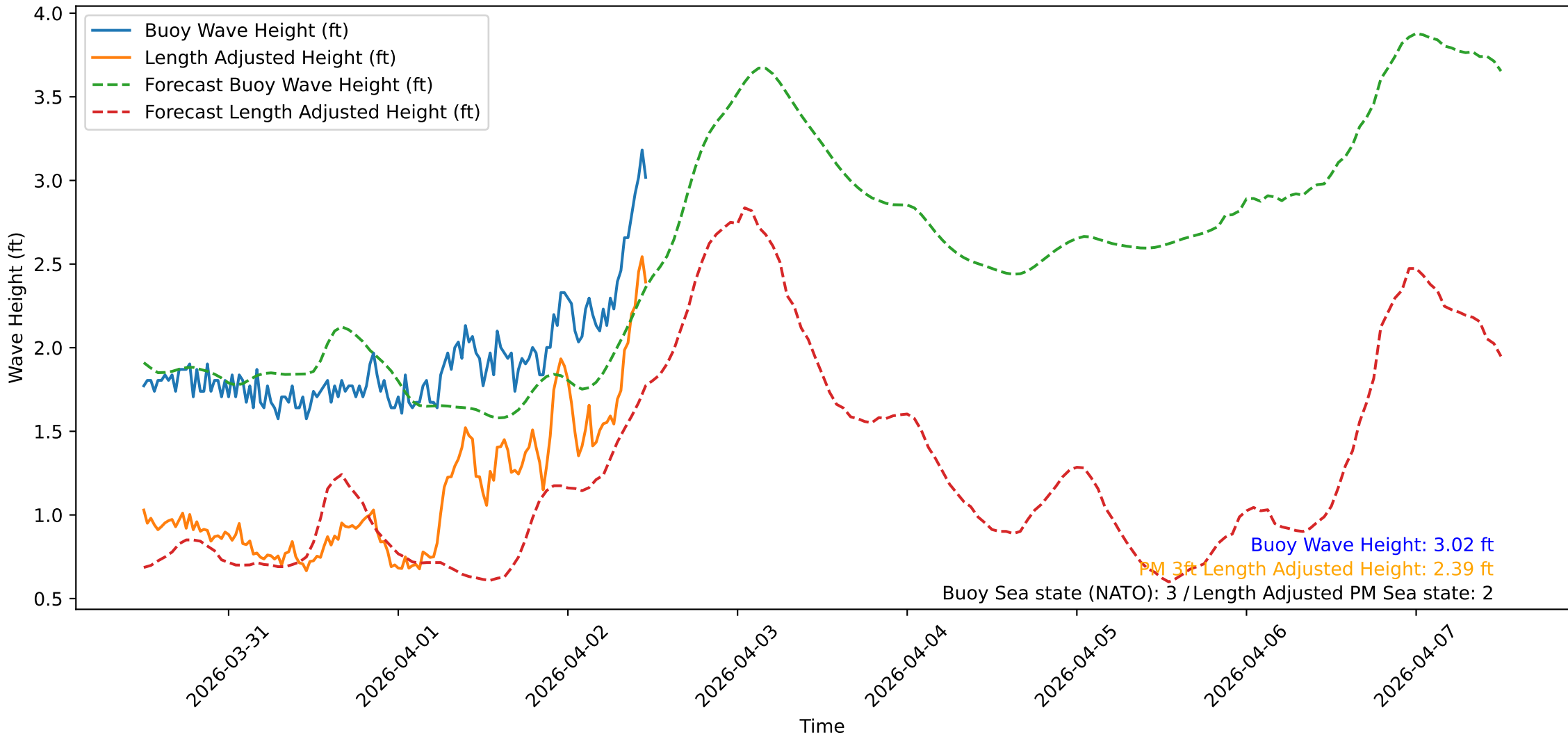
Wave Heights over Time for Oceanside Harbor at 2026-04-02 12:00:31
