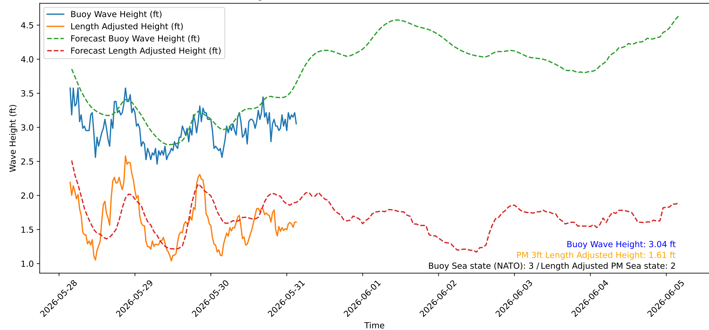
Wave Heights over Time for Green Beach at 2026-05-31 03:41:07
