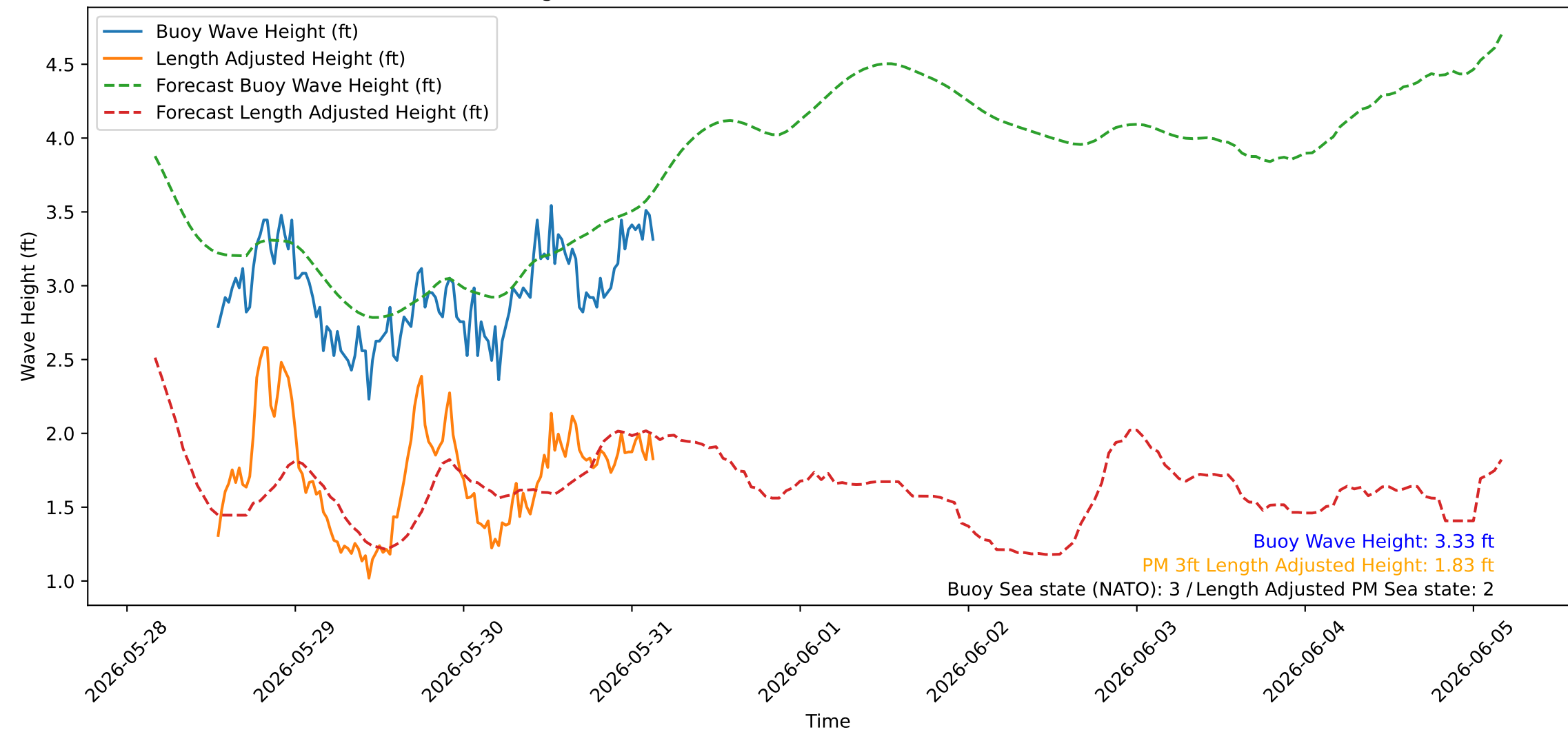
Wave Heights over Time for Oceanside Harbor at 2026-05-31 03:40:25
