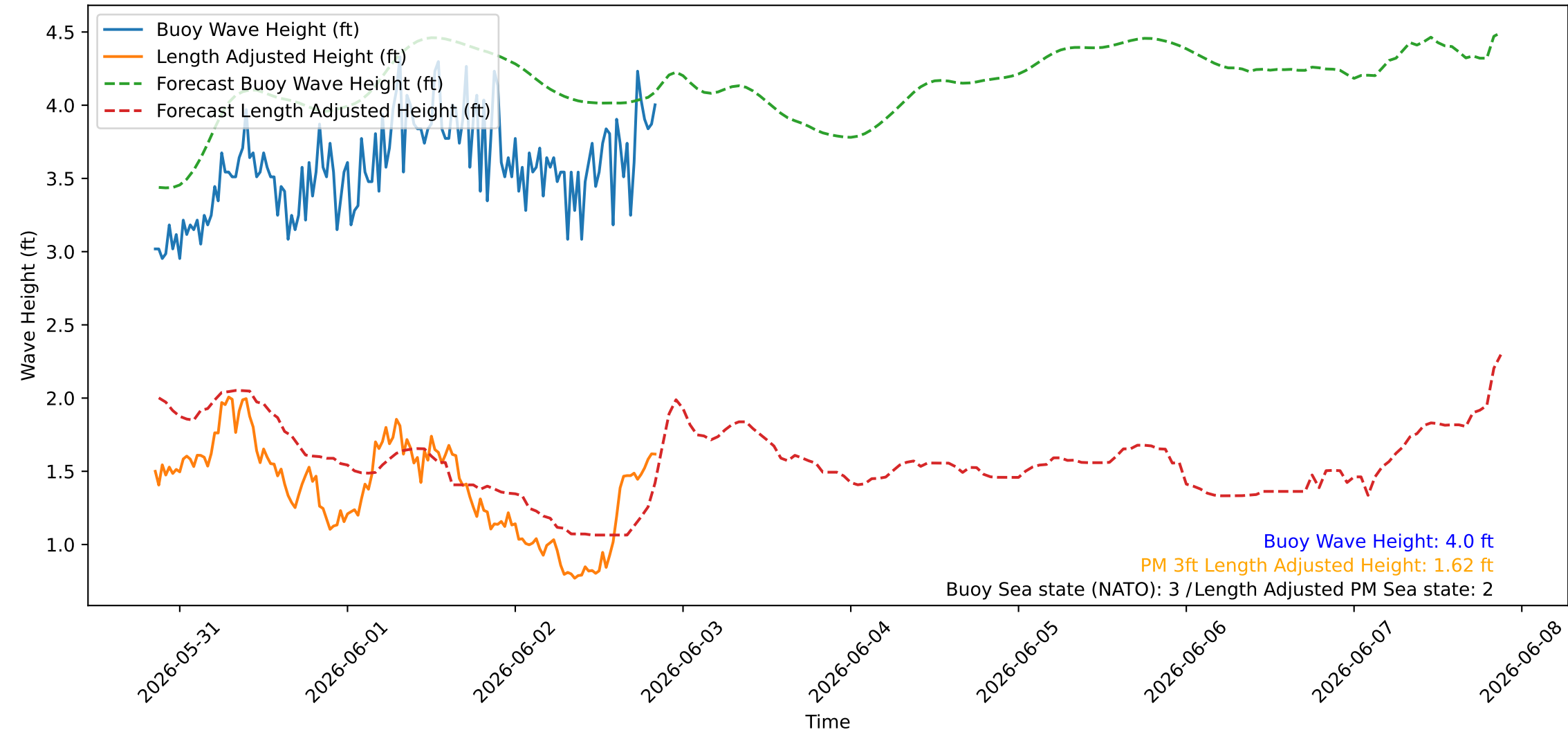
Wave Heights over Time for Green Beach at 2026-06-02 20:41:08
