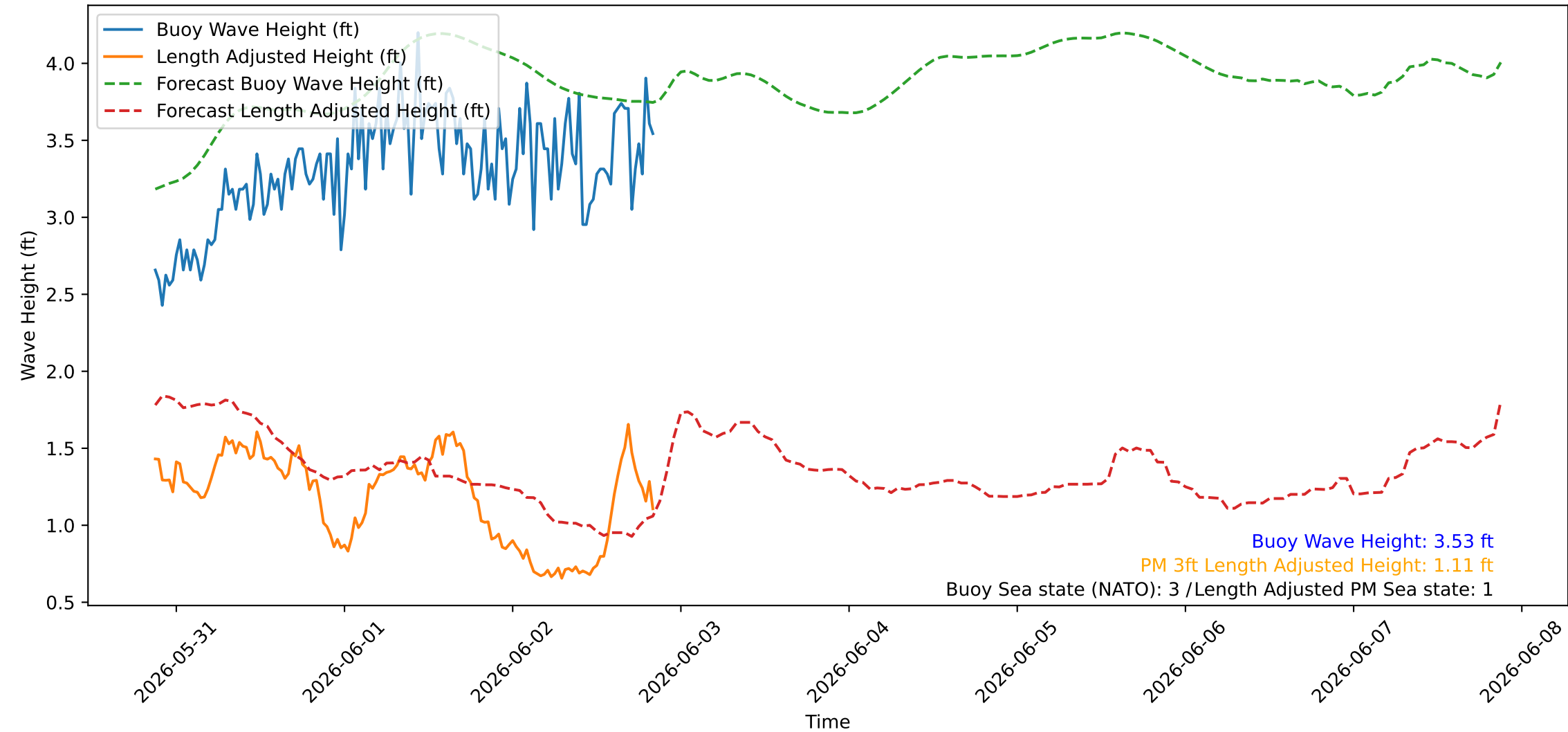
Wave Heights over Time for Red Beach at 2026-06-02 20:40:45
