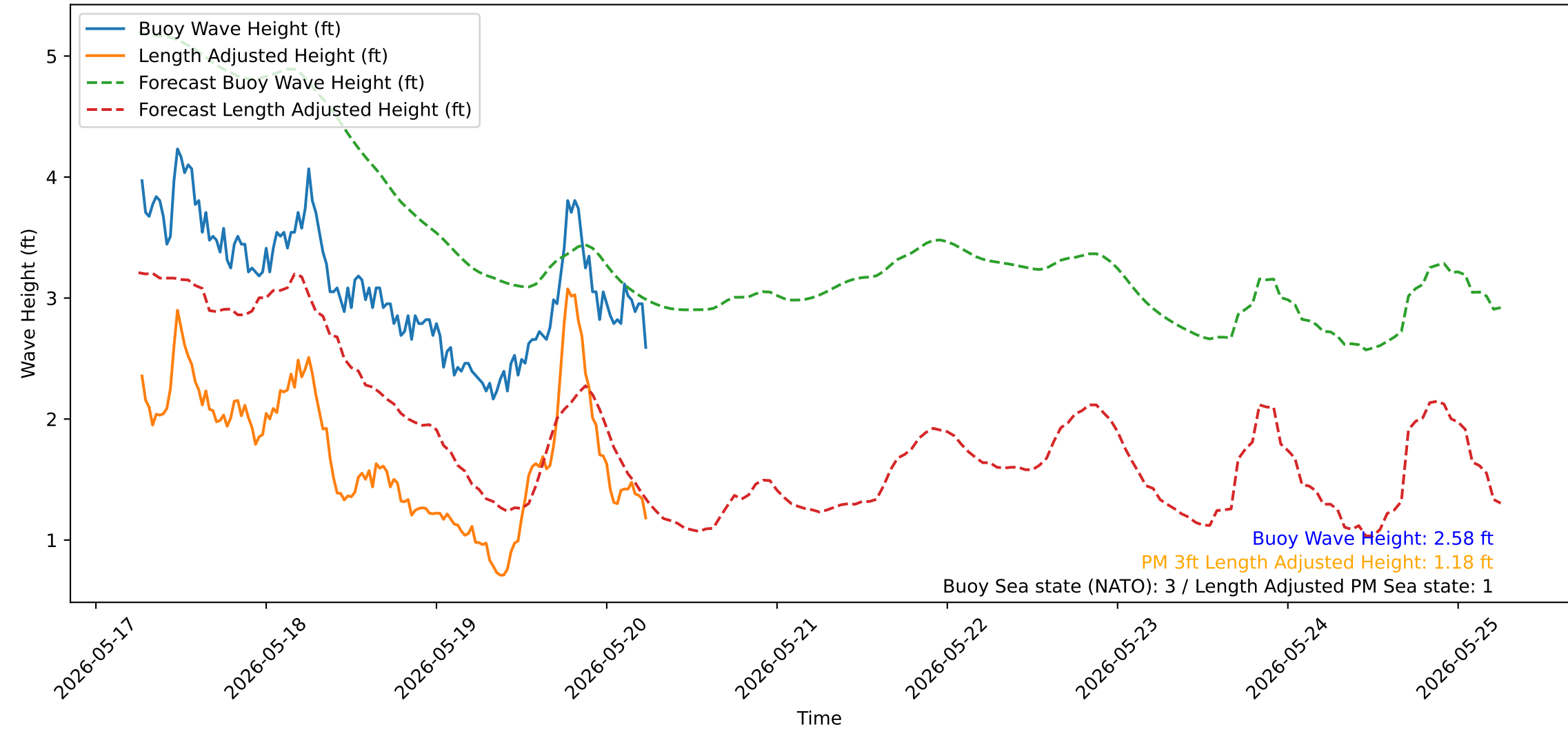
Wave Heights over Time for Green Beach at 2026-05-20 06:21:14
