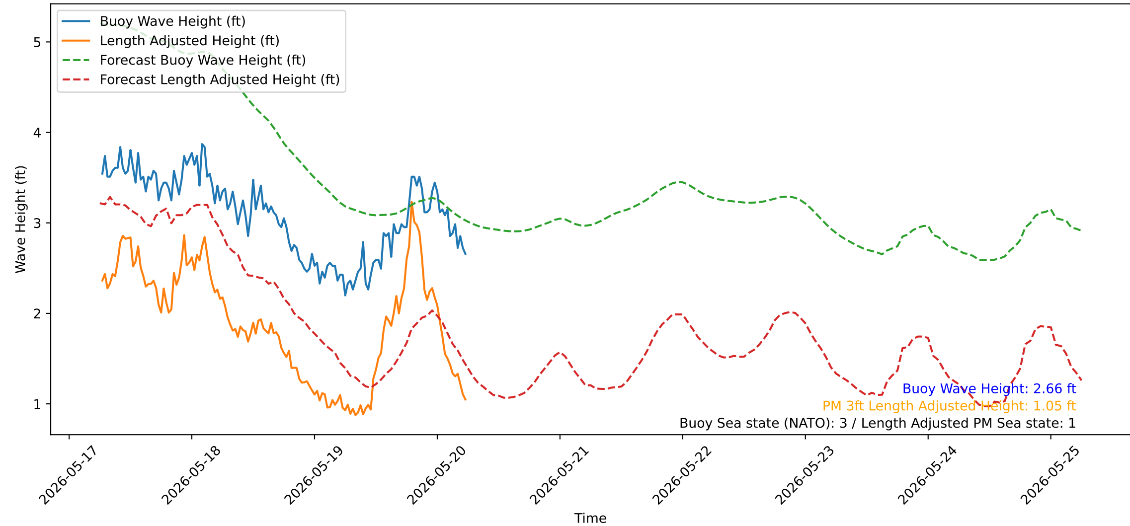
Wave Heights over Time for Oceanside Harbor at 2026-05-20 06:20:31
