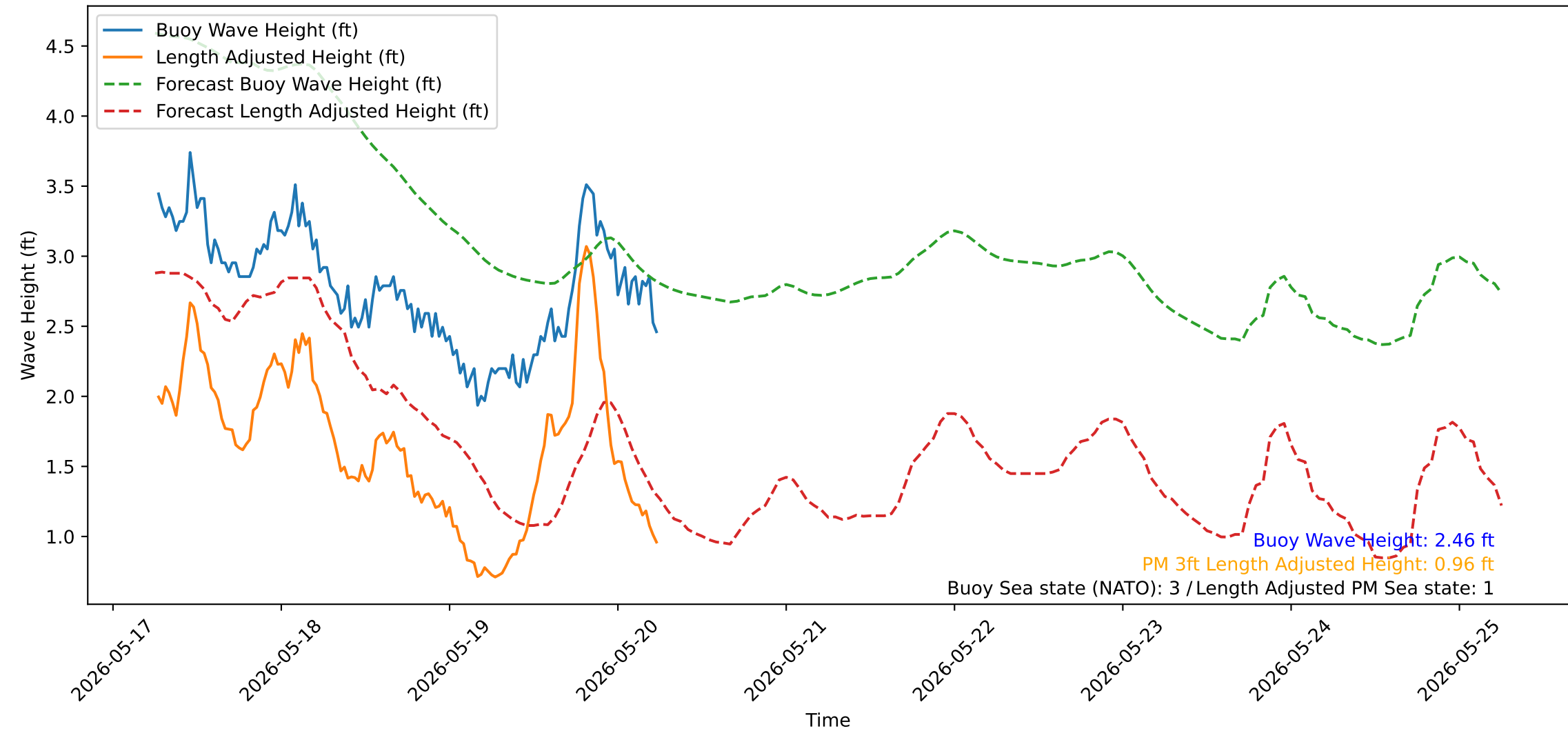
Wave Heights over Time for Red Beach at 2026-05-20 06:20:52
