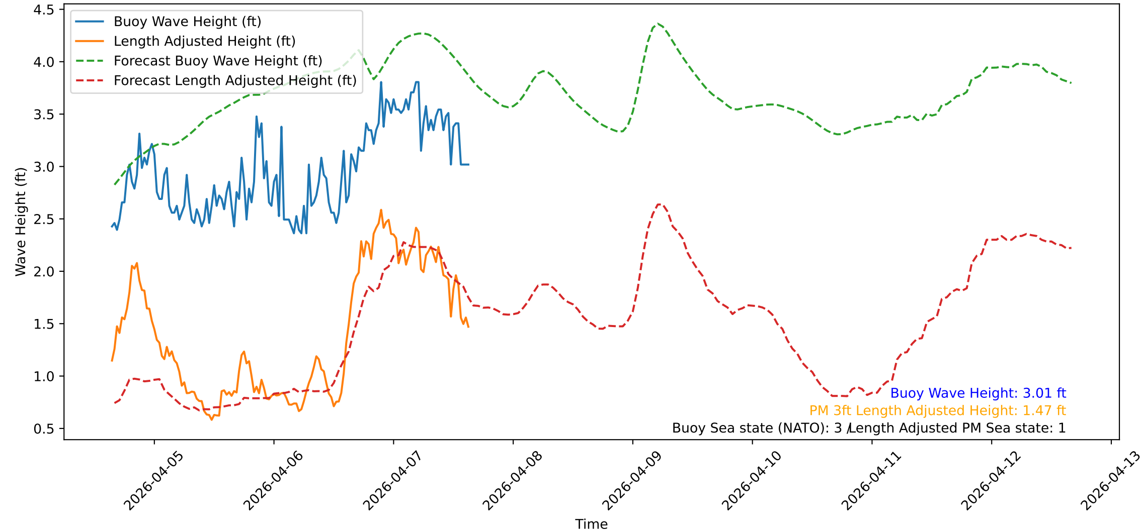
Wave Heights over Time for Green Beach at 2026-04-07 15:41:12
