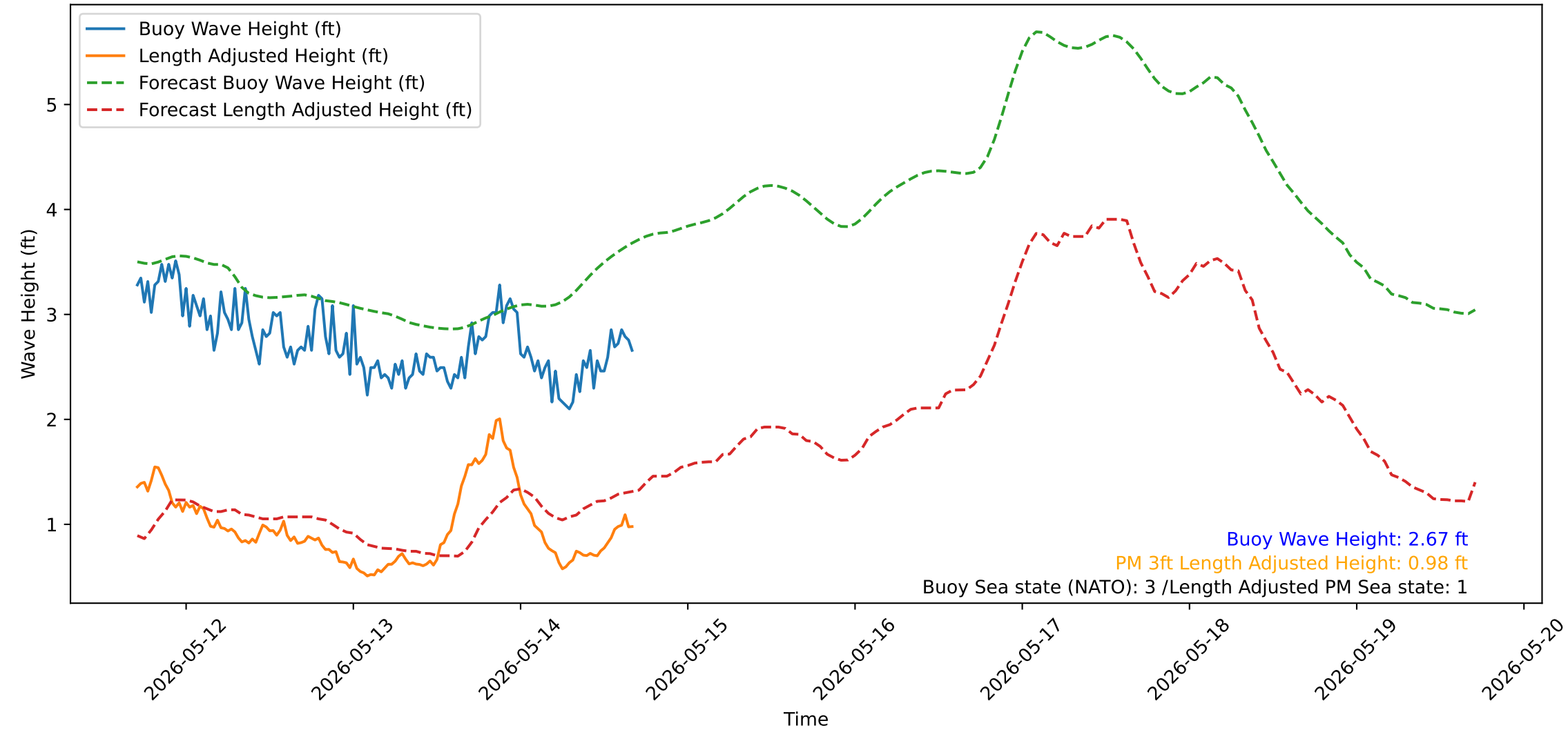
Wave Heights over Time for Green Beach at 2026-05-14 17:01:14
