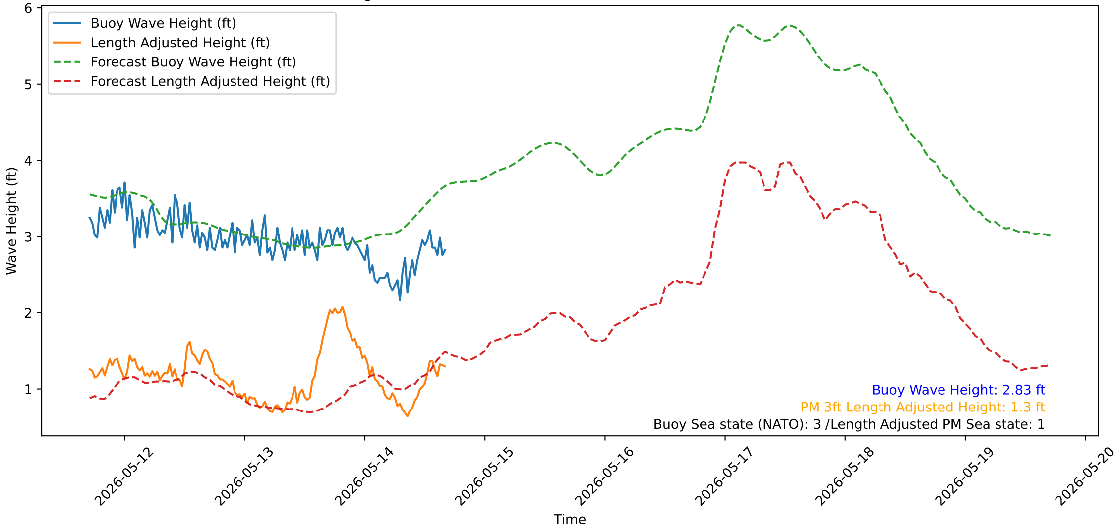
Wave Heights over Time for Oceanside Harbor at 2026-05-14 17:00:32
