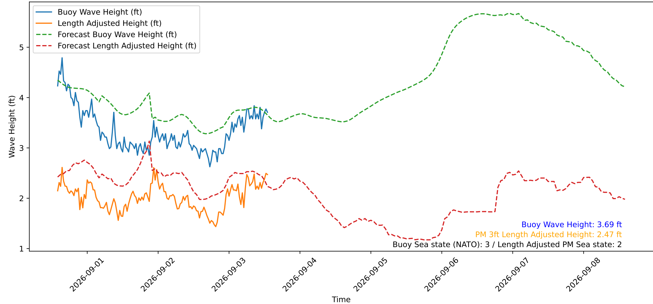
Wave Heights over Time for Oceanside Harbor at 2026-09-03 13:50:30
