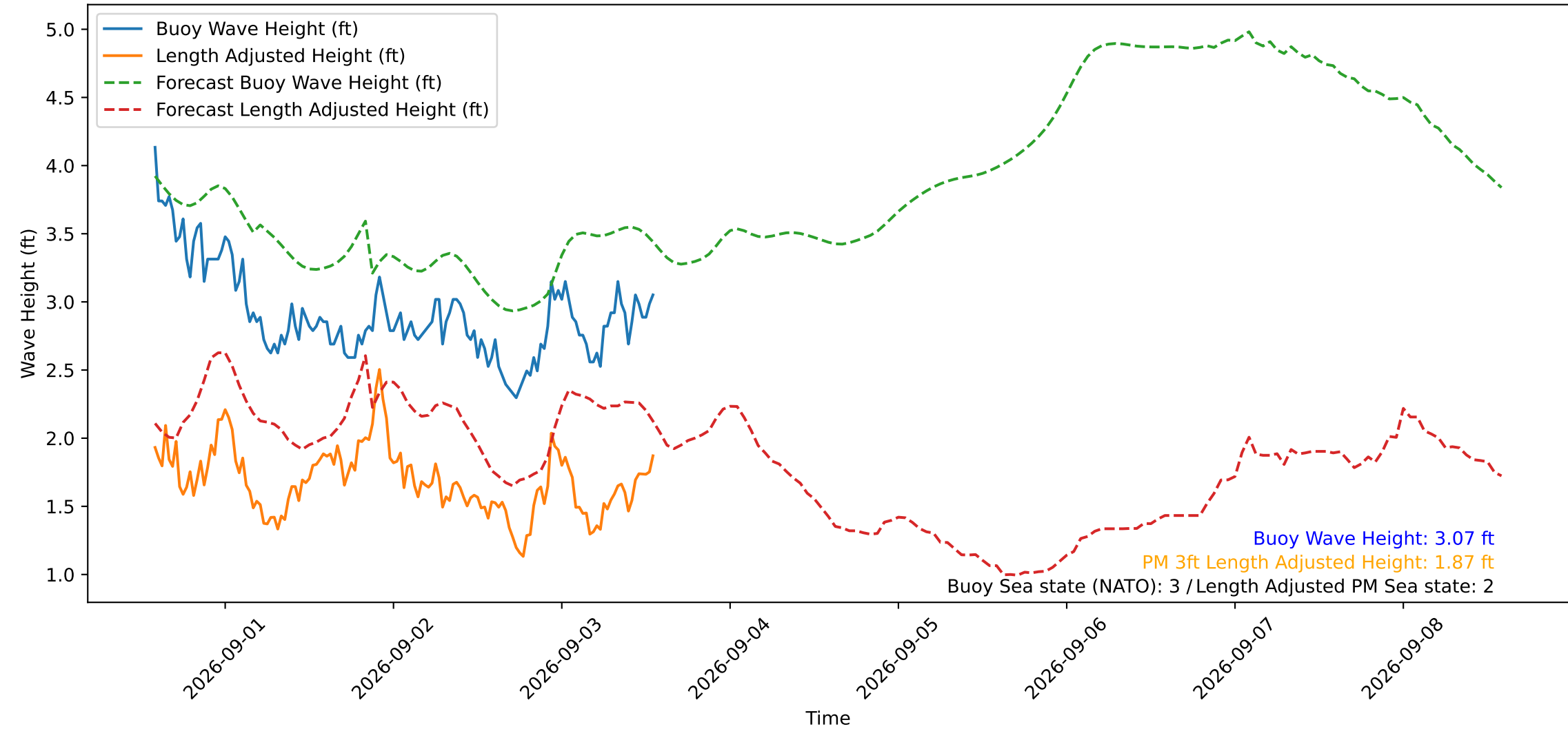
Wave Heights over Time for Red Beach at 2026-09-03 13:50:51
