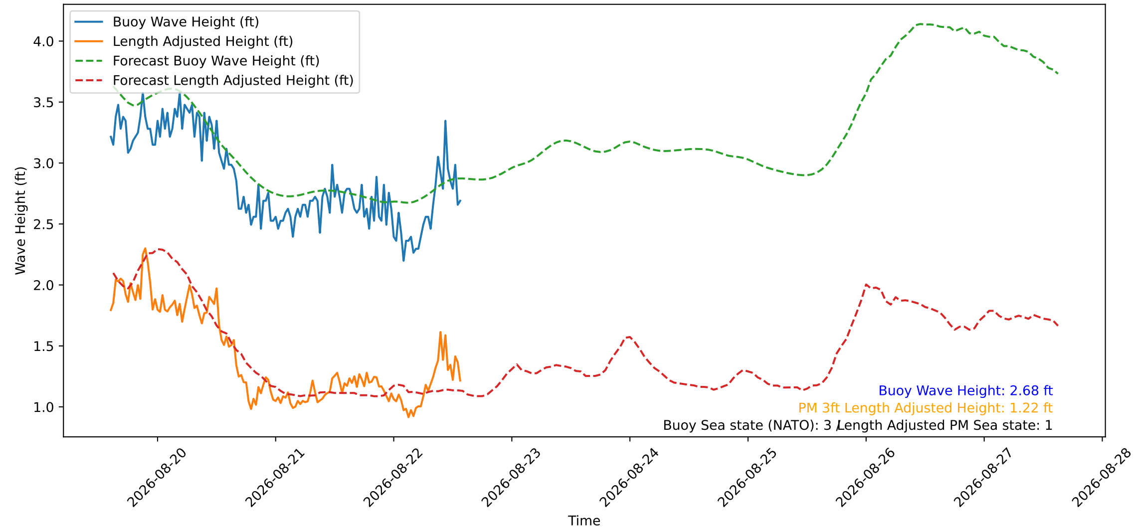
Wave Heights over Time for Oceanside Harbor at 2026-08-22 14:30:30
