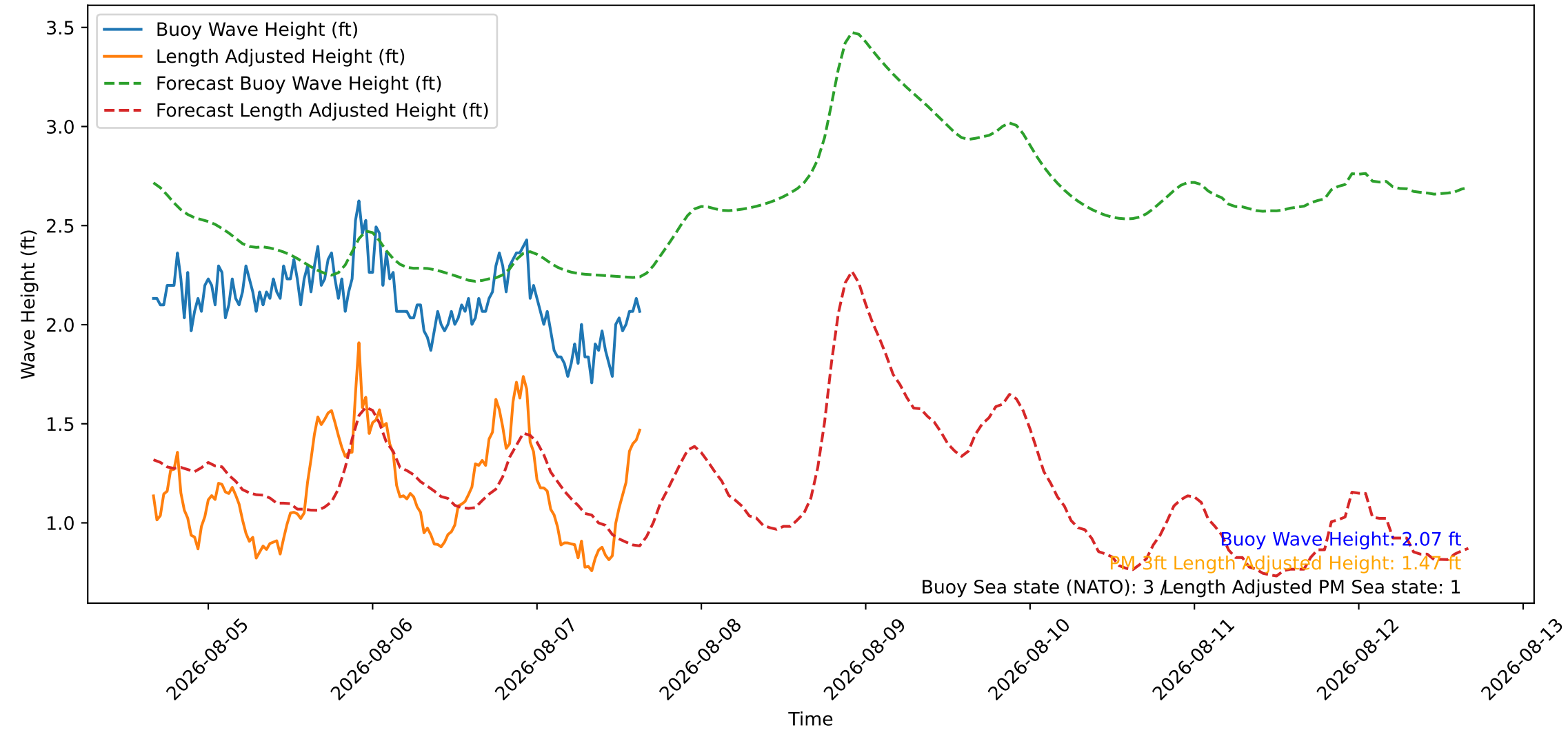
Wave Heights over Time for Green Beach at 2026-08-07 16:01:08
