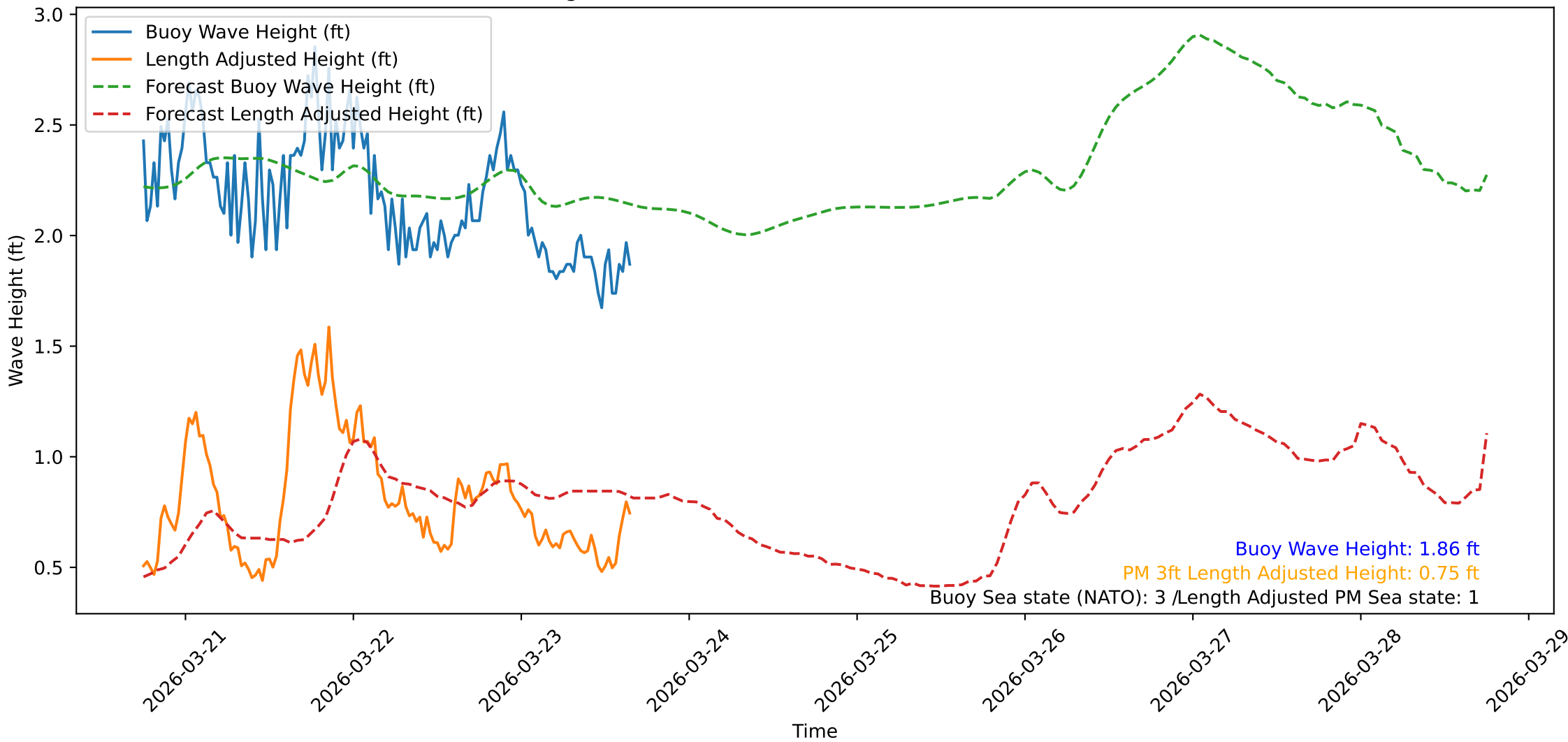
Wave Heights over Time for Red Beach at 2026-03-23 17:50:48
