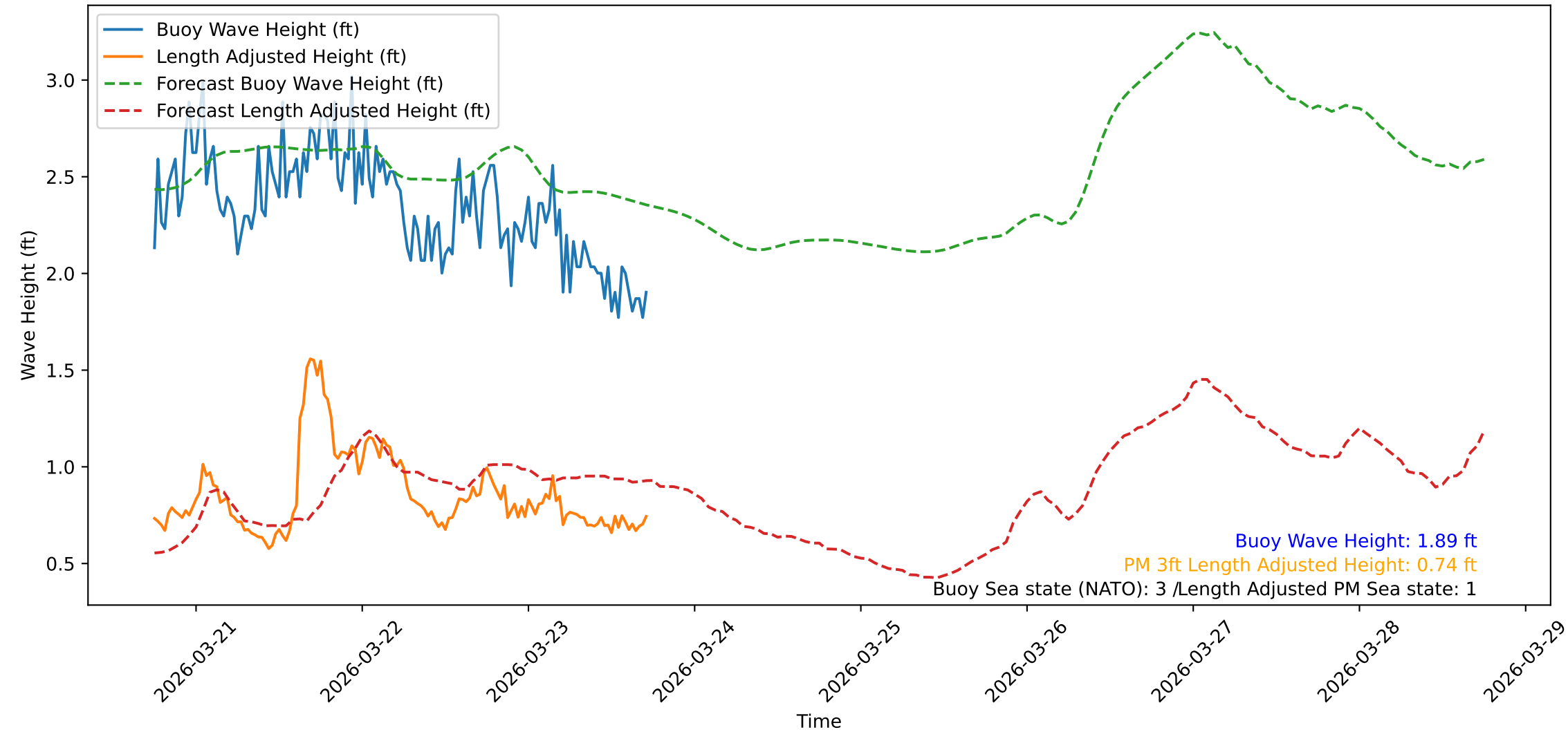
Wave Heights over Time for Oceanside Harbor at 2026-03-23 17:50:31
