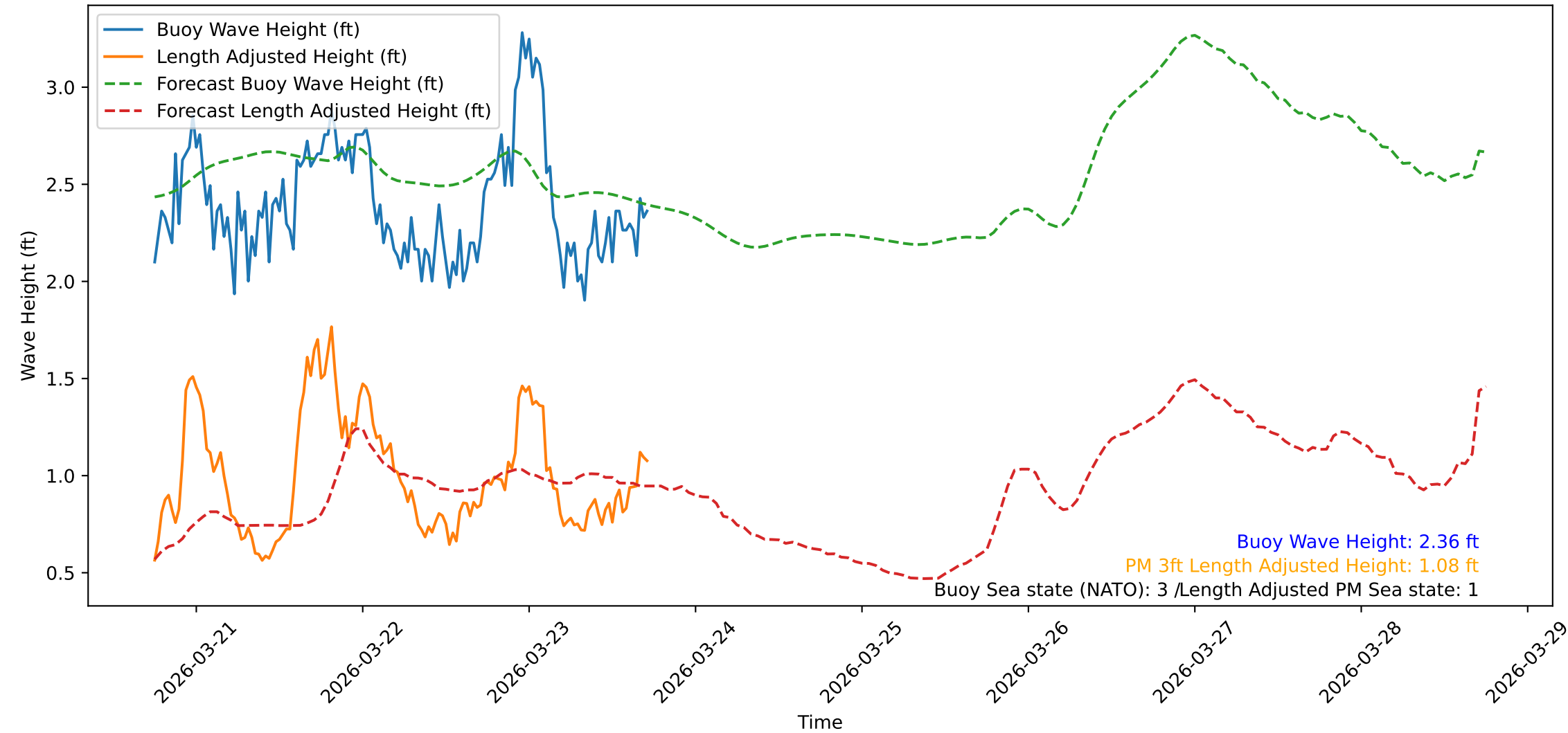
Wave Heights over Time for Green Beach at 2026-03-23 17:51:11
