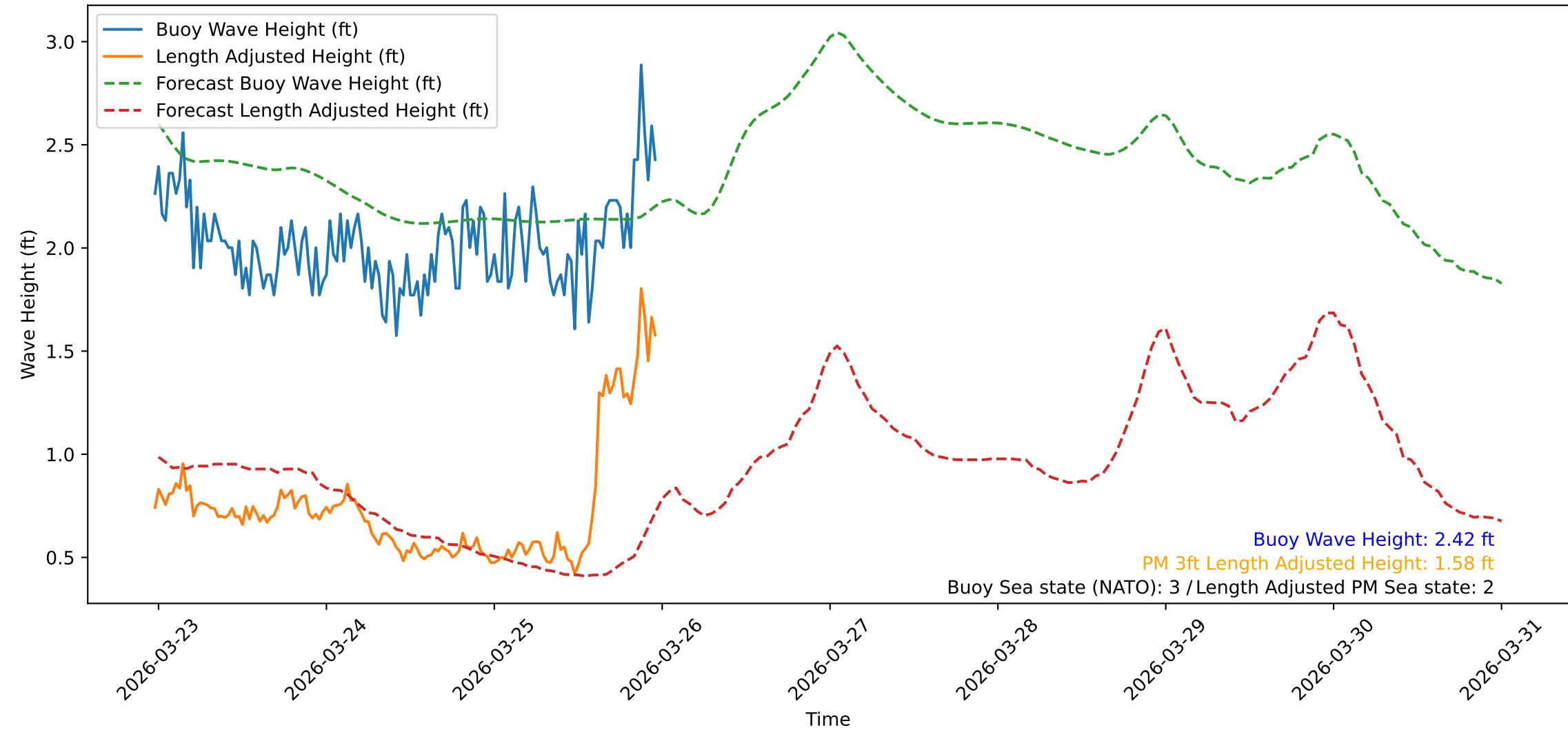
Wave Heights over Time for Oceanside Harbor at 2026-03-25 23:40:32
