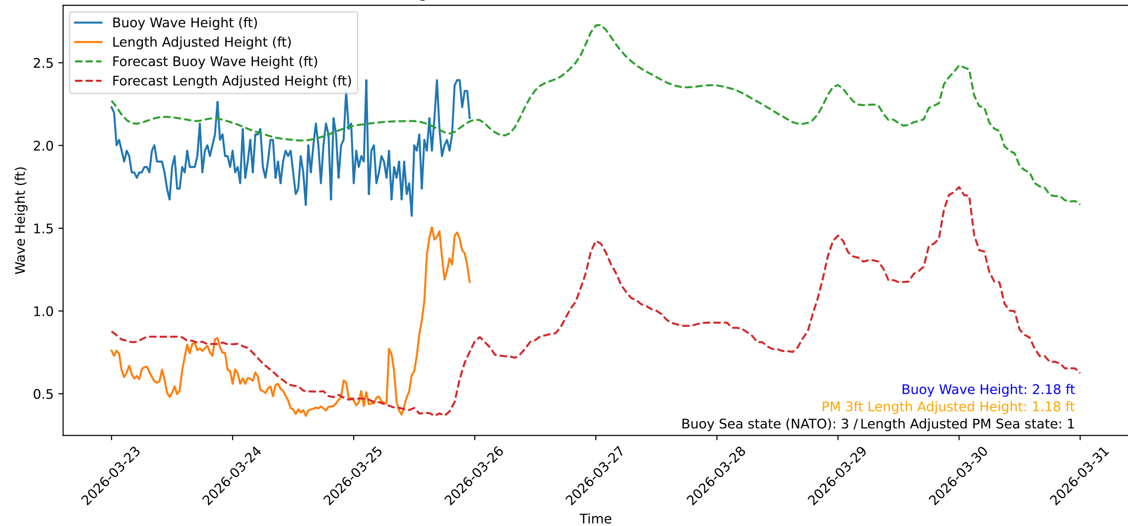
Wave Heights over Time for Red Beach at 2026-03-25 23:40:48
