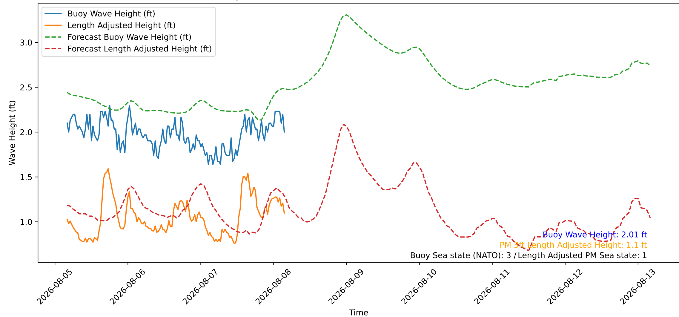
Wave Heights over Time for Oceanside Harbor at 2026-08-08 04:10:26
