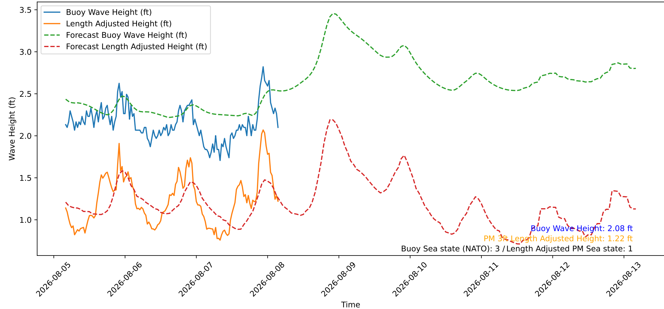
Wave Heights over Time for Green Beach at 2026-08-08 04:11:08
