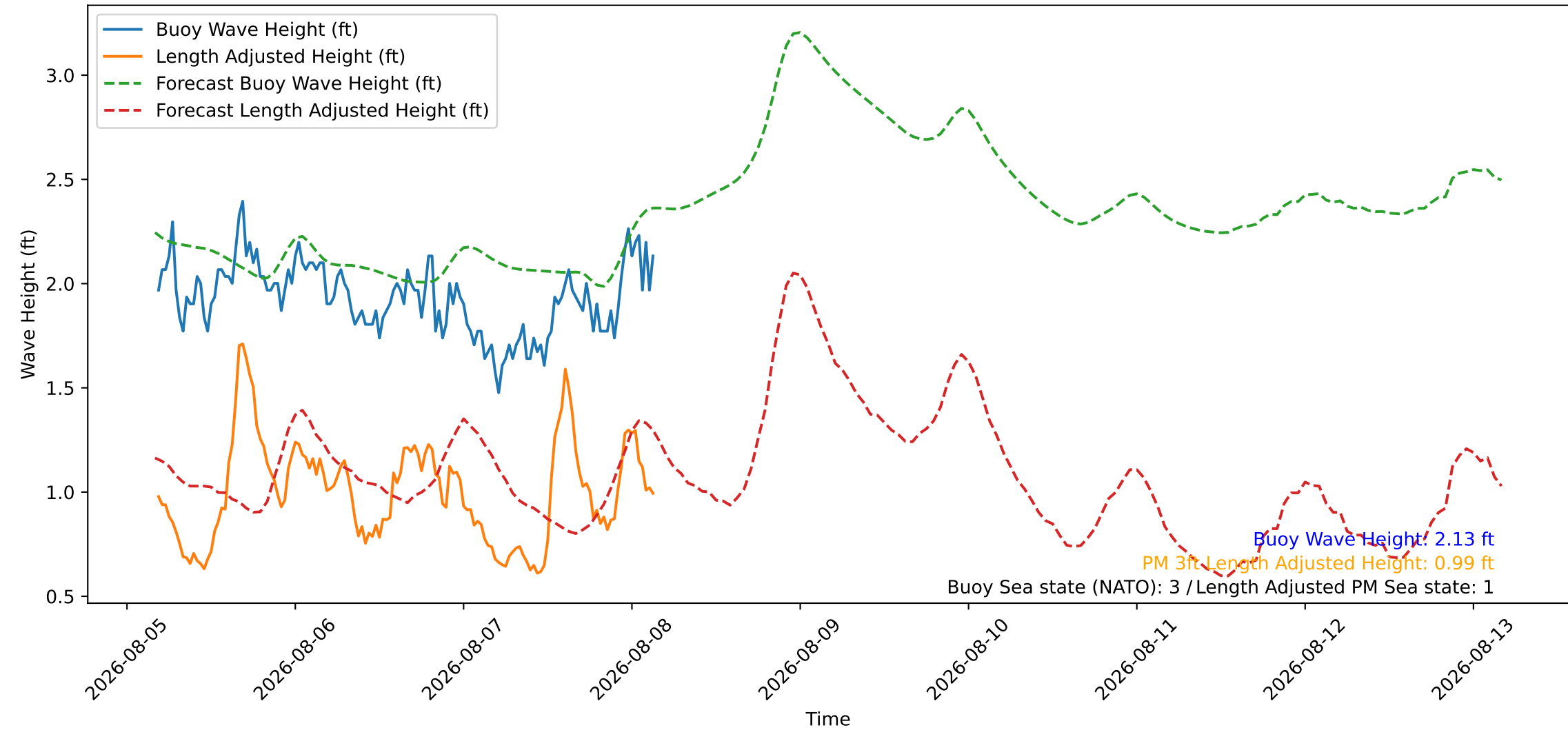
Wave Heights over Time for Red Beach at 2026-08-08 04:10:46
