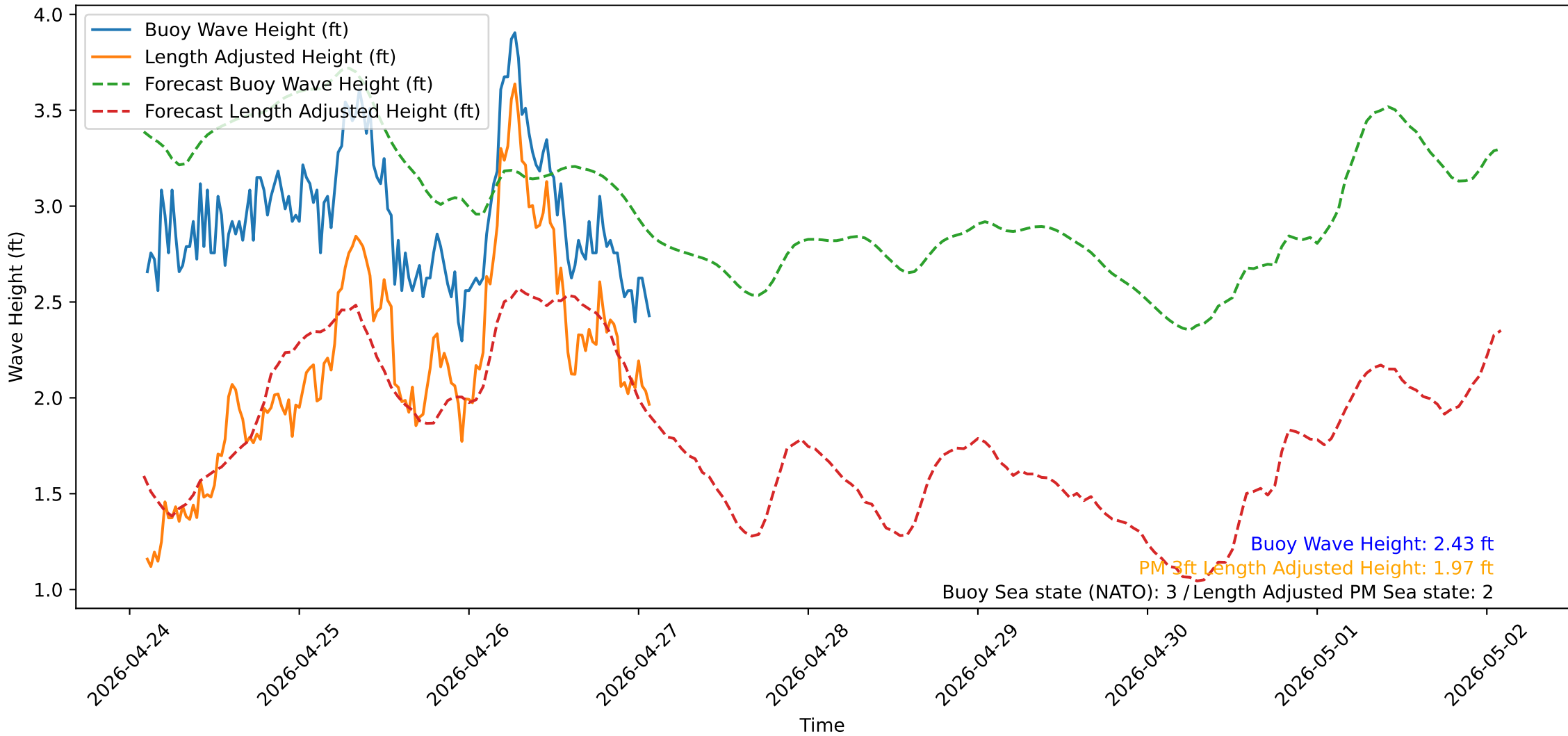
Wave Heights over Time for Oceanside Harbor at 2026-04-27 02:20:31
