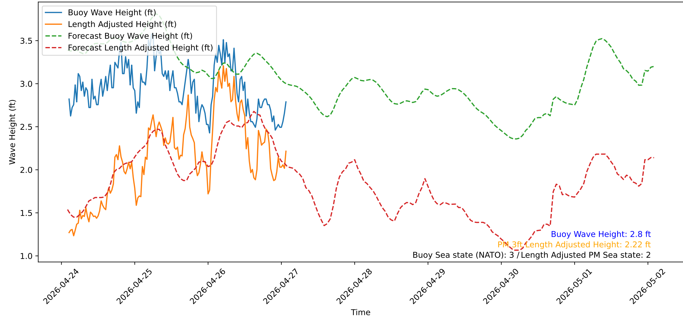
Wave Heights over Time for Green Beach at 2026-04-27 02:21:15
