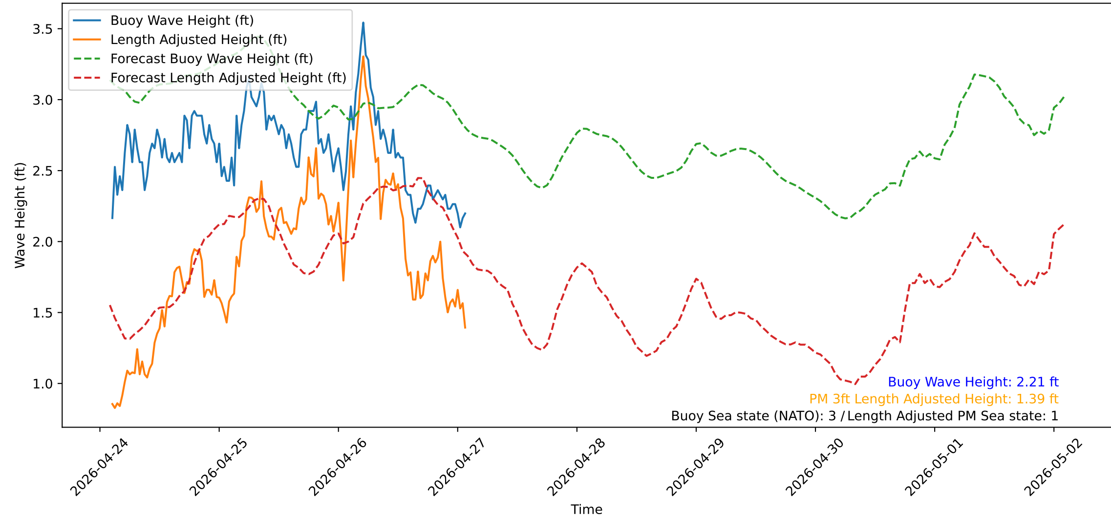
Wave Heights over Time for Red Beach at 2026-04-27 02:20:52
