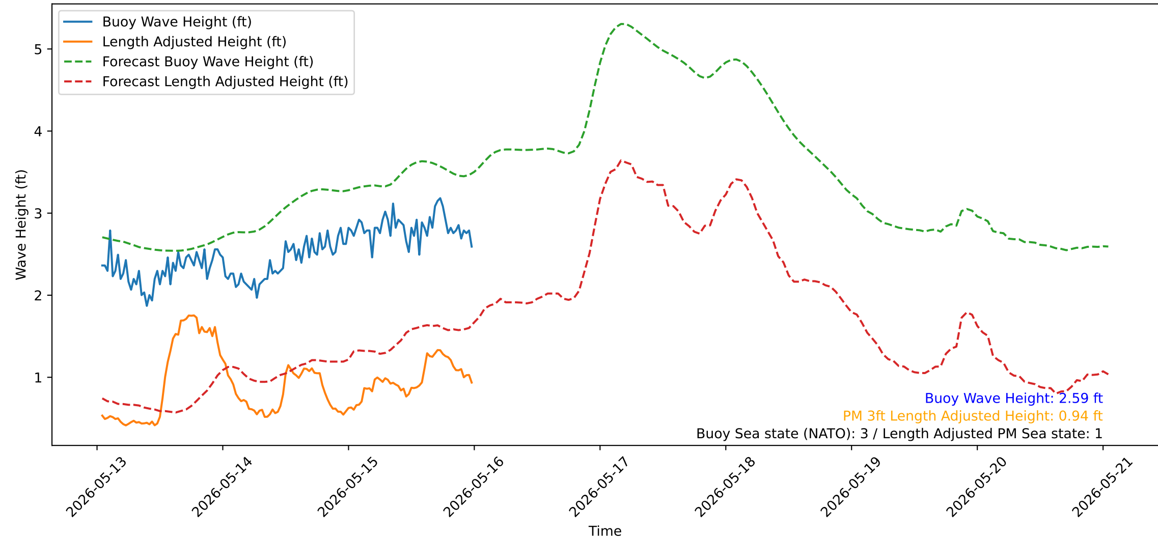
Wave Heights over Time for Red Beach at 2026-05-16 00:30:51
