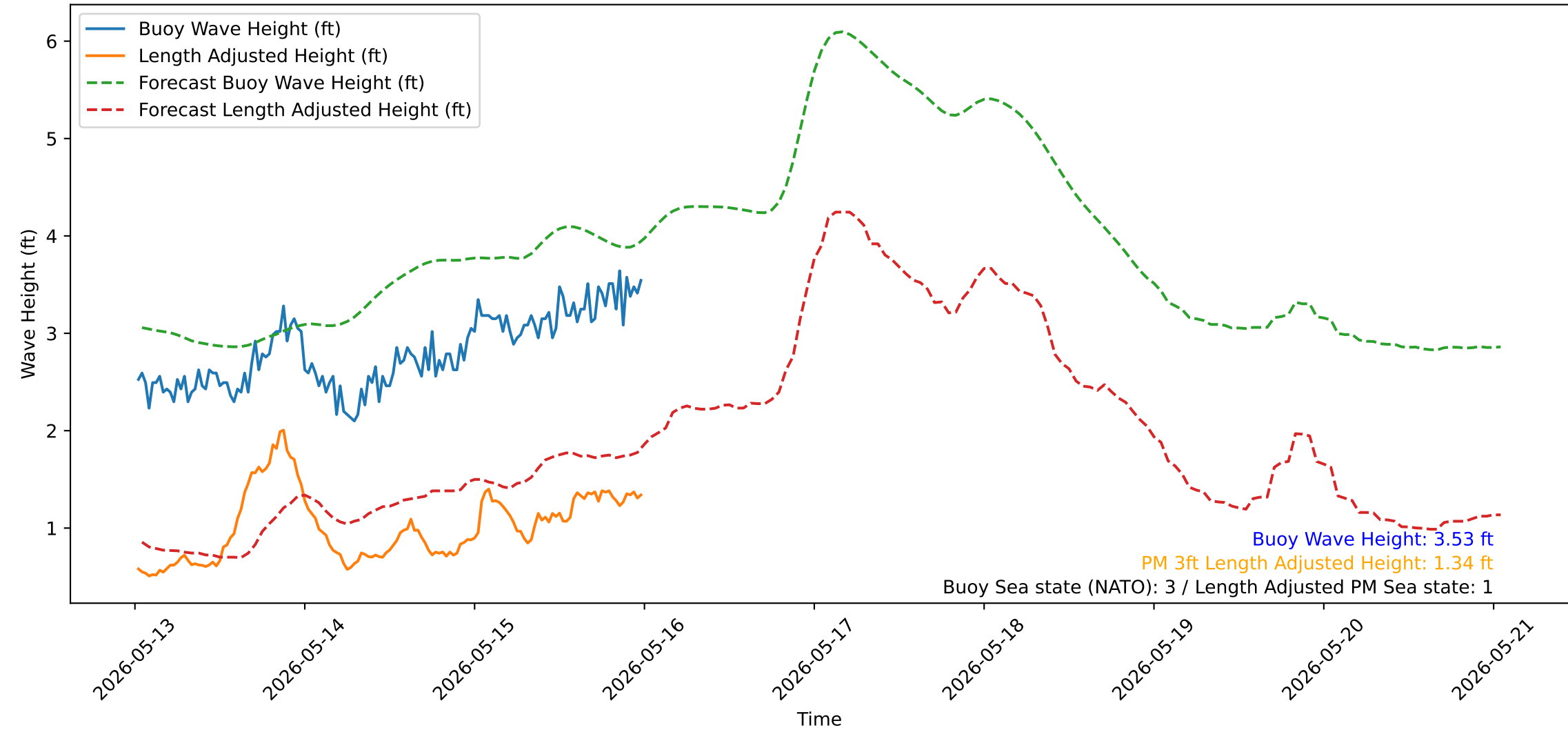
Wave Heights over Time for Green Beach at 2026-05-16 00:31:14
