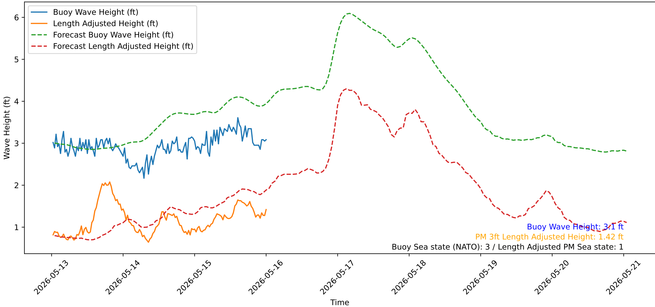
Wave Heights over Time for Oceanside Harbor at 2026-05-16 00:30:32
