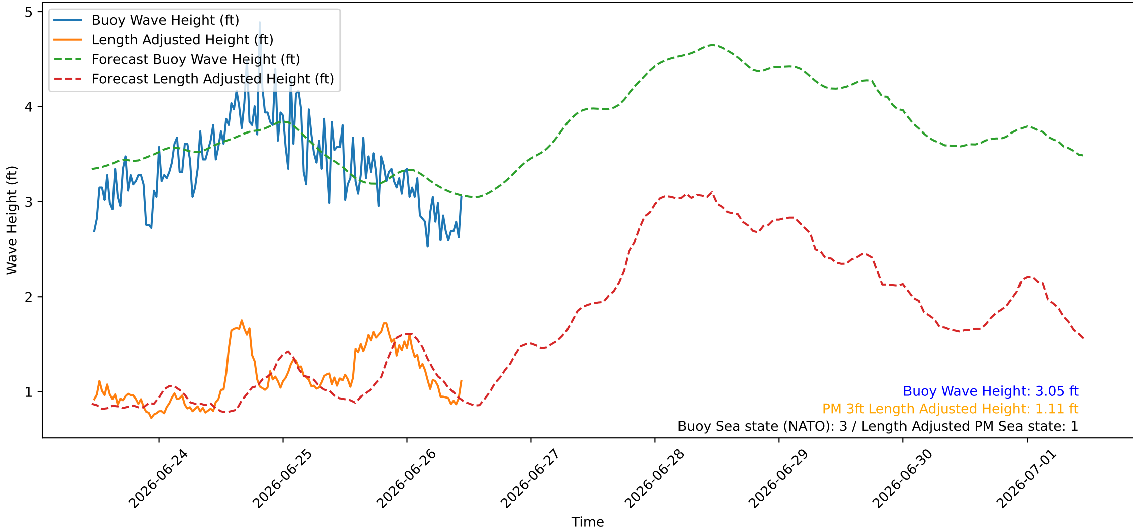
Wave Heights over Time for Oceanside Harbor at 2026-06-26 11:20:26
