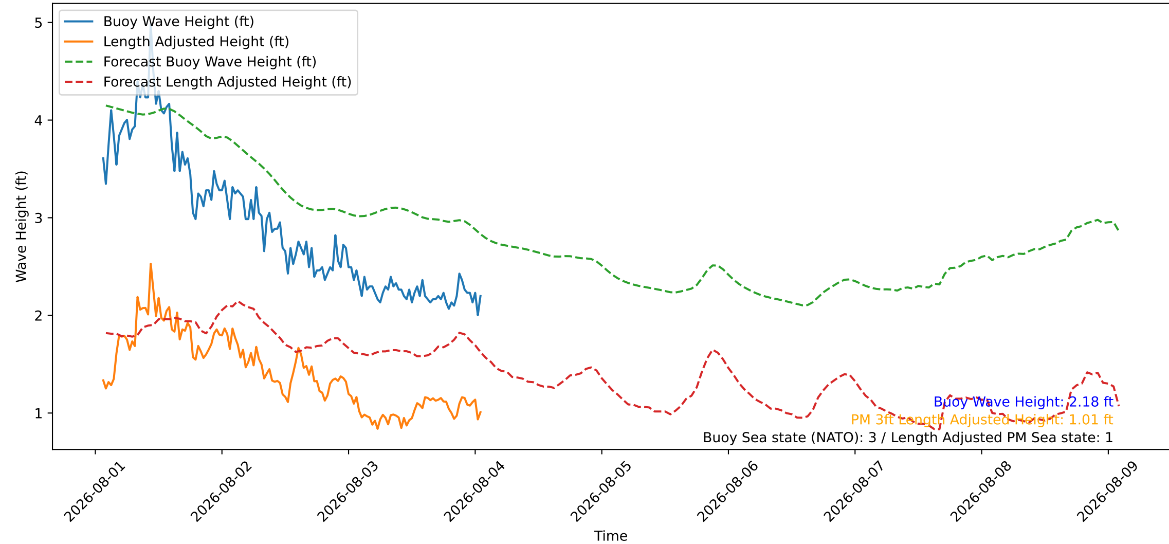
Wave Heights over Time for Green Beach at 2026-08-04 01:41:08
