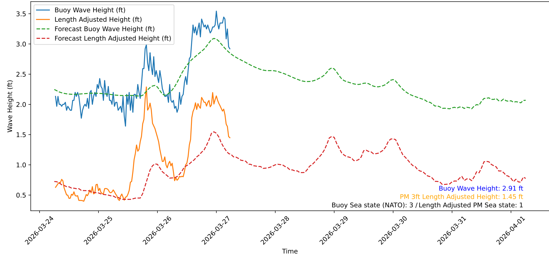
Wave Heights over Time for Green Beach at 2026-03-27 06:21:10
