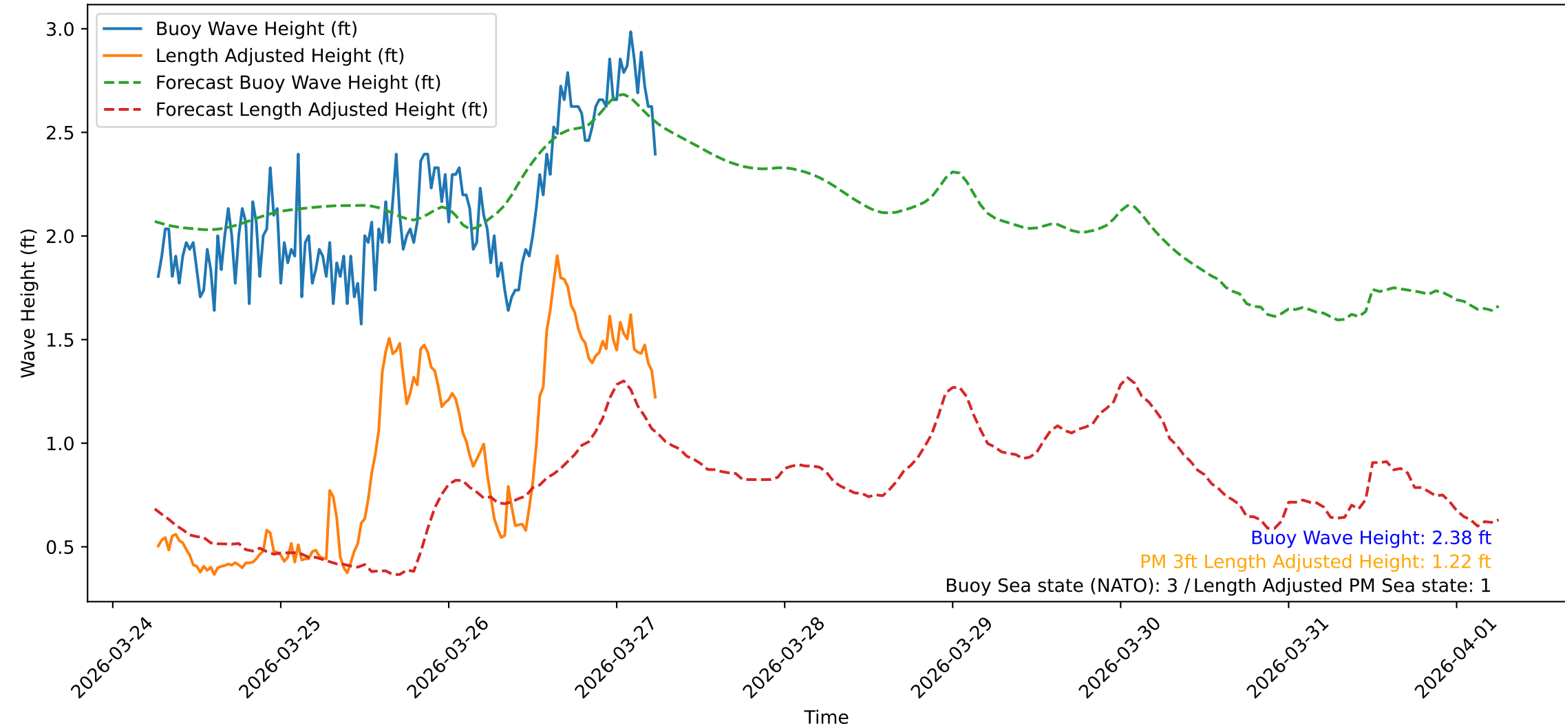
Wave Heights over Time for Red Beach at 2026-03-27 06:20:47
