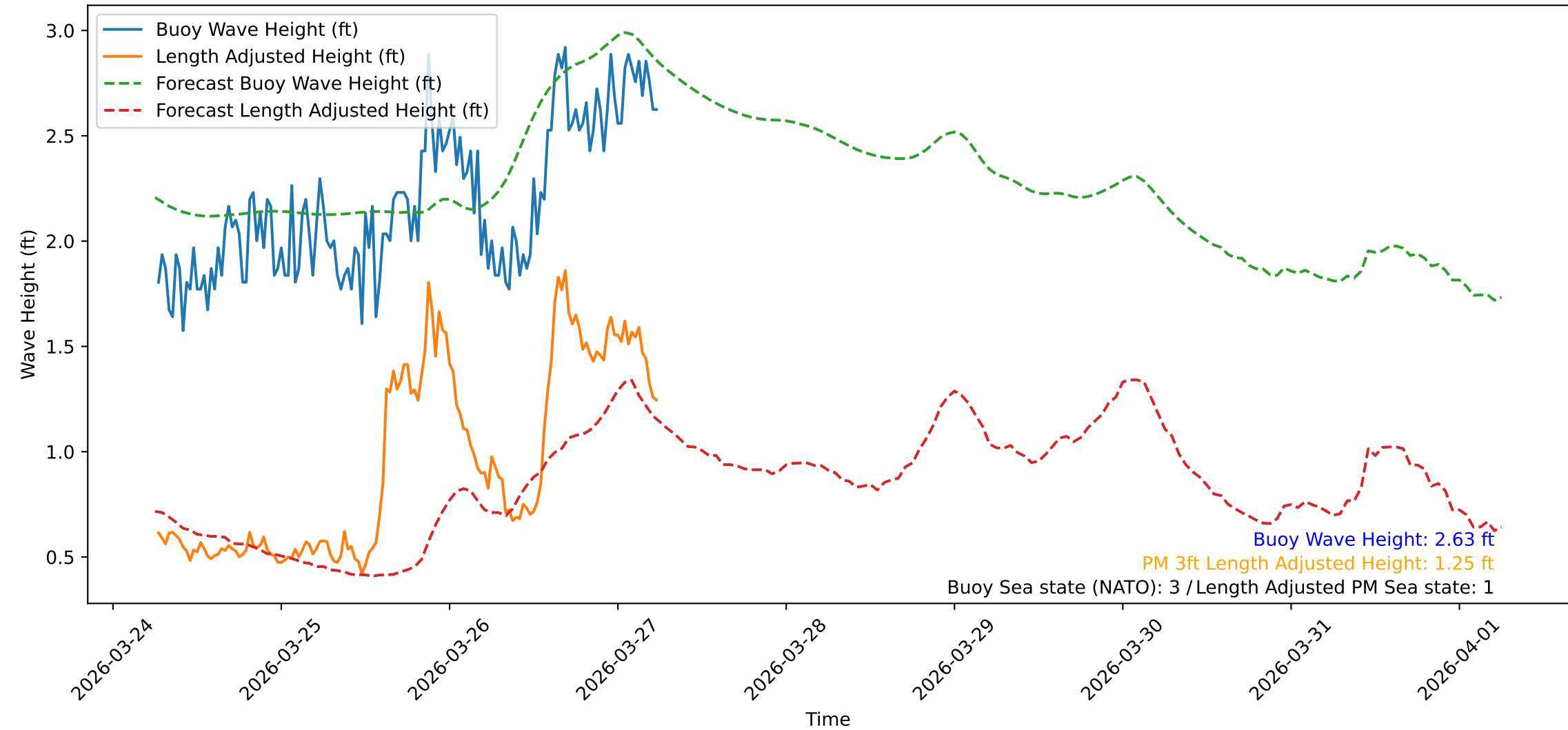
Wave Heights over Time for Oceanside Harbor at 2026-03-27 06:20:32
