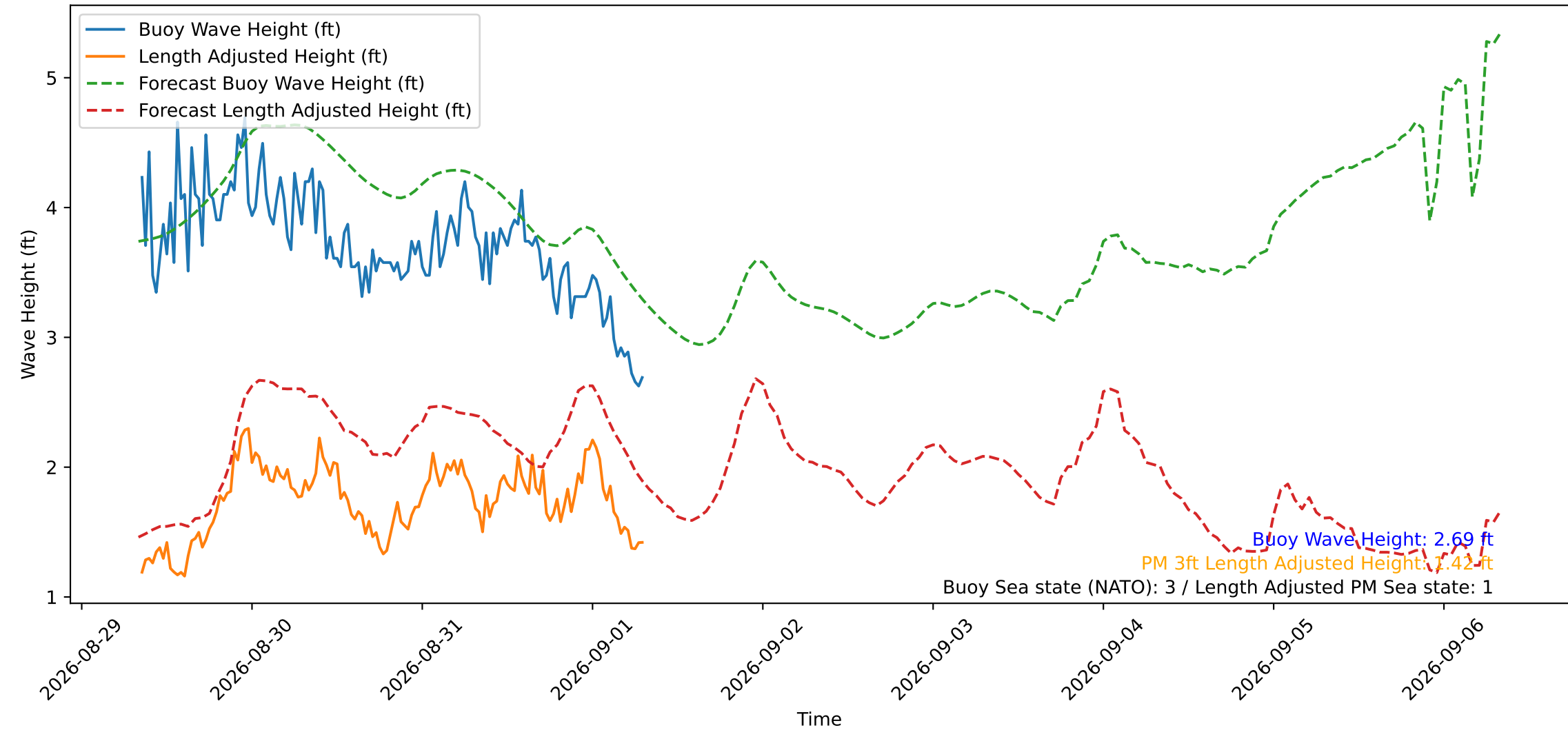
Wave Heights over Time for Red Beach at 2026-09-01 08:00:49
