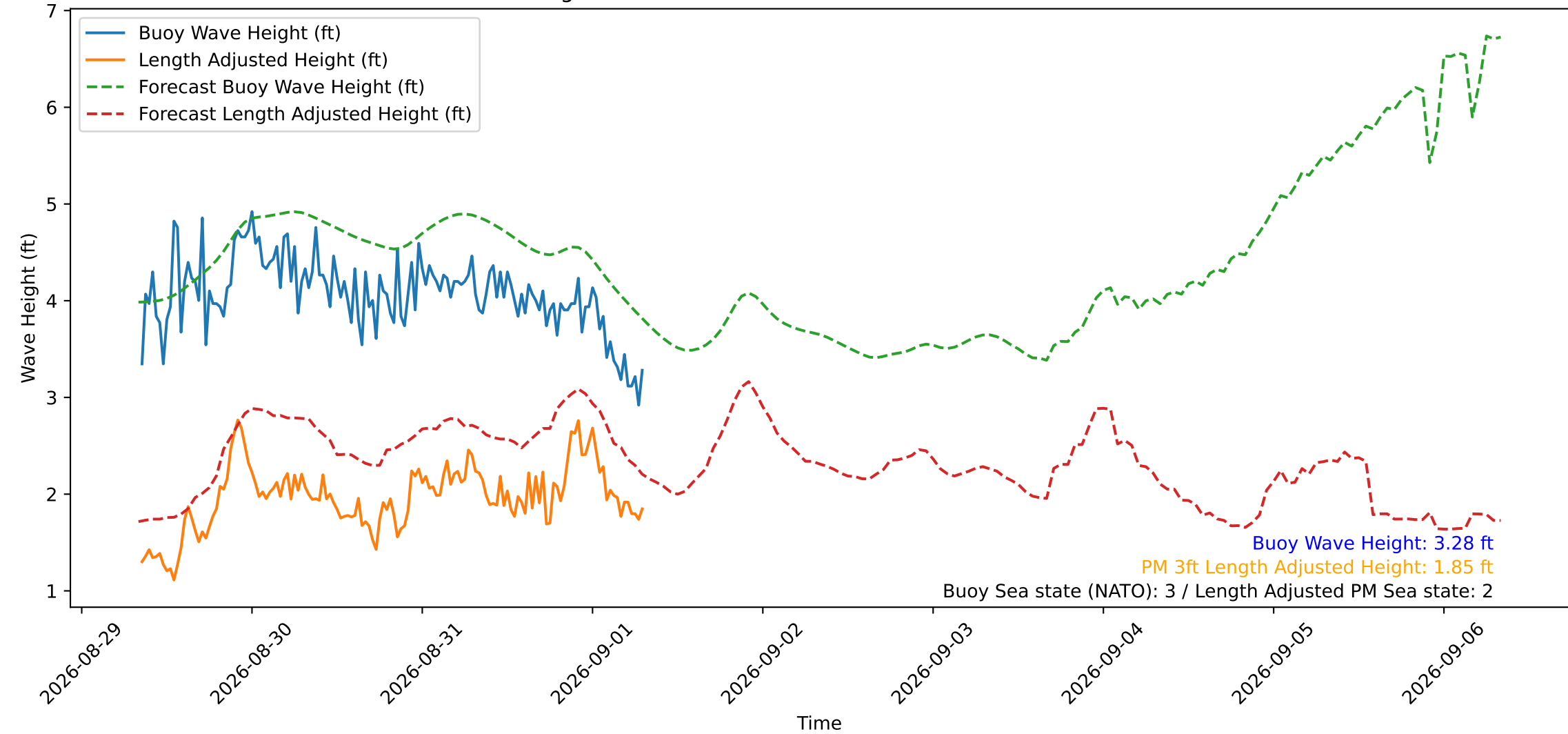
Wave Heights over Time for Green Beach at 2026-09-01 08:01:11
