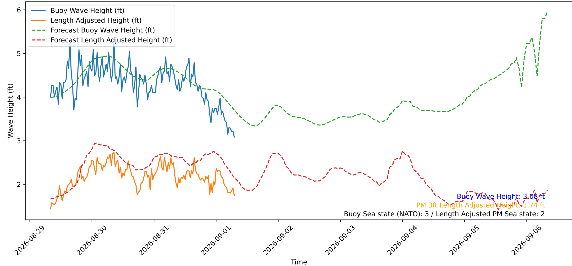
Wave Heights over Time for Oceanside Harbor at 2026-09-01 08:00:29
