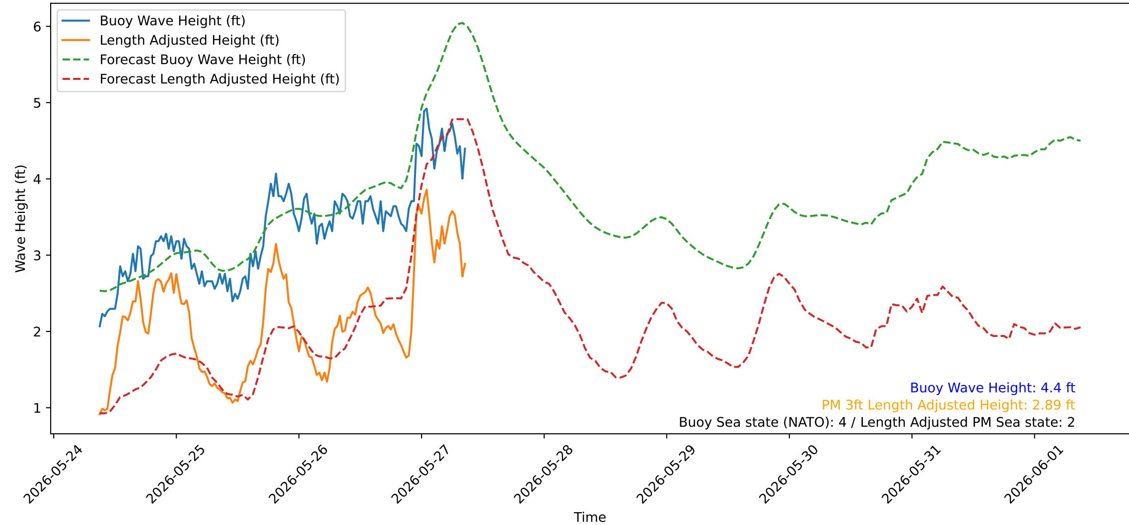
Wave Heights over Time for Green Beach at 2026-05-27 09:11:08
