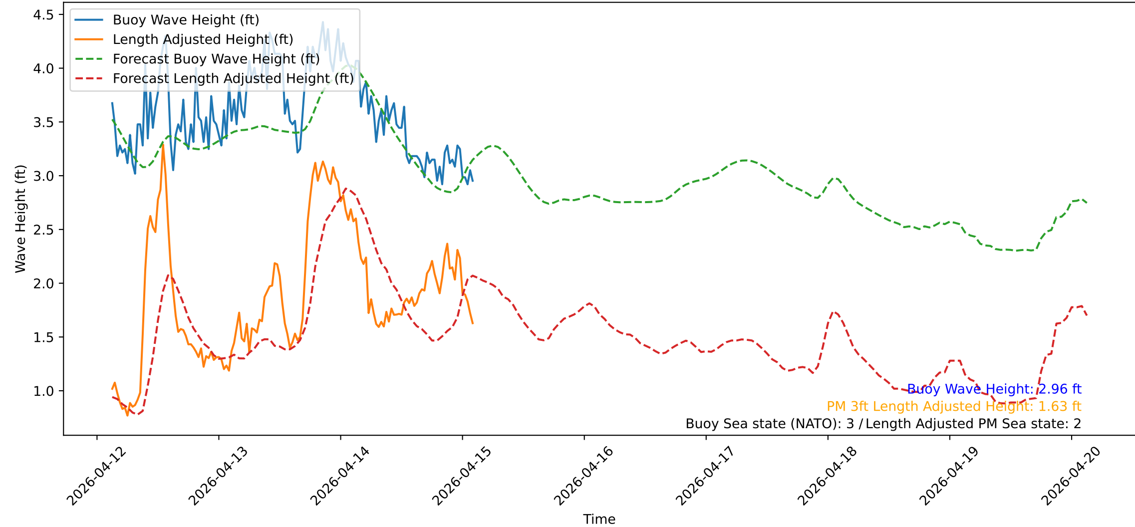
Wave Heights over Time for Red Beach at 2026-04-15 02:50:52
