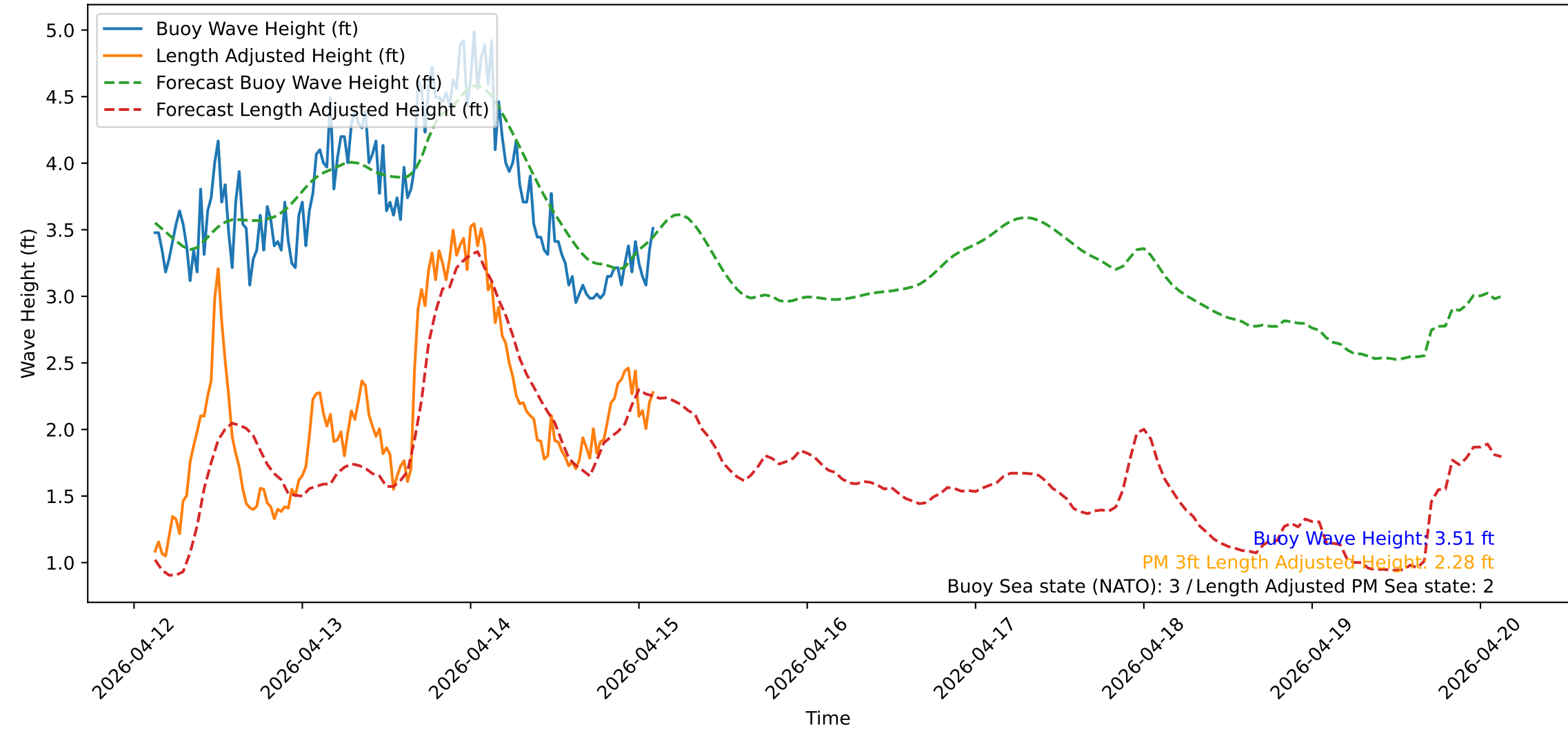
Wave Heights over Time for Green Beach at 2026-04-15 02:51:14
