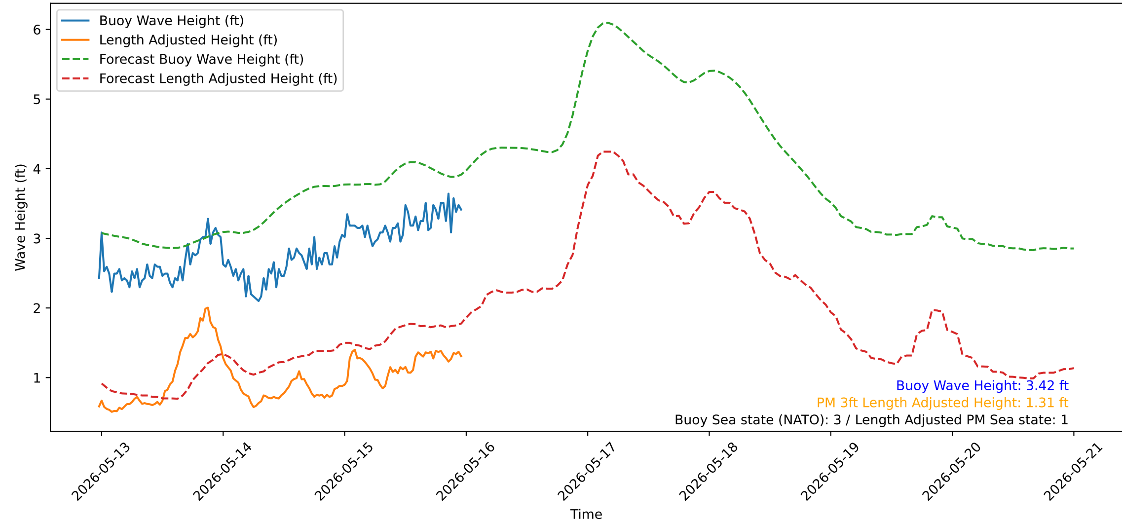
Wave Heights over Time for Green Beach at 2026-05-15 23:41:14
