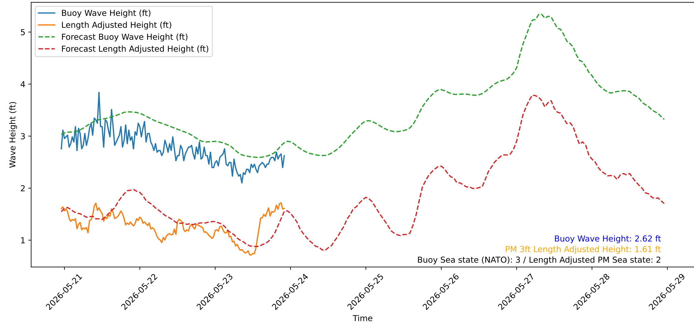
Wave Heights over Time for Oceanside Harbor at 2026-05-23 23:10:31
