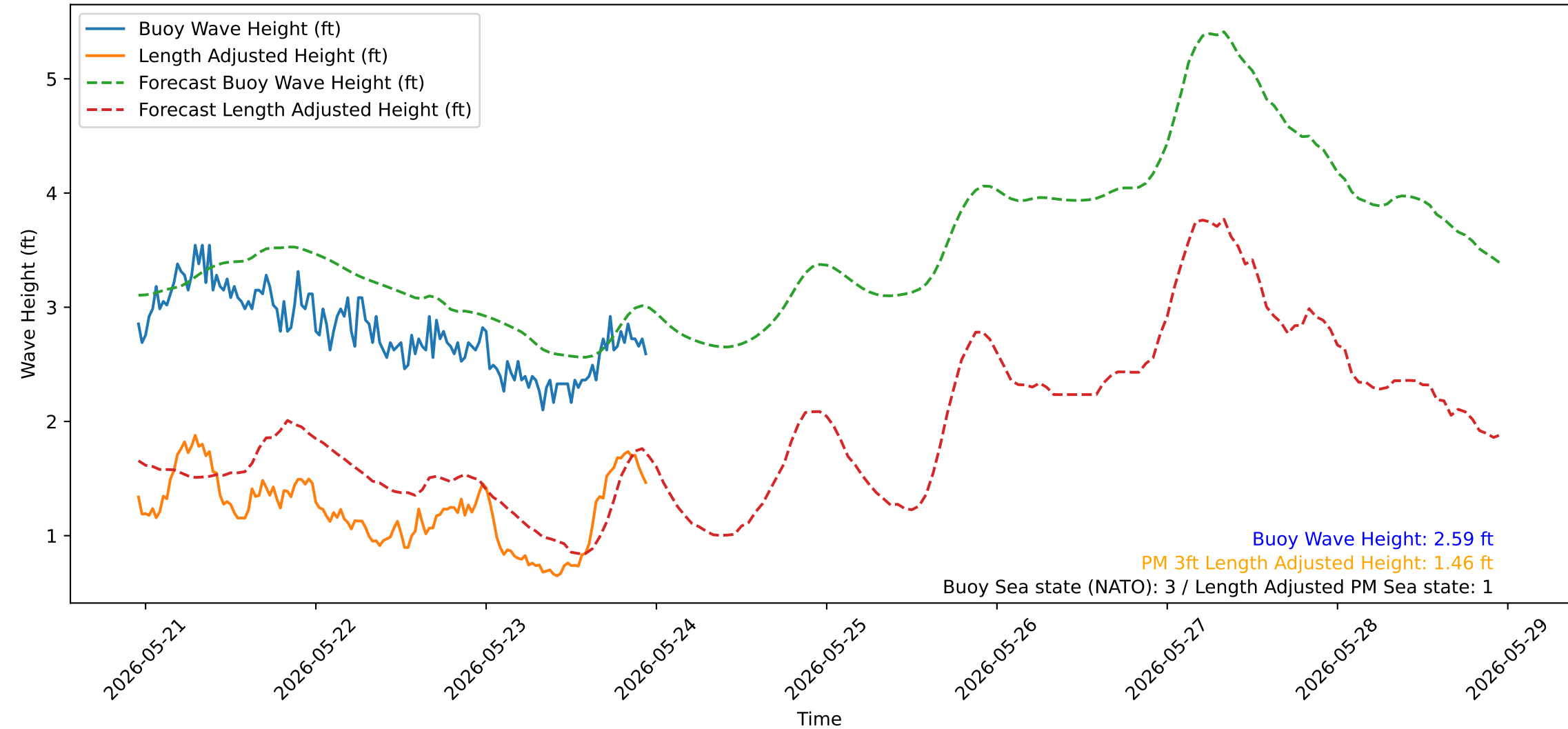
Wave Heights over Time for Green Beach at 2026-05-23 23:11:13
