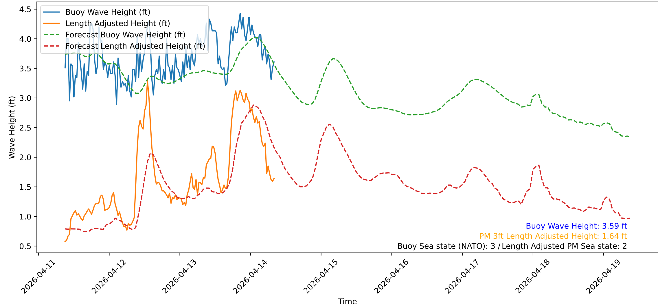
Wave Heights over Time for Red Beach at 2026-04-14 08:40:51
