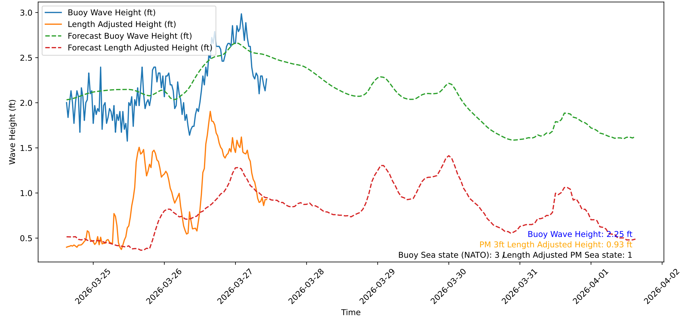
Wave Heights over Time for Red Beach at 2026-03-27 14:50:47
