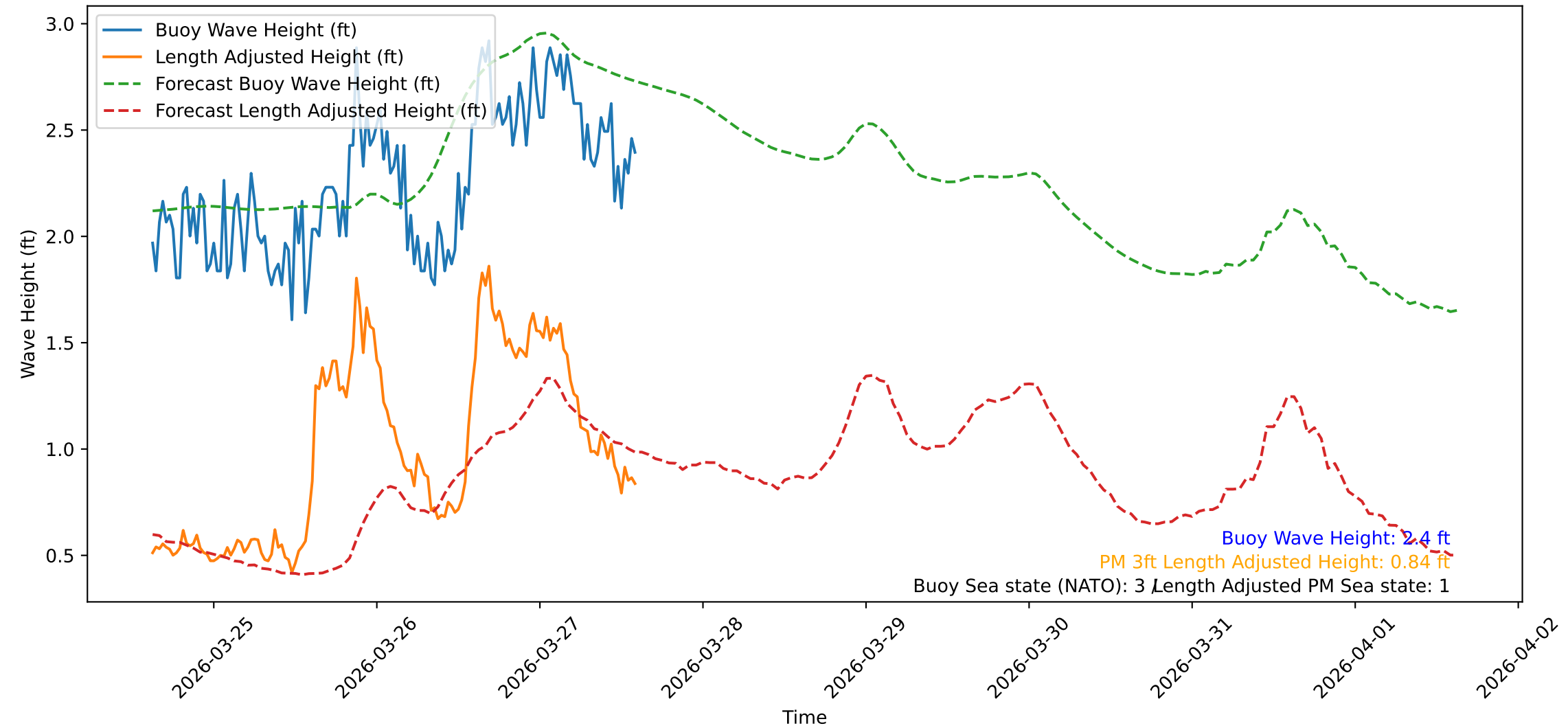
Wave Heights over Time for Oceanside Harbor at 2026-03-27 14:50:31
