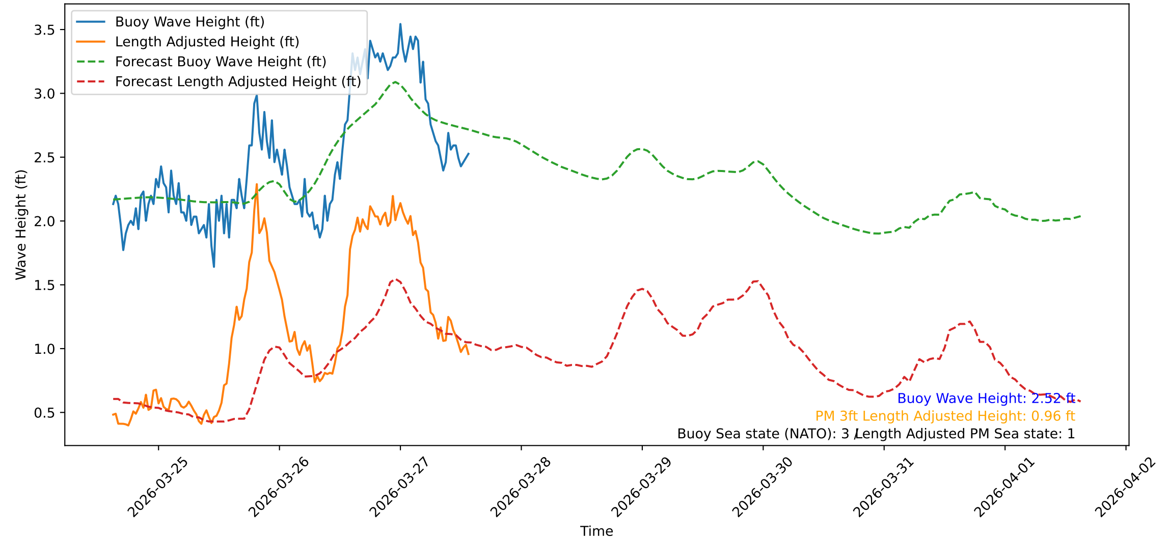
Wave Heights over Time for Green Beach at 2026-03-27 14:51:09
