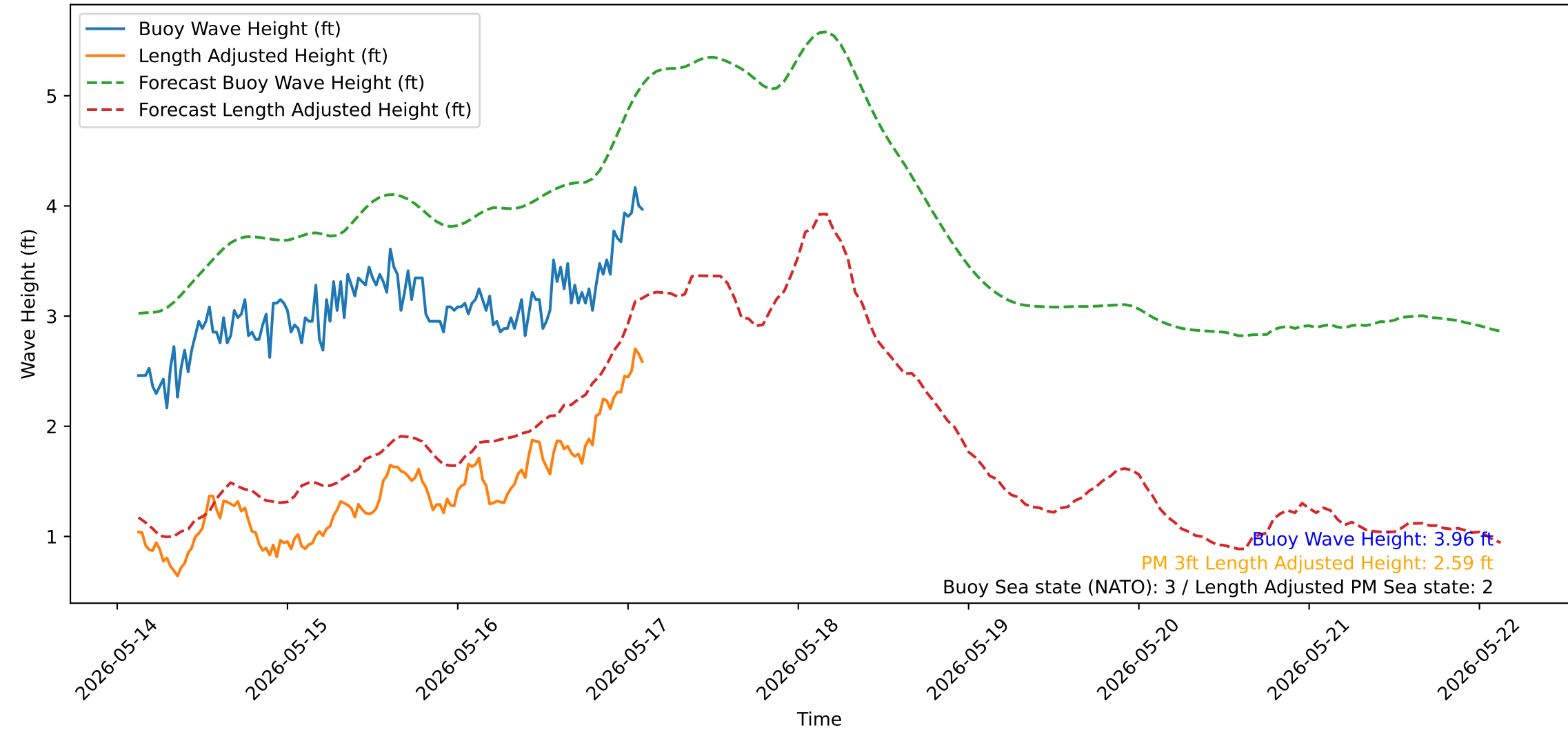
Wave Heights over Time for Oceanside Harbor at 2026-05-17 02:50:32
