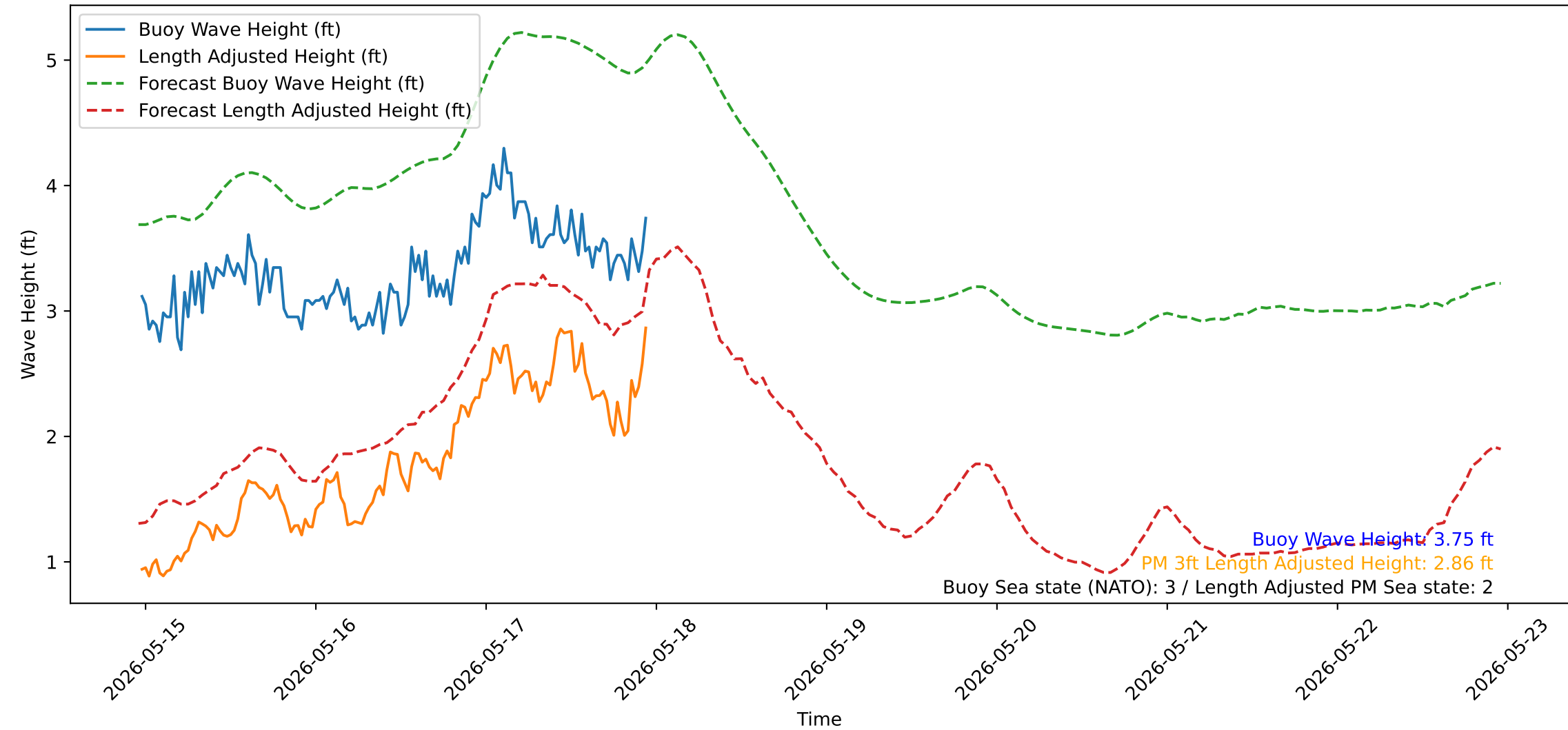
Wave Heights over Time for Oceanside Harbor at 2026-05-17 23:20:32
