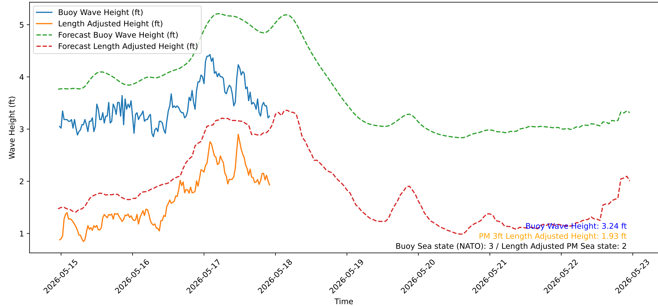
Wave Heights over Time for Green Beach at 2026-05-17 23:21:15
