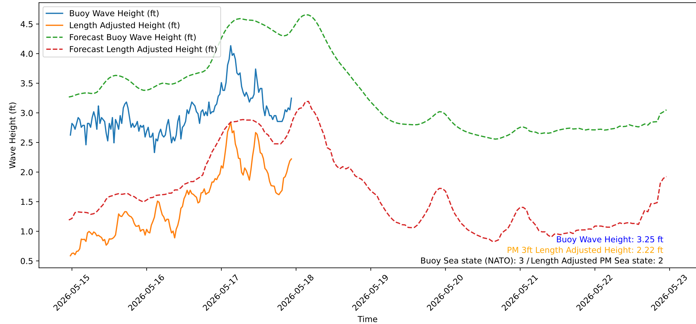
Wave Heights over Time for Red Beach at 2026-05-17 23:20:52
