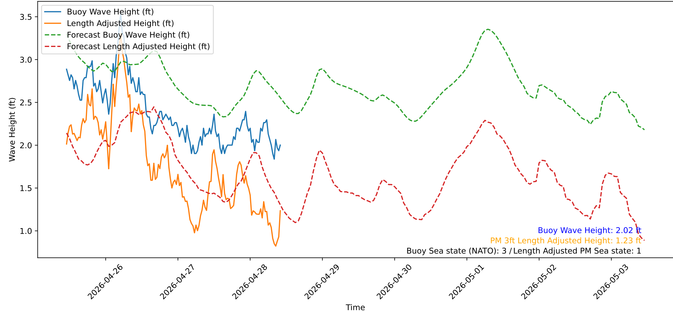
Wave Heights over Time for Red Beach at 2026-04-28 10:50:51
