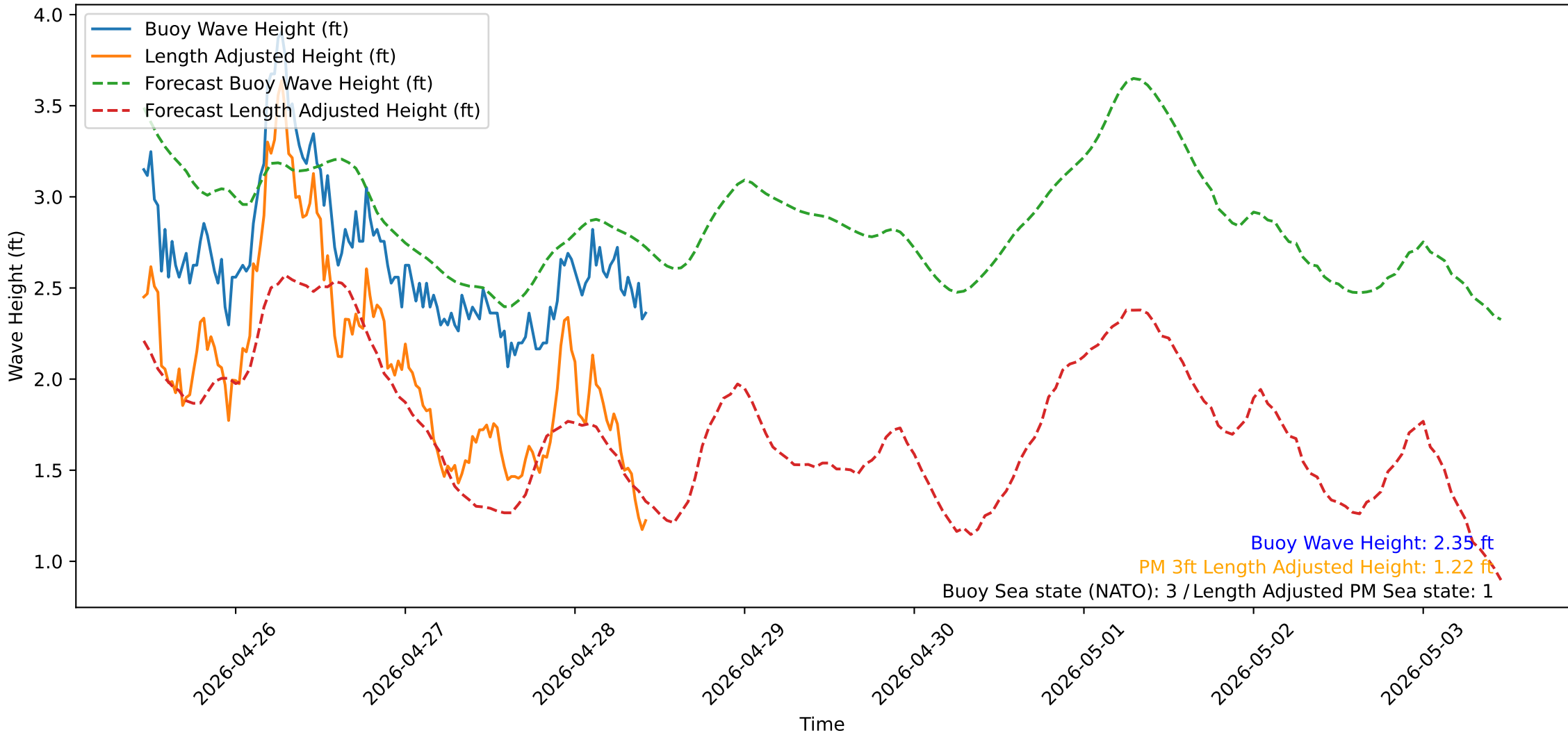
Wave Heights over Time for Oceanside Harbor at 2026-04-28 10:50:31
