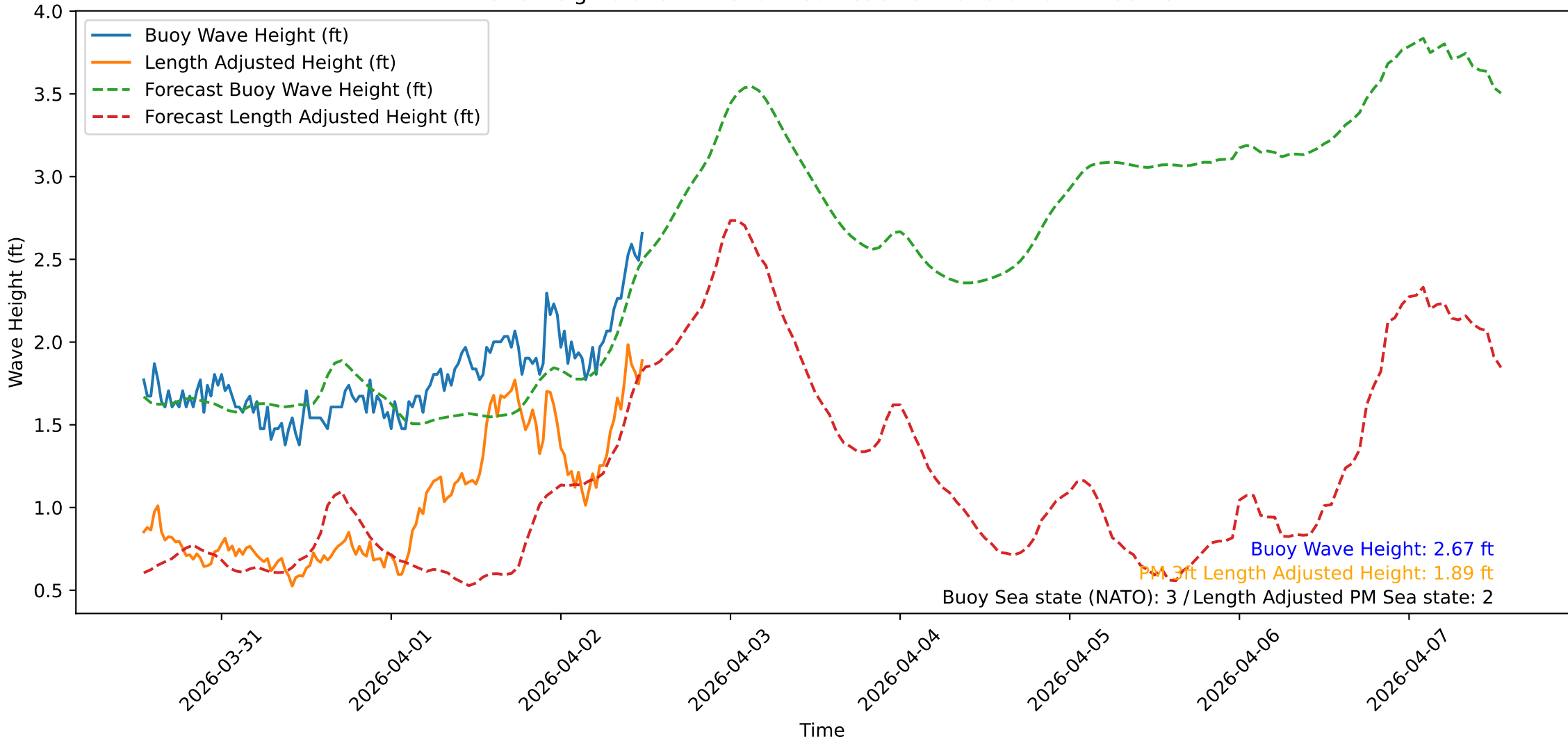
Wave Heights over Time for Red Beach at 2026-04-02 12:30:48
