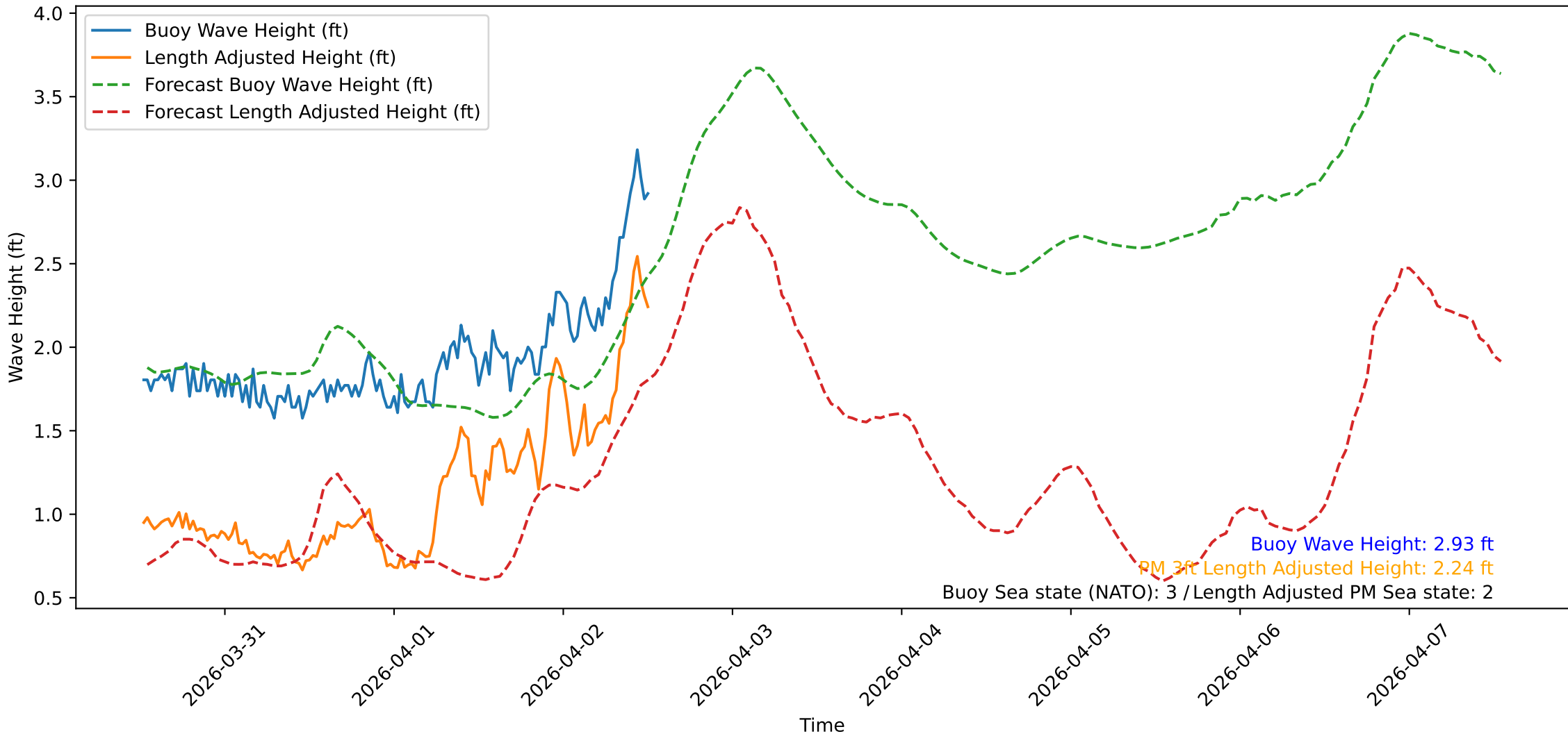
Wave Heights over Time for Oceanside Harbor at 2026-04-02 12:30:32
