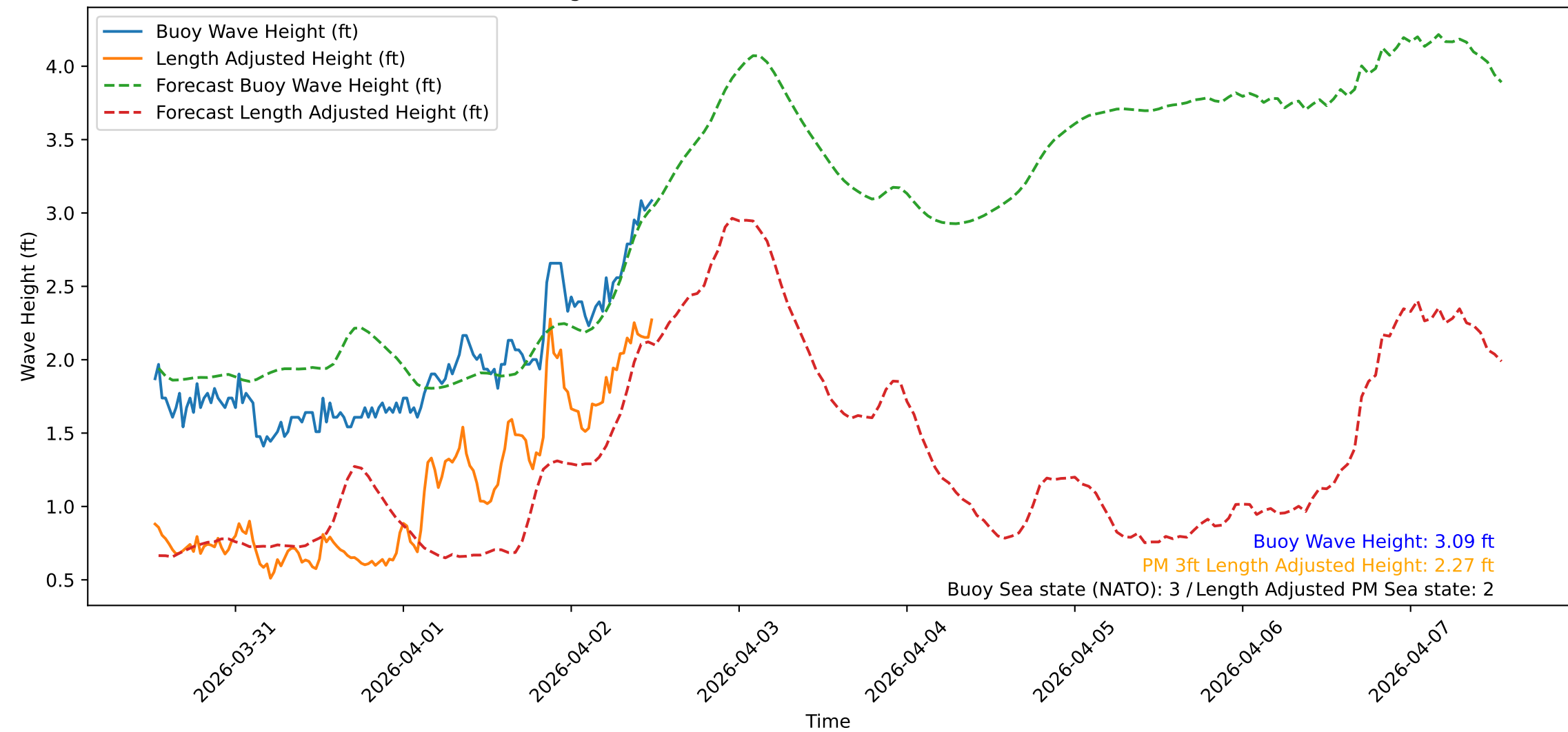
Wave Heights over Time for Green Beach at 2026-04-02 12:31:11
