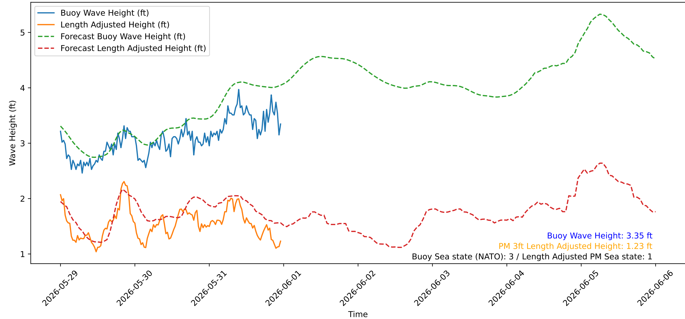
Wave Heights over Time for Green Beach at 2026-06-01 00:01:08
