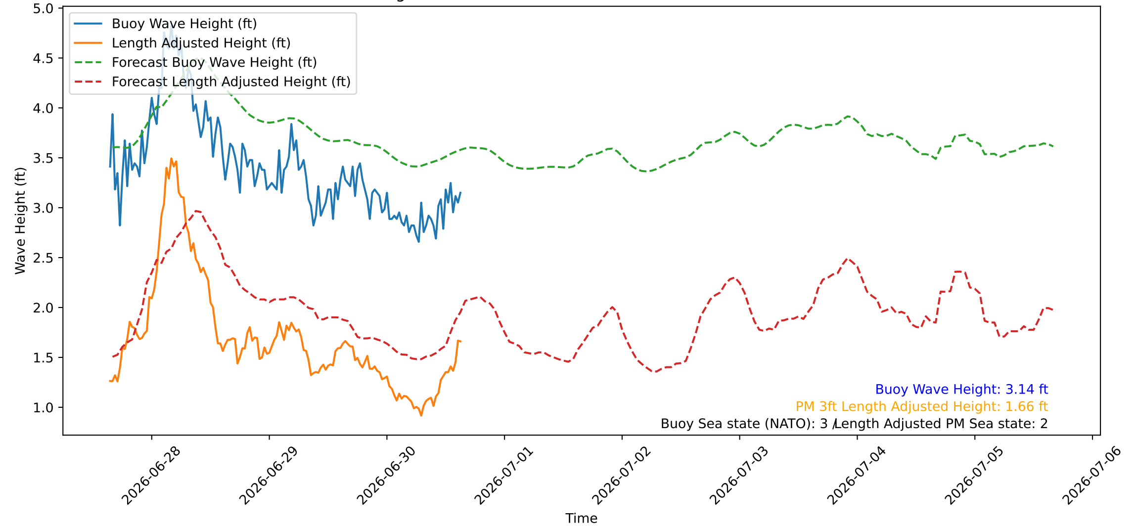
Wave Heights over Time for Green Beach at 2026-06-30 15:41:08
