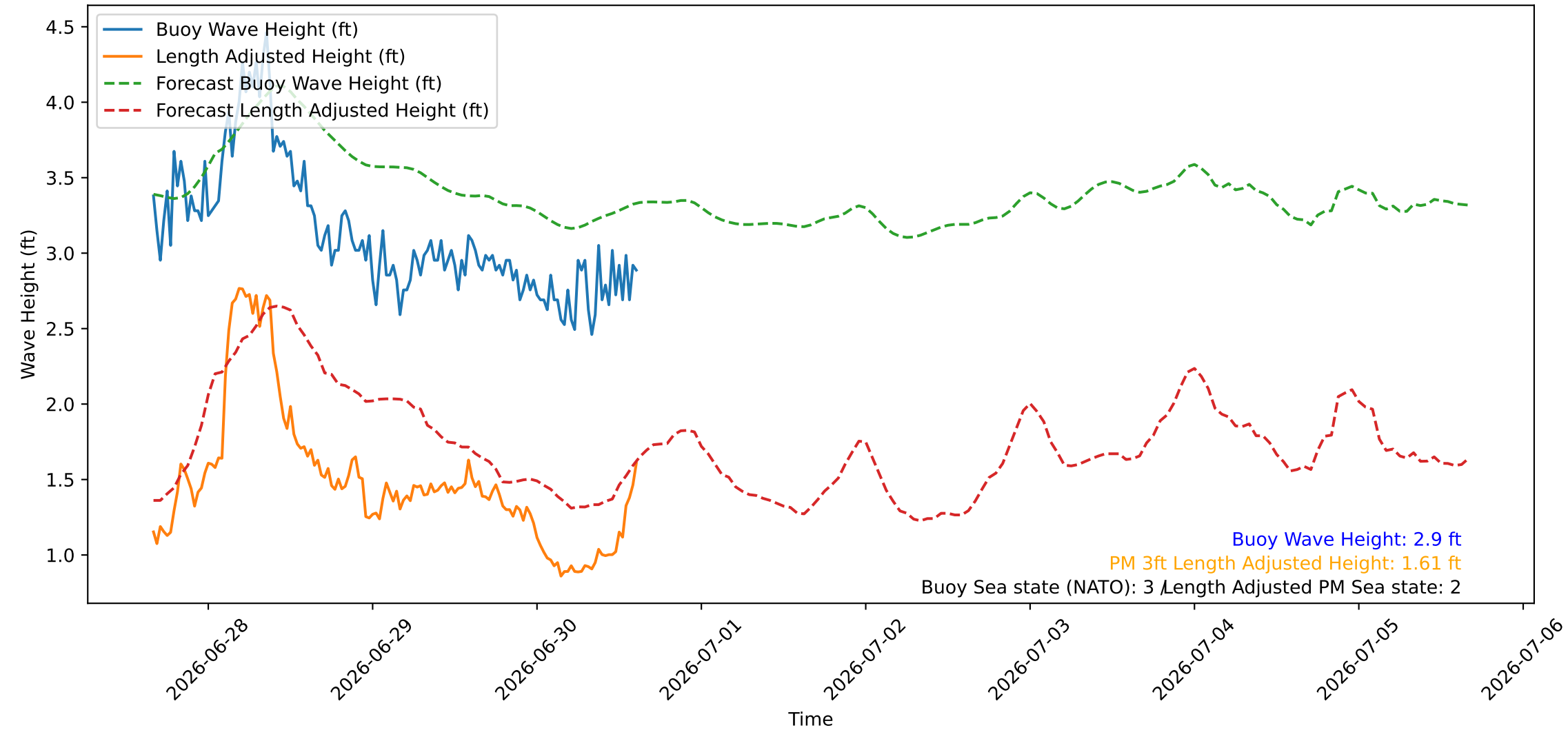
Wave Heights over Time for Red Beach at 2026-06-30 15:40:45
