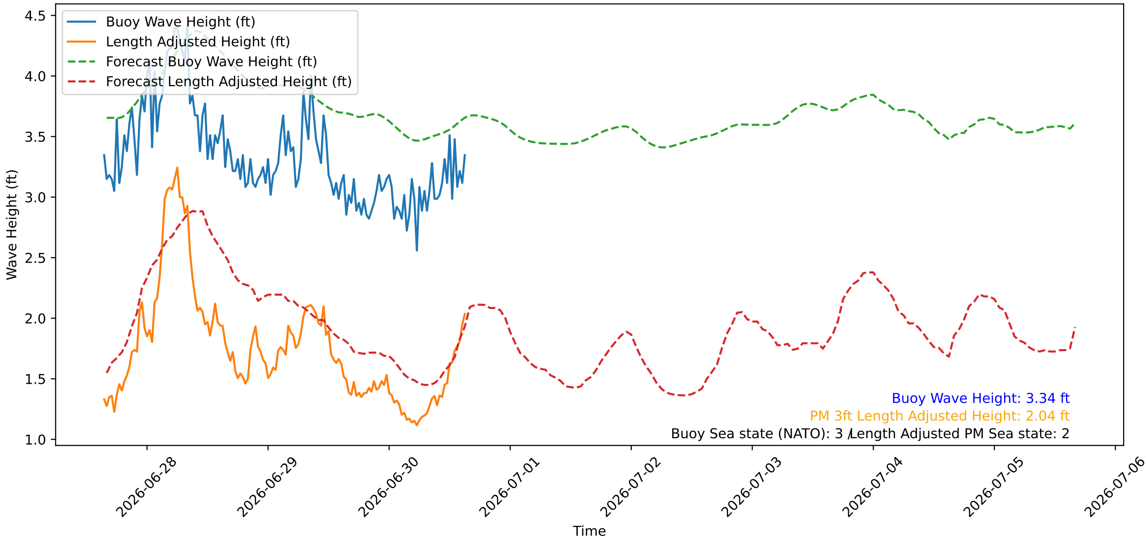
Wave Heights over Time for Oceanside Harbor at 2026-06-30 15:40:26
