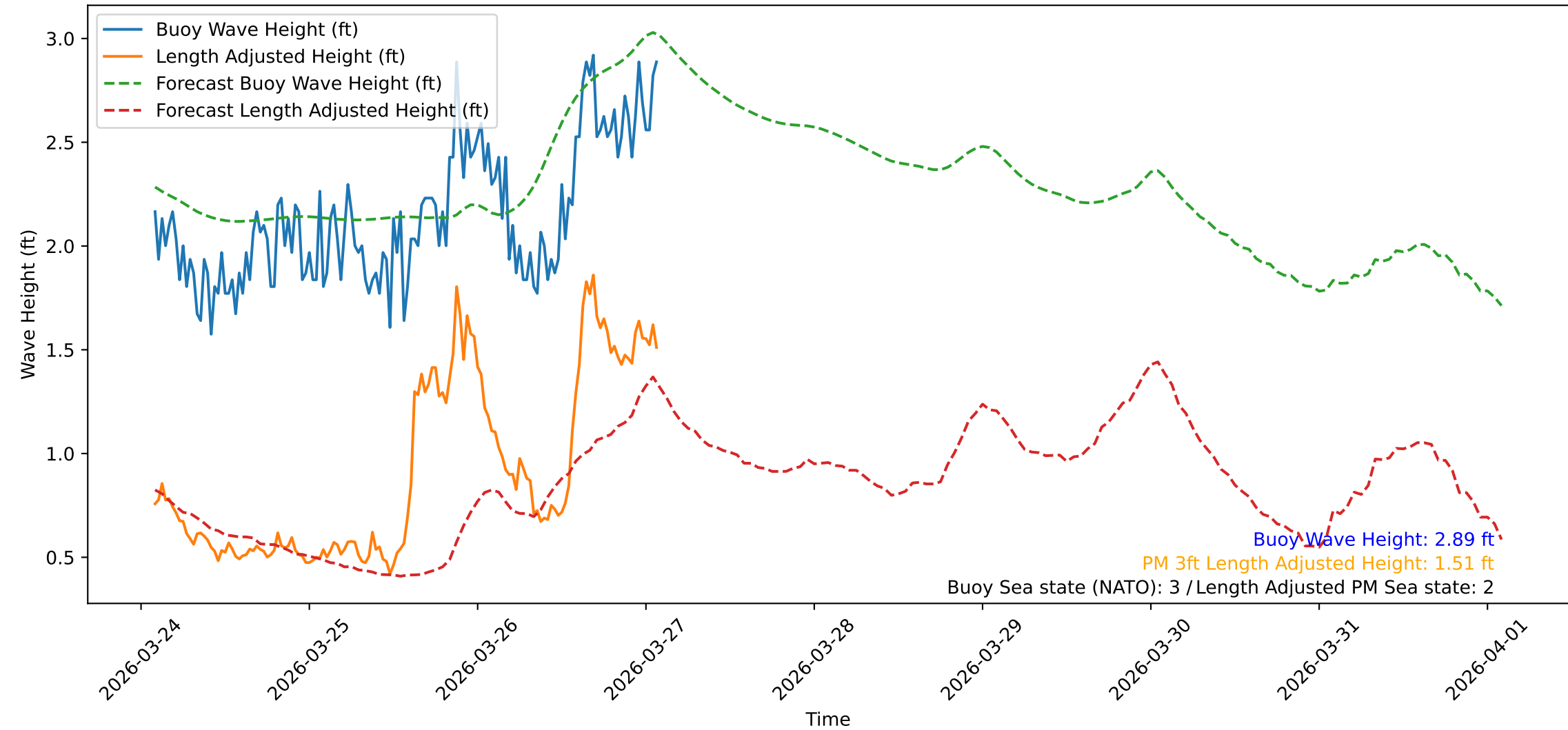
Wave Heights over Time for Oceanside Harbor at 2026-03-27 02:10:31
