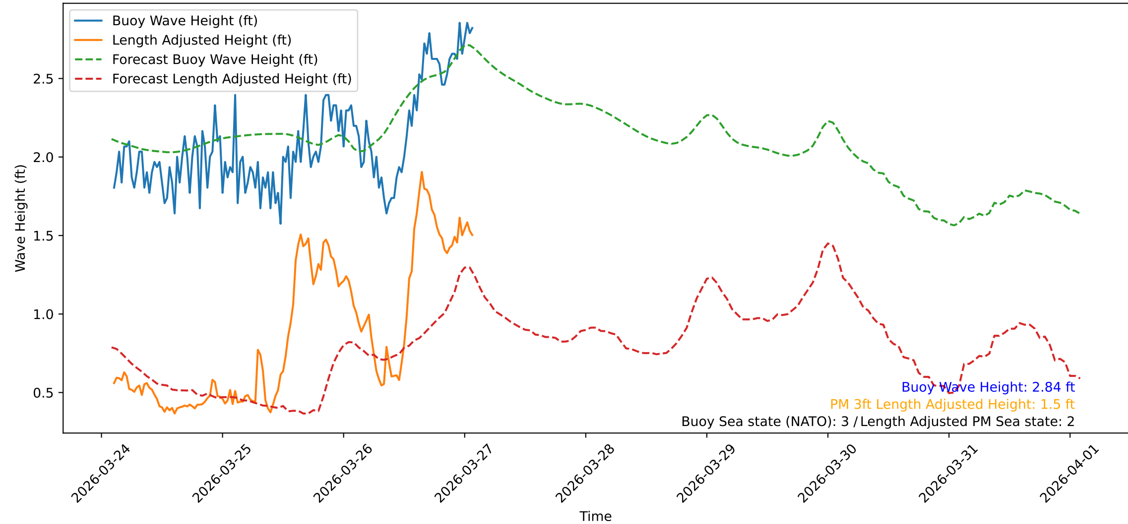
Wave Heights over Time for Red Beach at 2026-03-27 02:10:47
