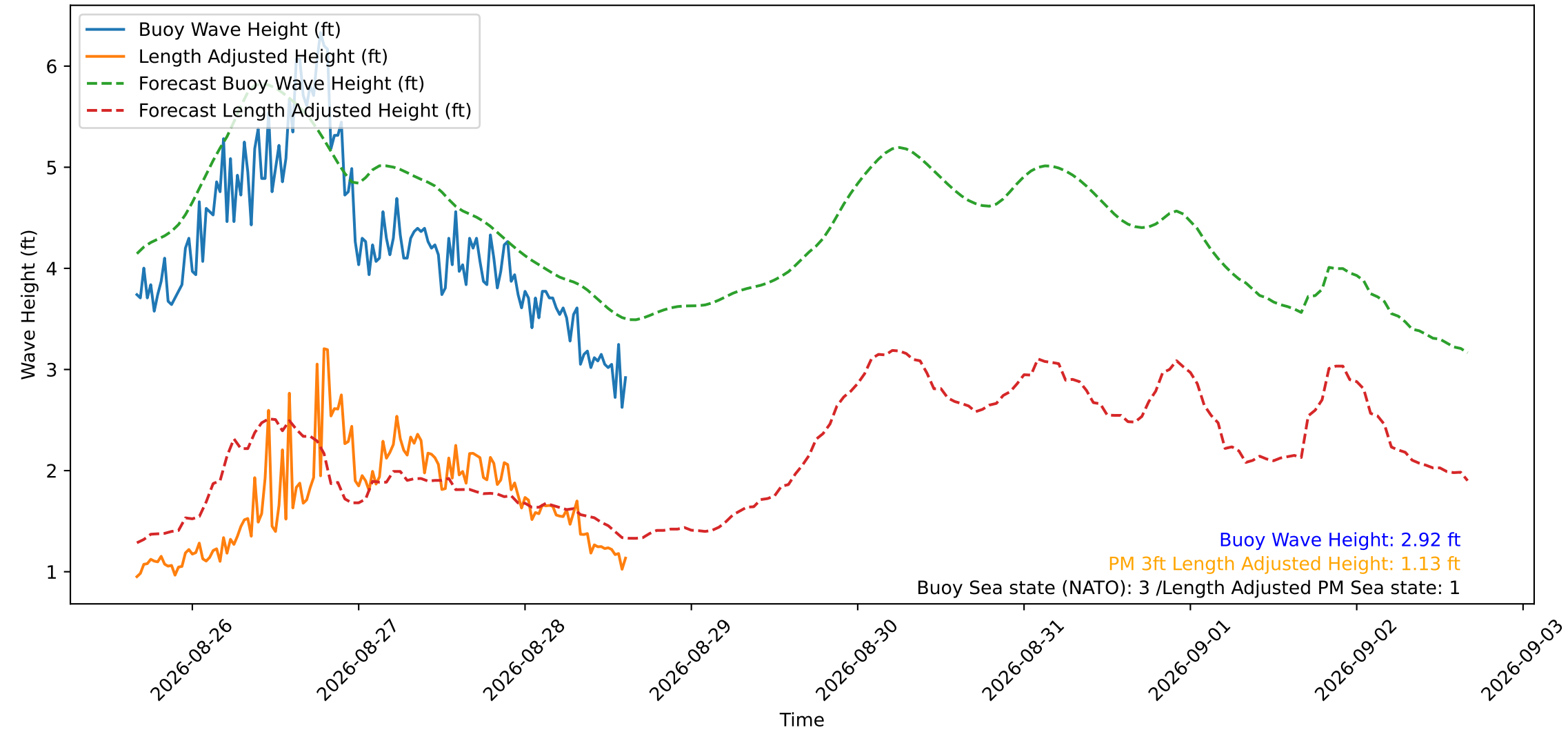
Wave Heights over Time for Green Beach at 2026-08-28 15:31:12
