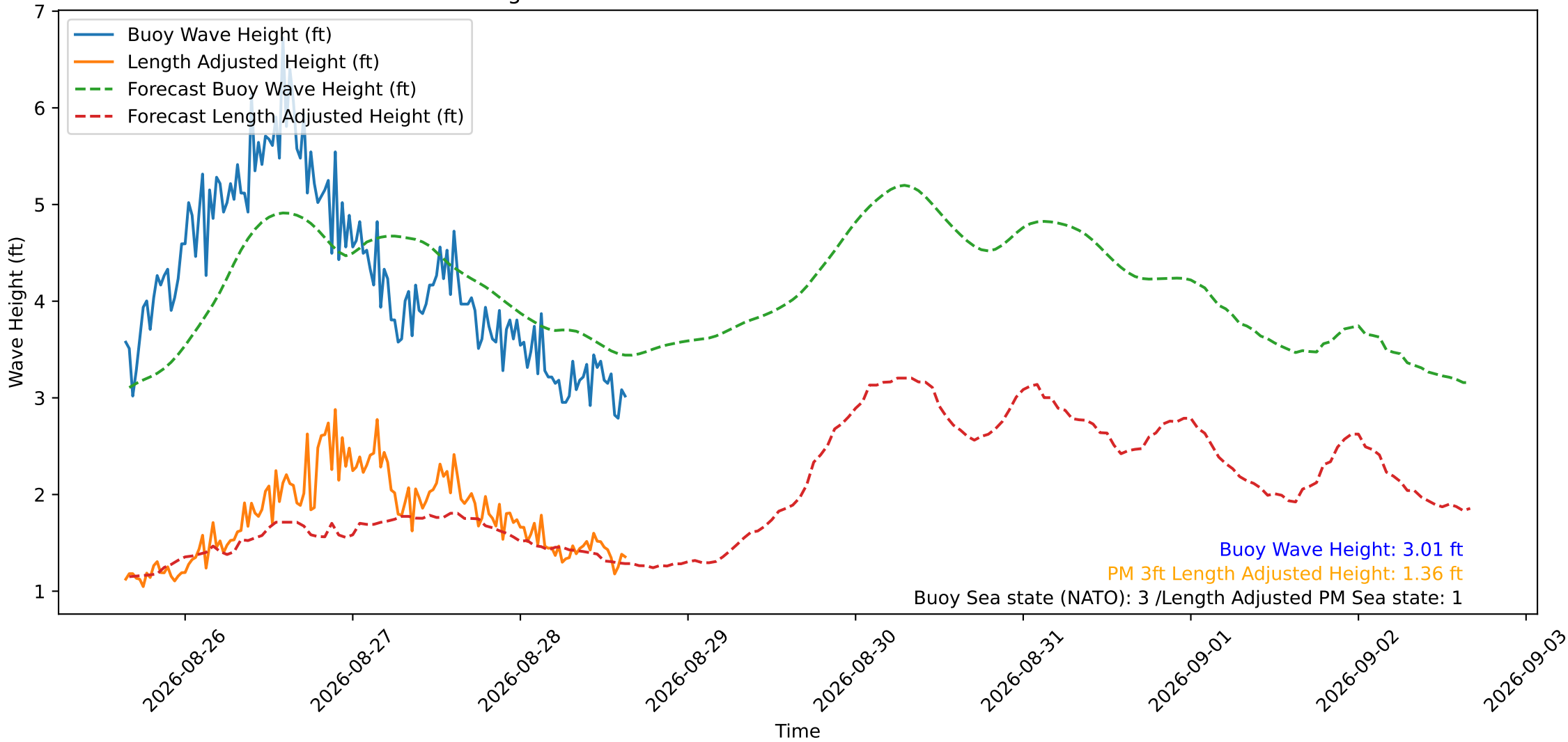
Wave Heights over Time for Oceanside Harbor at 2026-08-28 15:30:30
