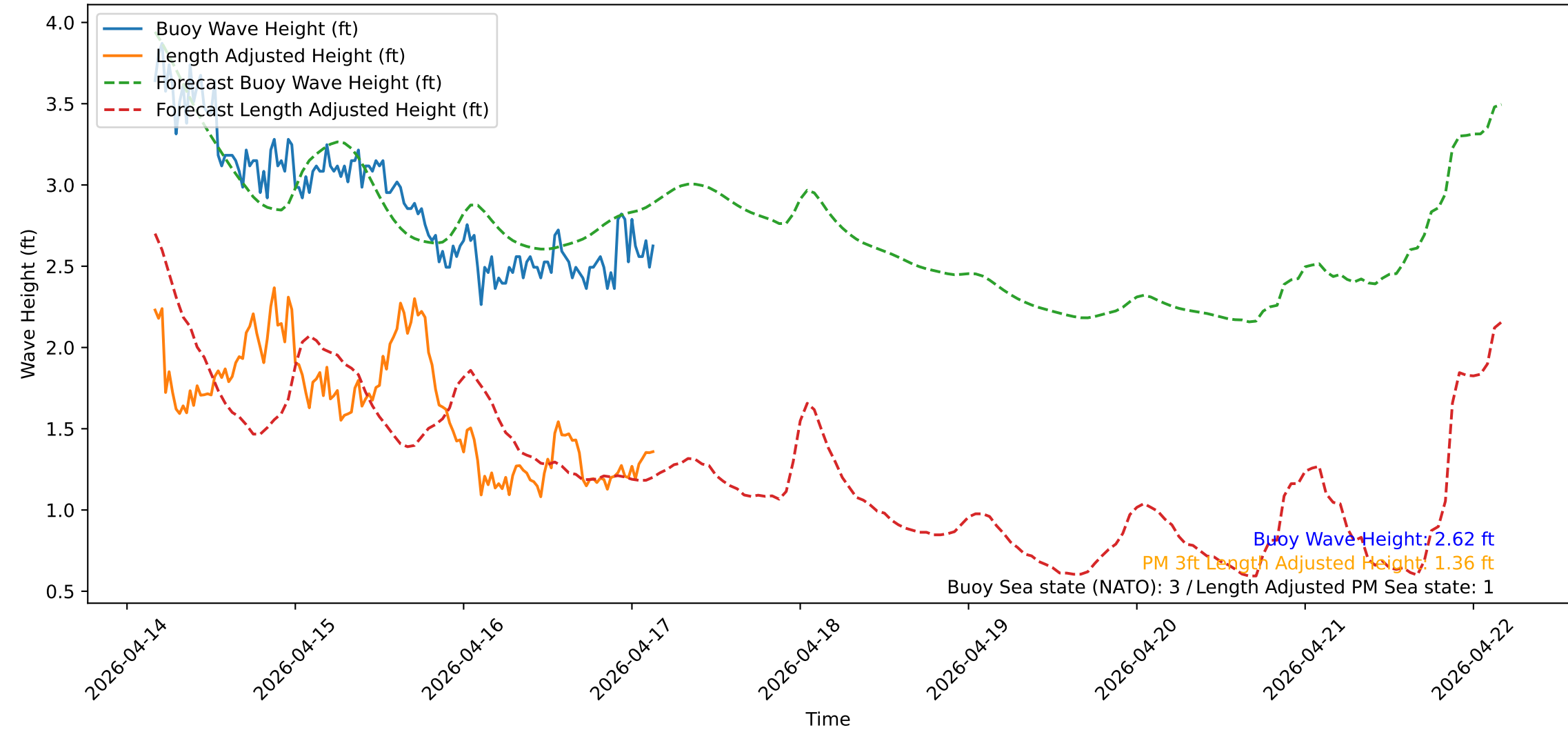
Wave Heights over Time for Red Beach at 2026-04-17 03:50:52
