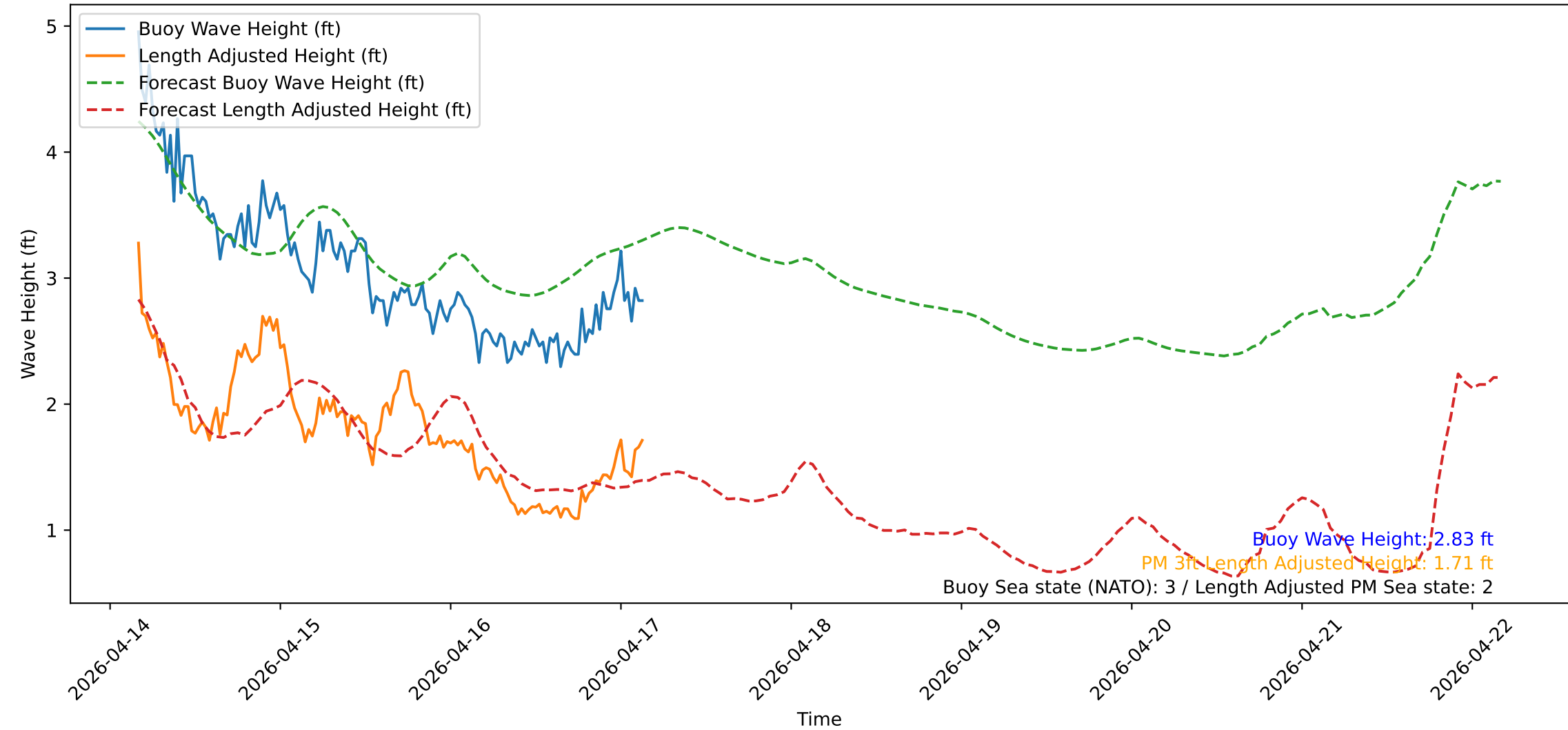
Wave Heights over Time for Oceanside Harbor at 2026-04-17 03:50:31
