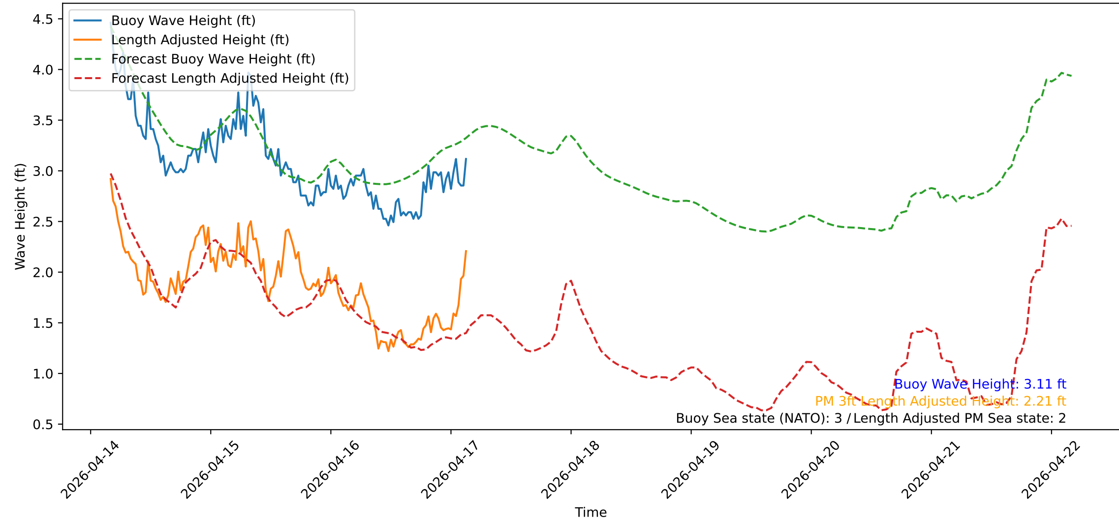
Wave Heights over Time for Green Beach at 2026-04-17 03:51:14
