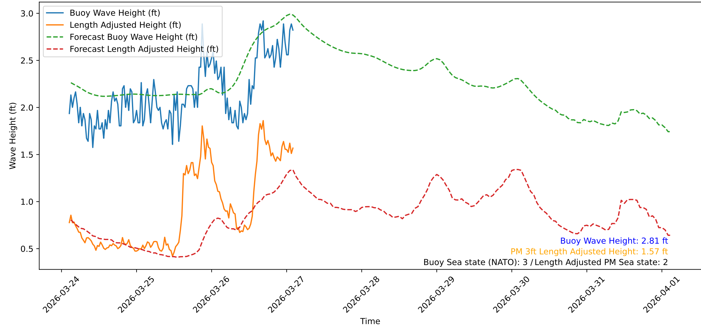
Wave Heights over Time for Oceanside Harbor at 2026-03-27 02:40:31
