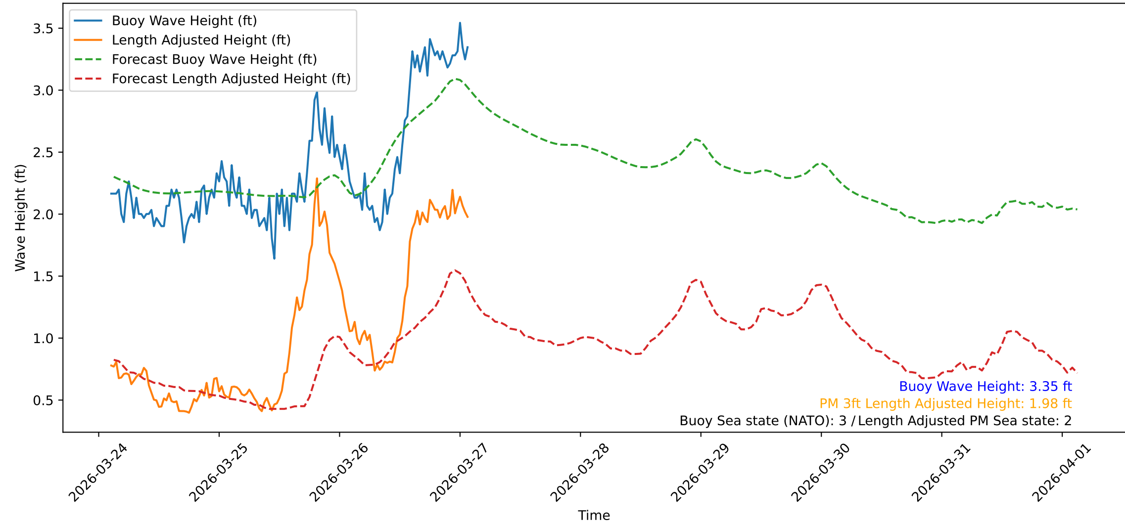
Wave Heights over Time for Green Beach at 2026-03-27 02:41:10
