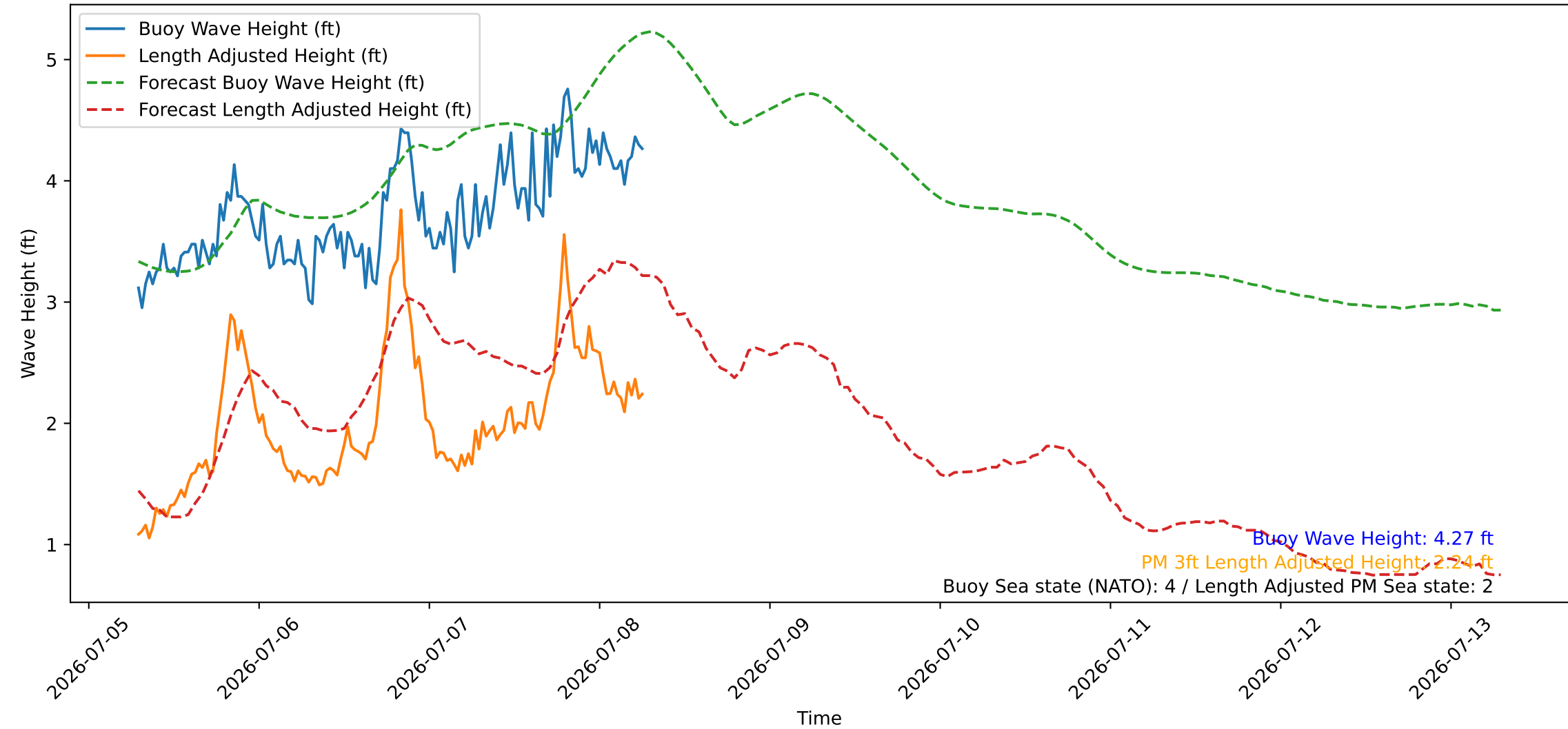
Wave Heights over Time for Green Beach at 2026-07-08 06:51:09
