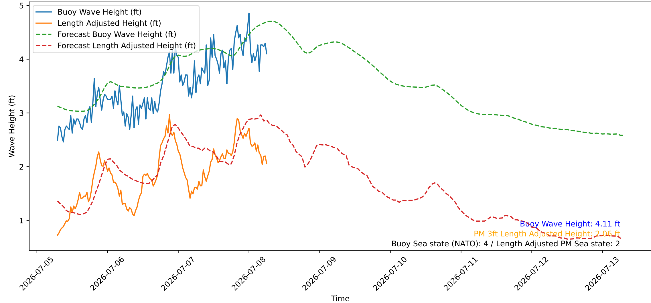
Wave Heights over Time for Red Beach at 2026-07-08 06:50:47
