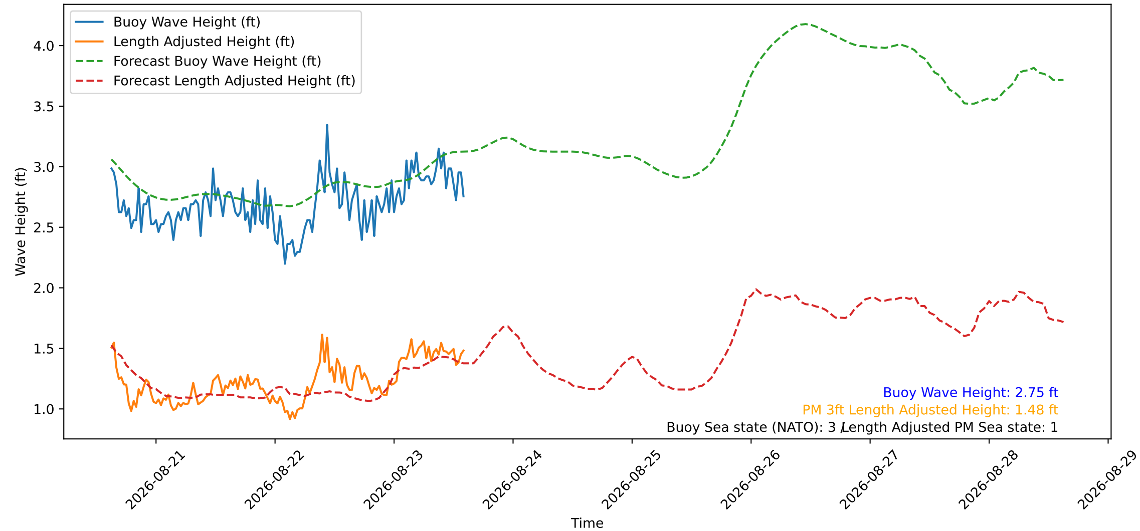
Wave Heights over Time for Oceanside Harbor at 2026-08-23 14:50:29
