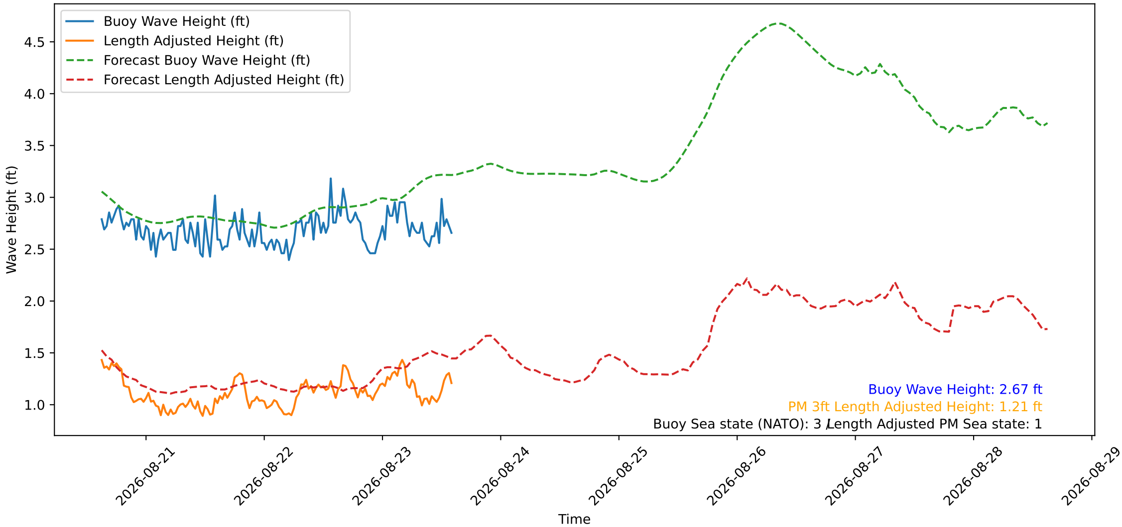
Wave Heights over Time for Green Beach at 2026-08-23 14:51:13
