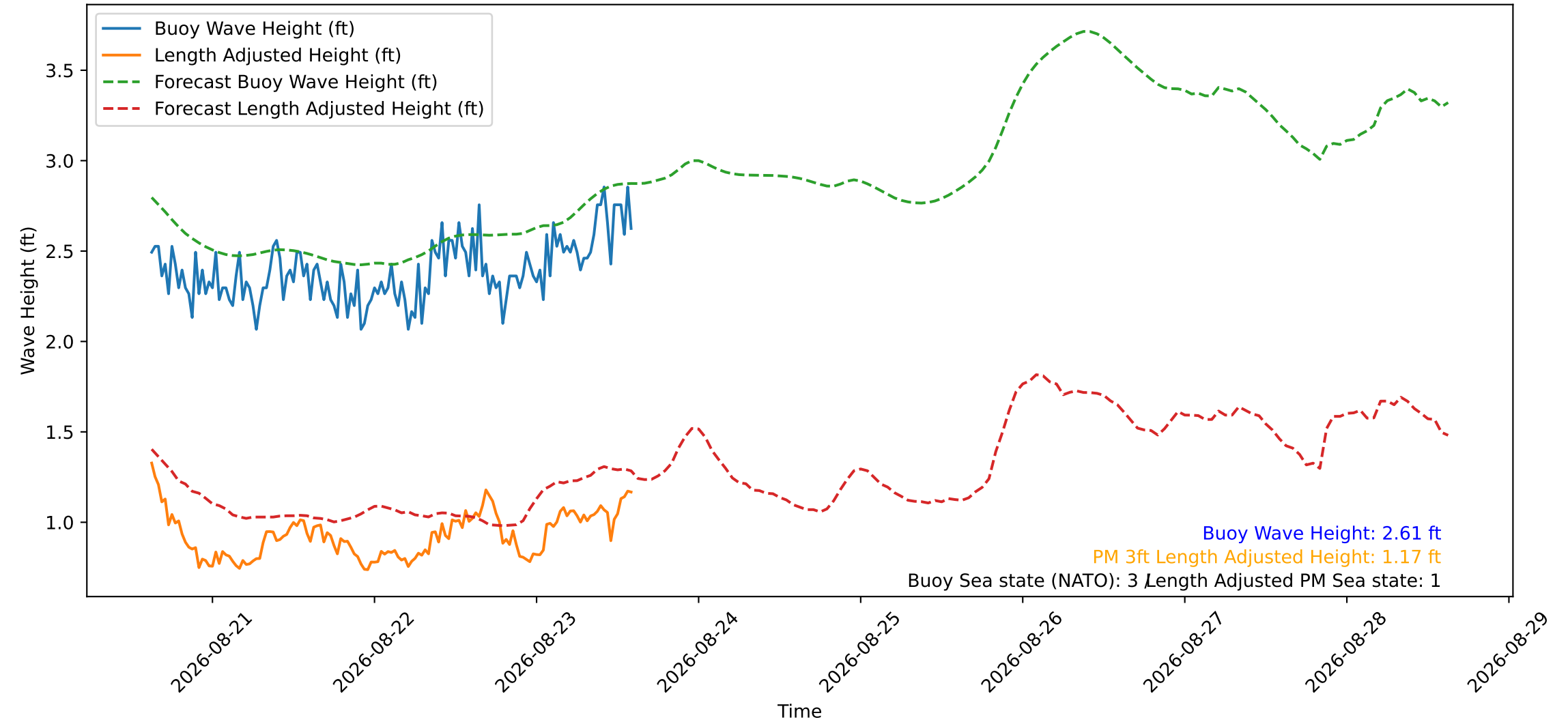
Wave Heights over Time for Red Beach at 2026-08-23 14:50:50
