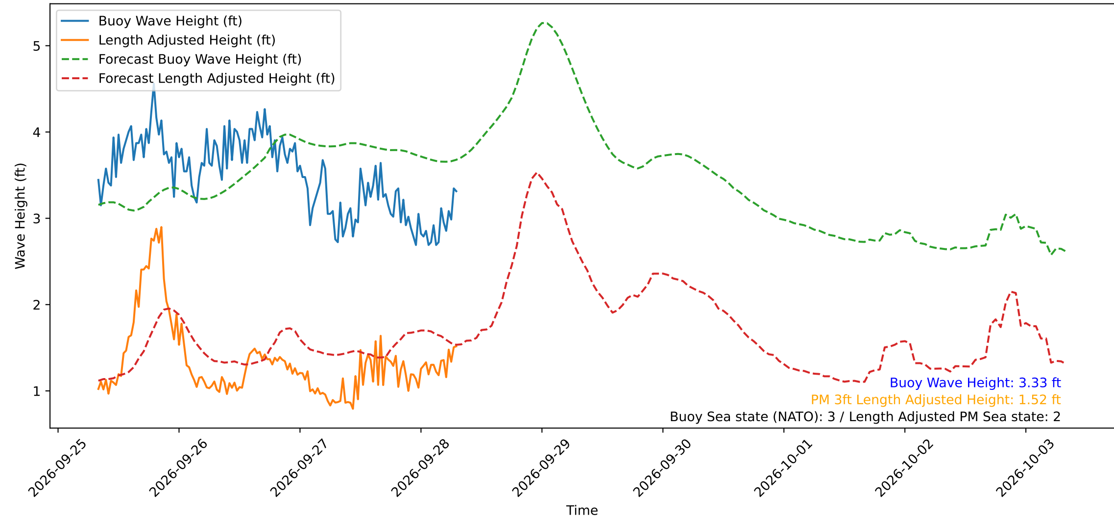
Wave Heights over Time for Green Beach at 2026-09-28 07:51:15
