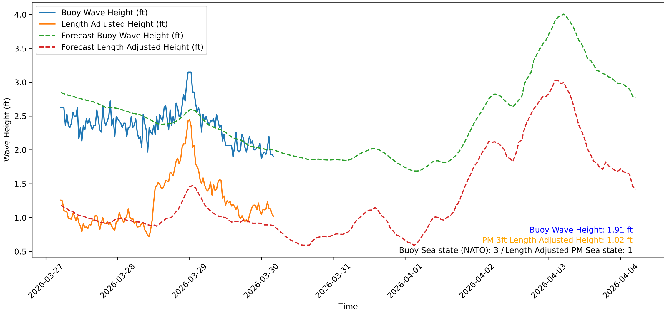
Wave Heights over Time for Oceanside Harbor at 2026-03-30 05:10:31
