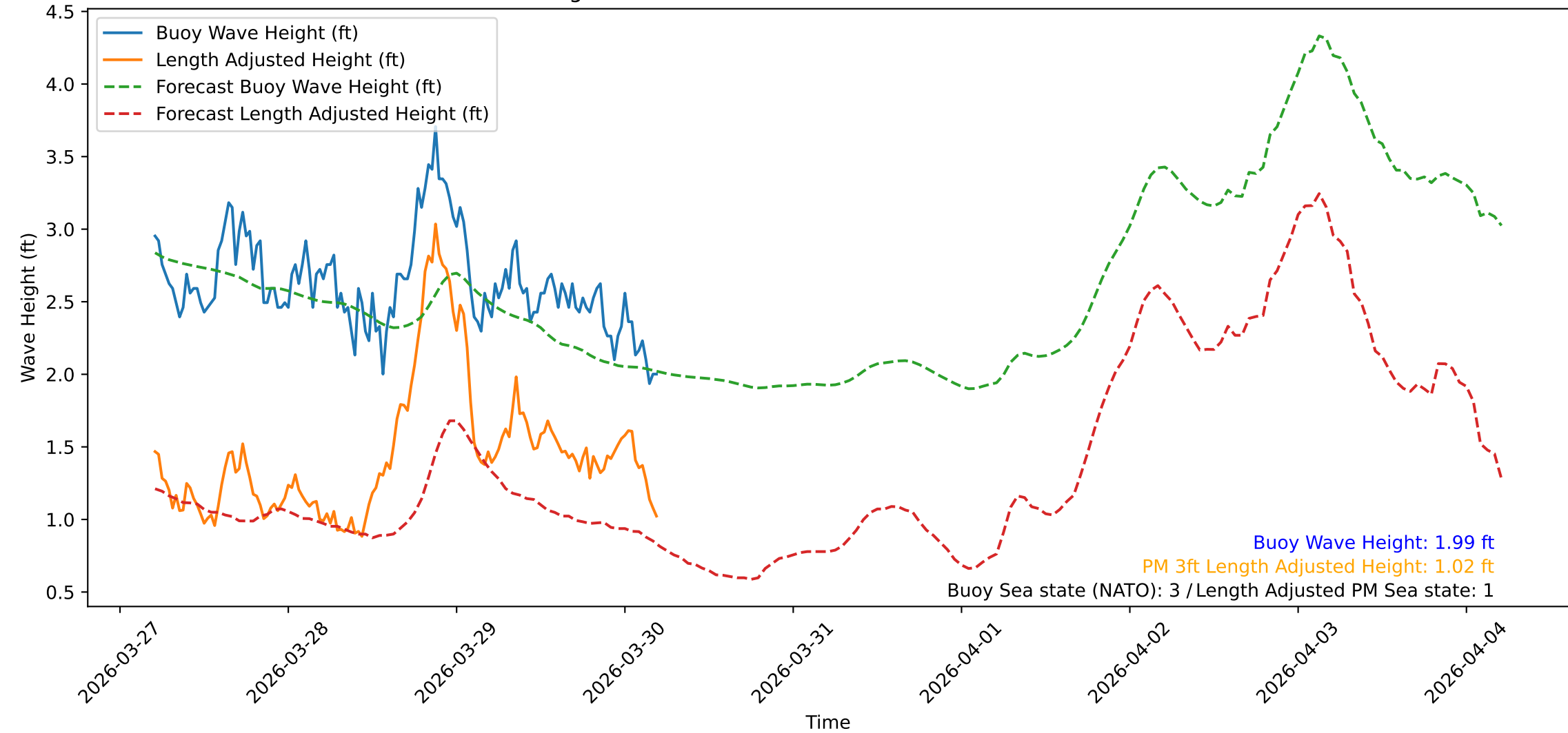
Wave Heights over Time for Green Beach at 2026-03-30 05:11:10
