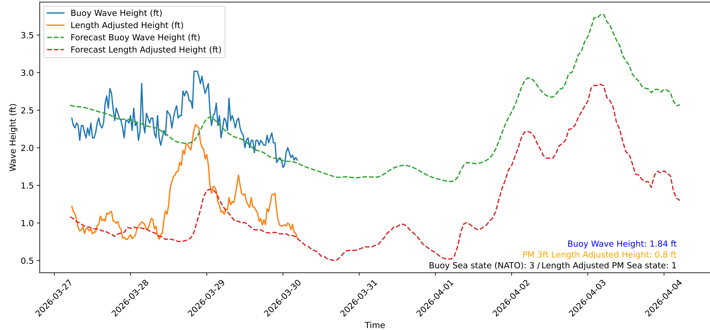
Wave Heights over Time for Red Beach at 2026-03-30 05:10:47
