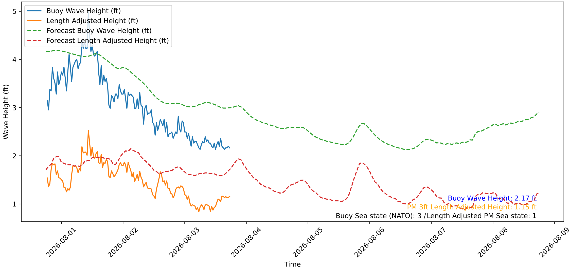
Wave Heights over Time for Green Beach at 2026-08-03 18:21:09
