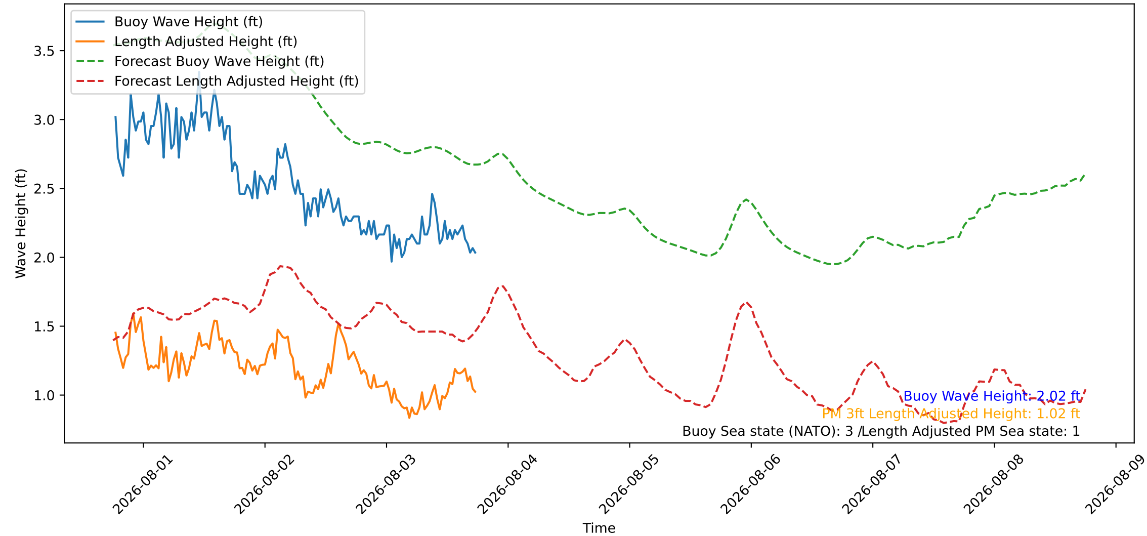
Wave Heights over Time for Red Beach at 2026-08-03 18:20:46
