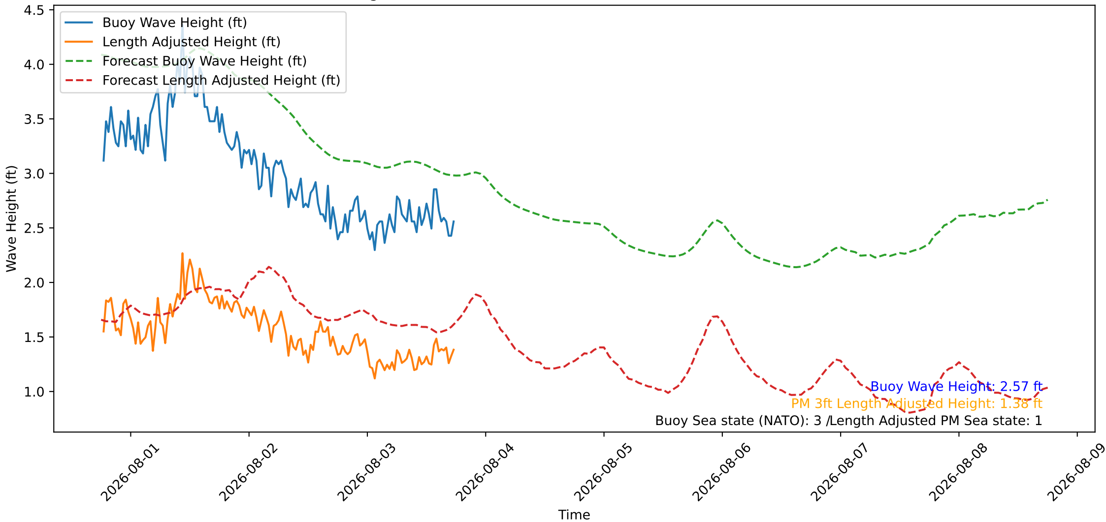
Wave Heights over Time for Oceanside Harbor at 2026-08-03 18:20:26
