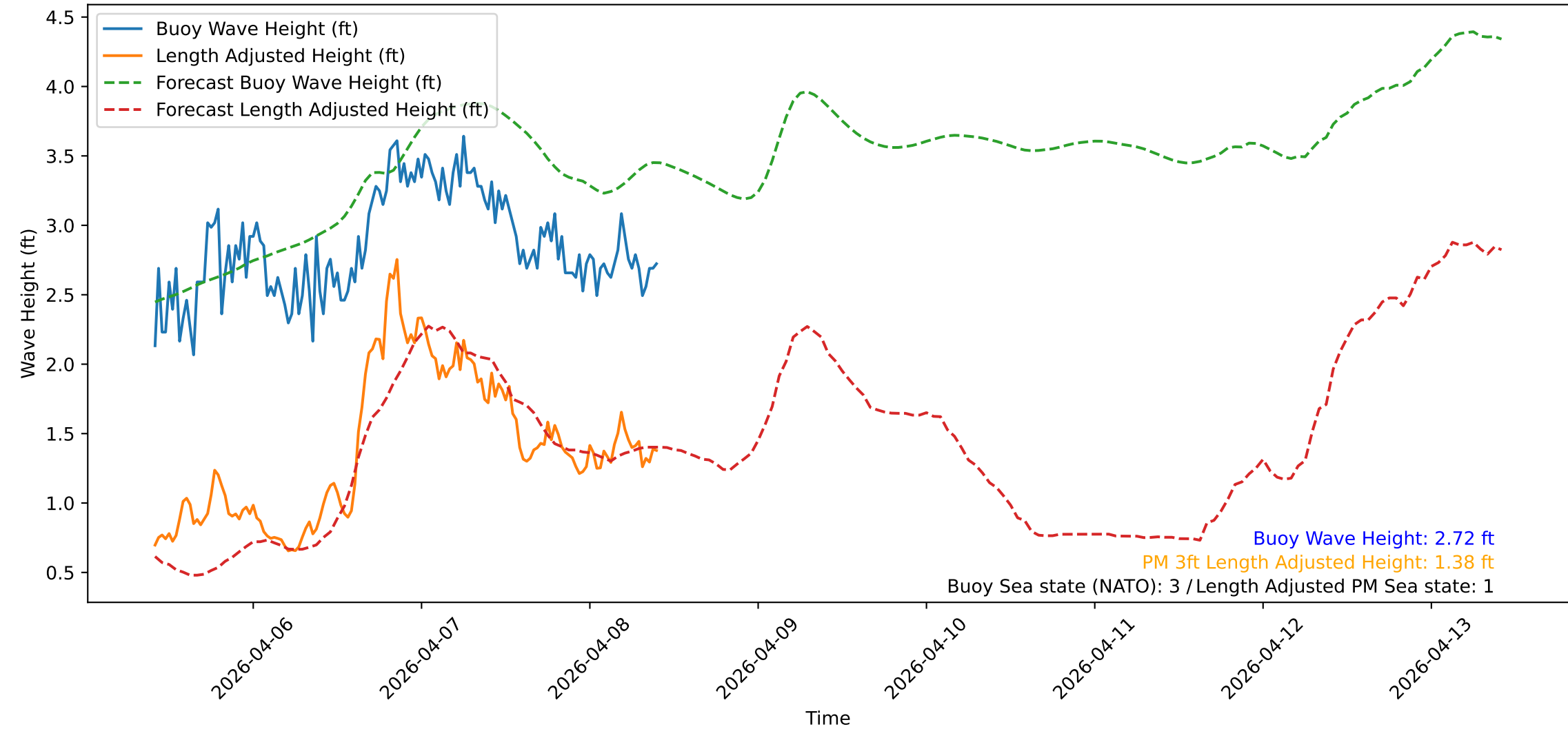
Wave Heights over Time for Oceanside Harbor at 2026-04-08 10:10:31
