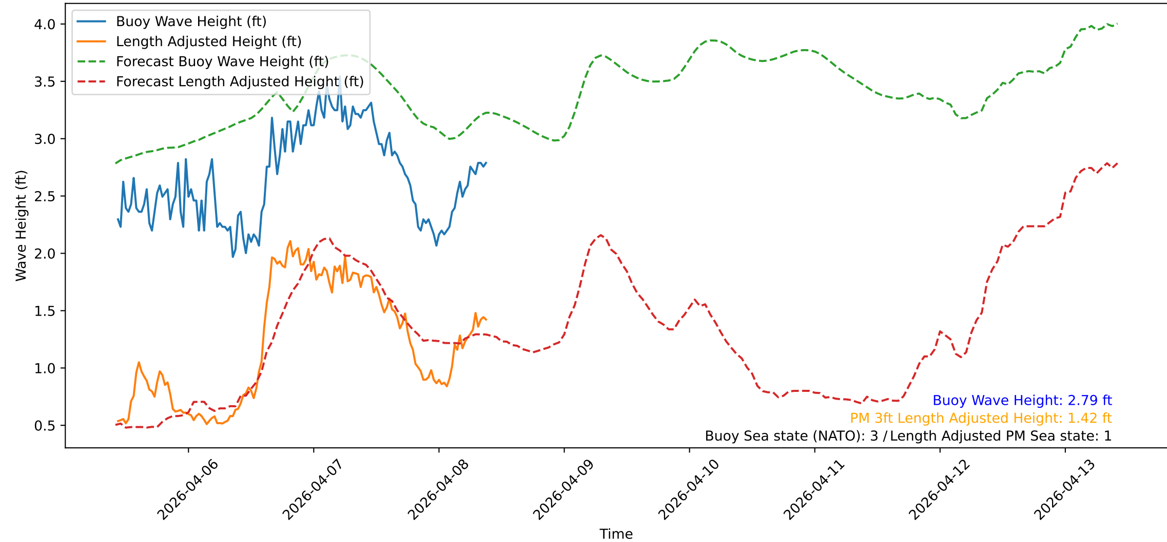
Wave Heights over Time for Red Beach at 2026-04-08 10:10:48
