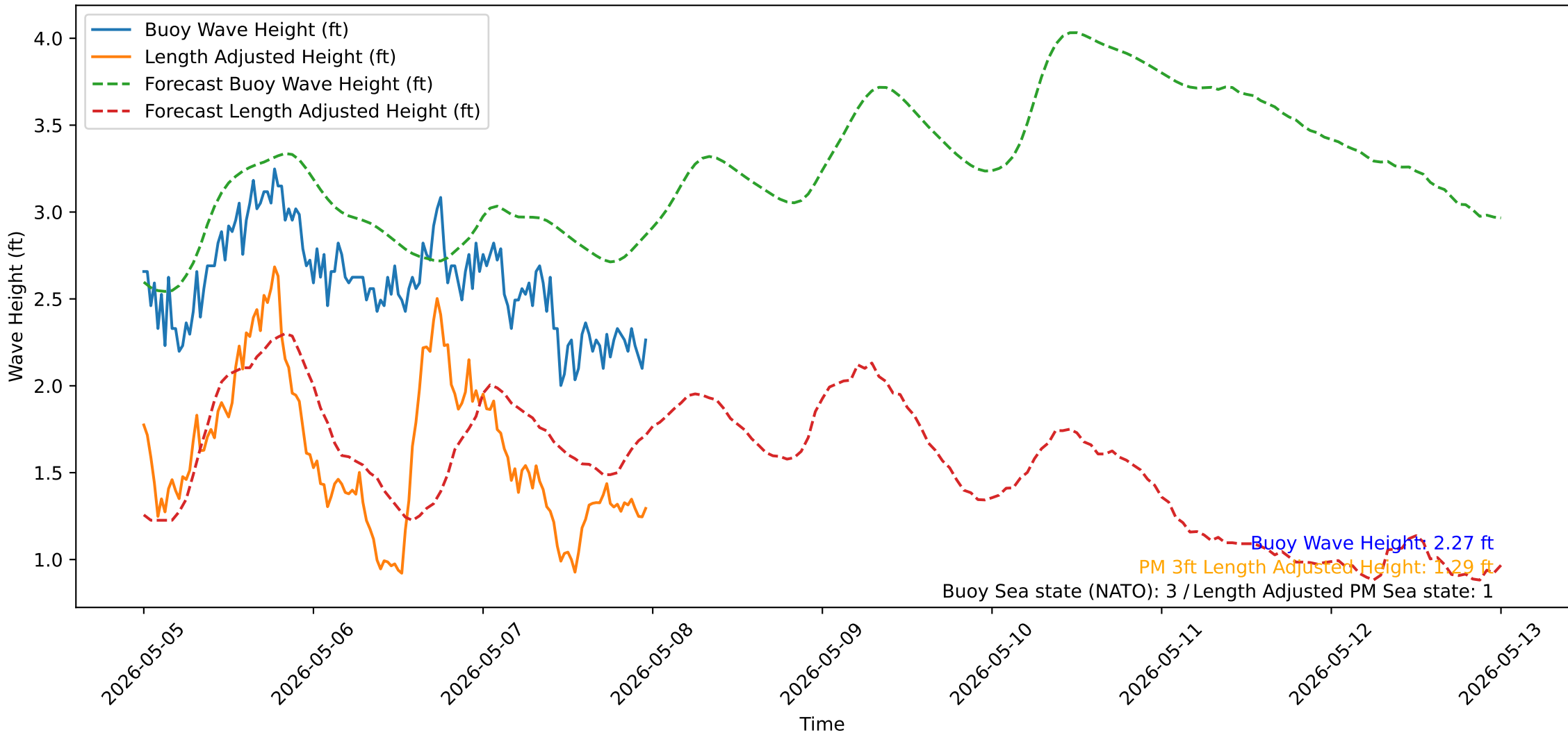
Wave Heights over Time for Oceanside Harbor at 2026-05-07 23:50:30
