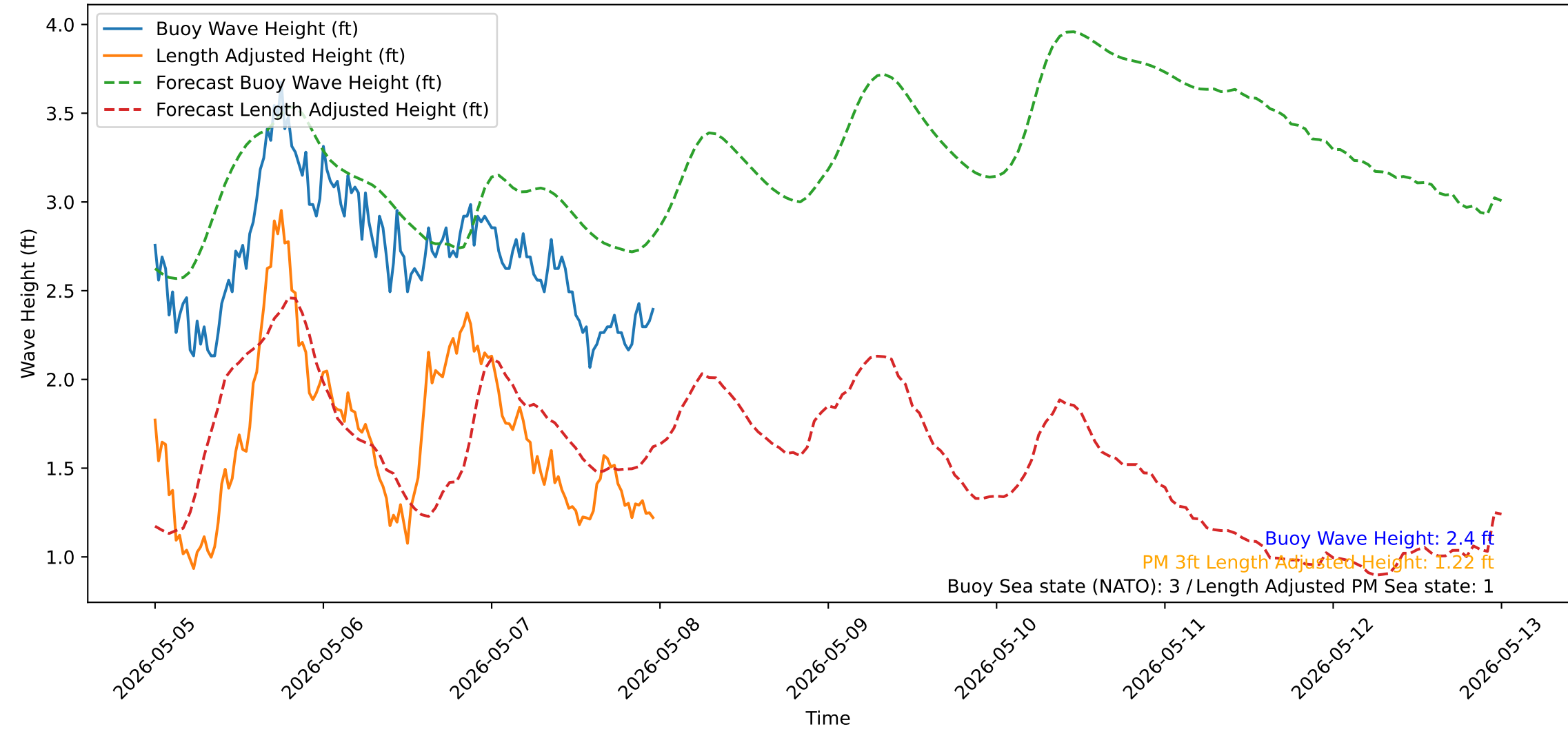
Wave Heights over Time for Green Beach at 2026-05-07 23:51:13
