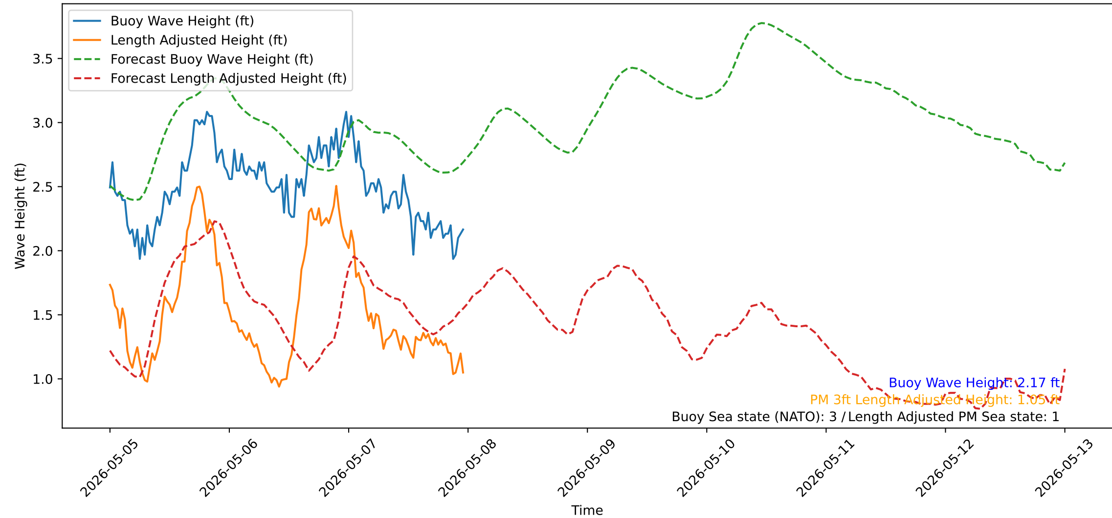
Wave Heights over Time for Red Beach at 2026-05-07 23:50:50
