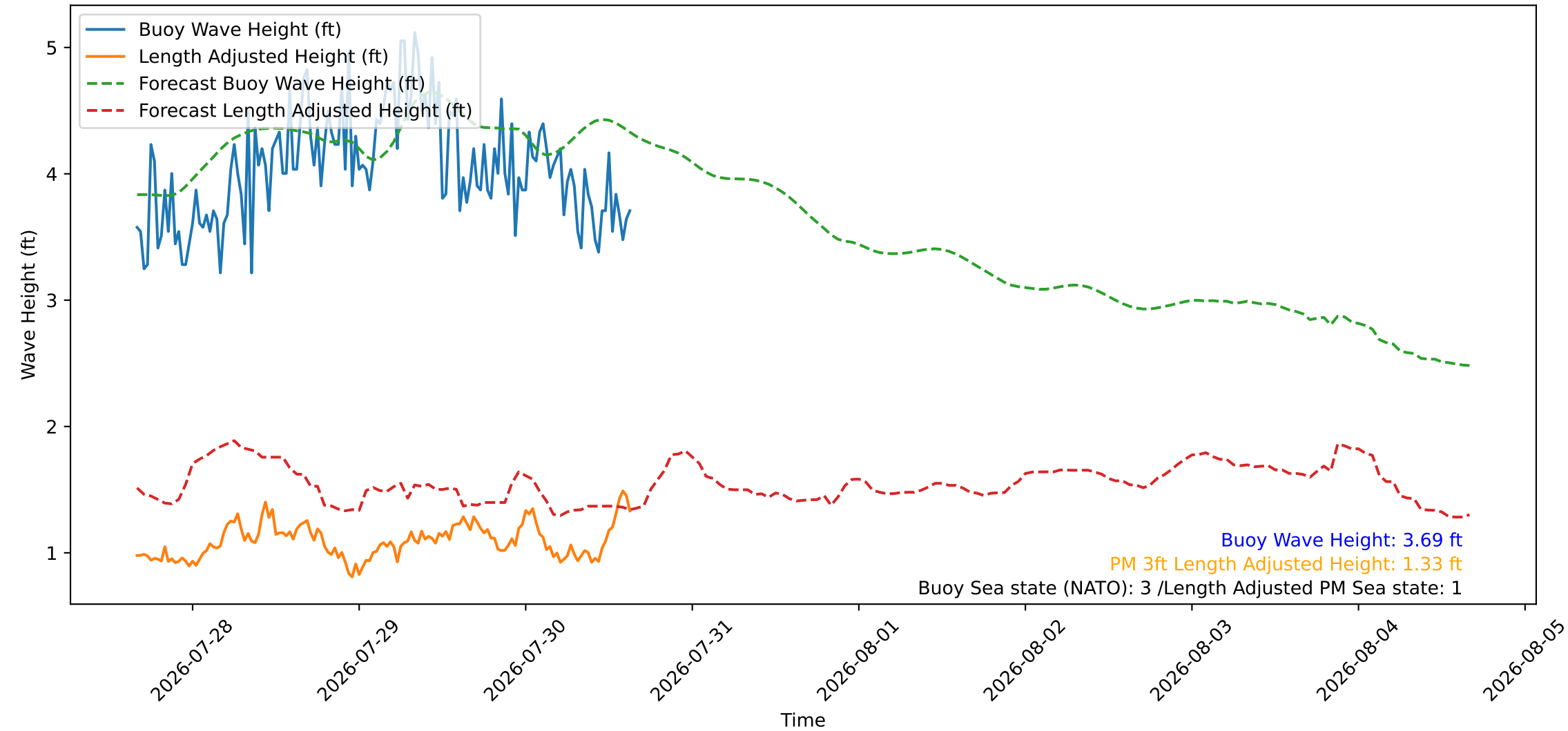
Wave Heights over Time for Red Beach at 2026-07-30 15:40:46
