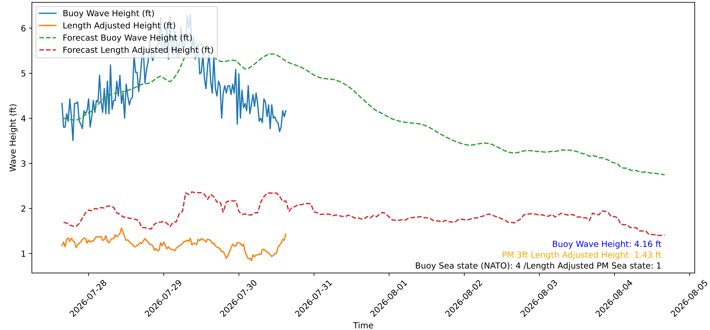
Wave Heights over Time for Green Beach at 2026-07-30 15:41:10
