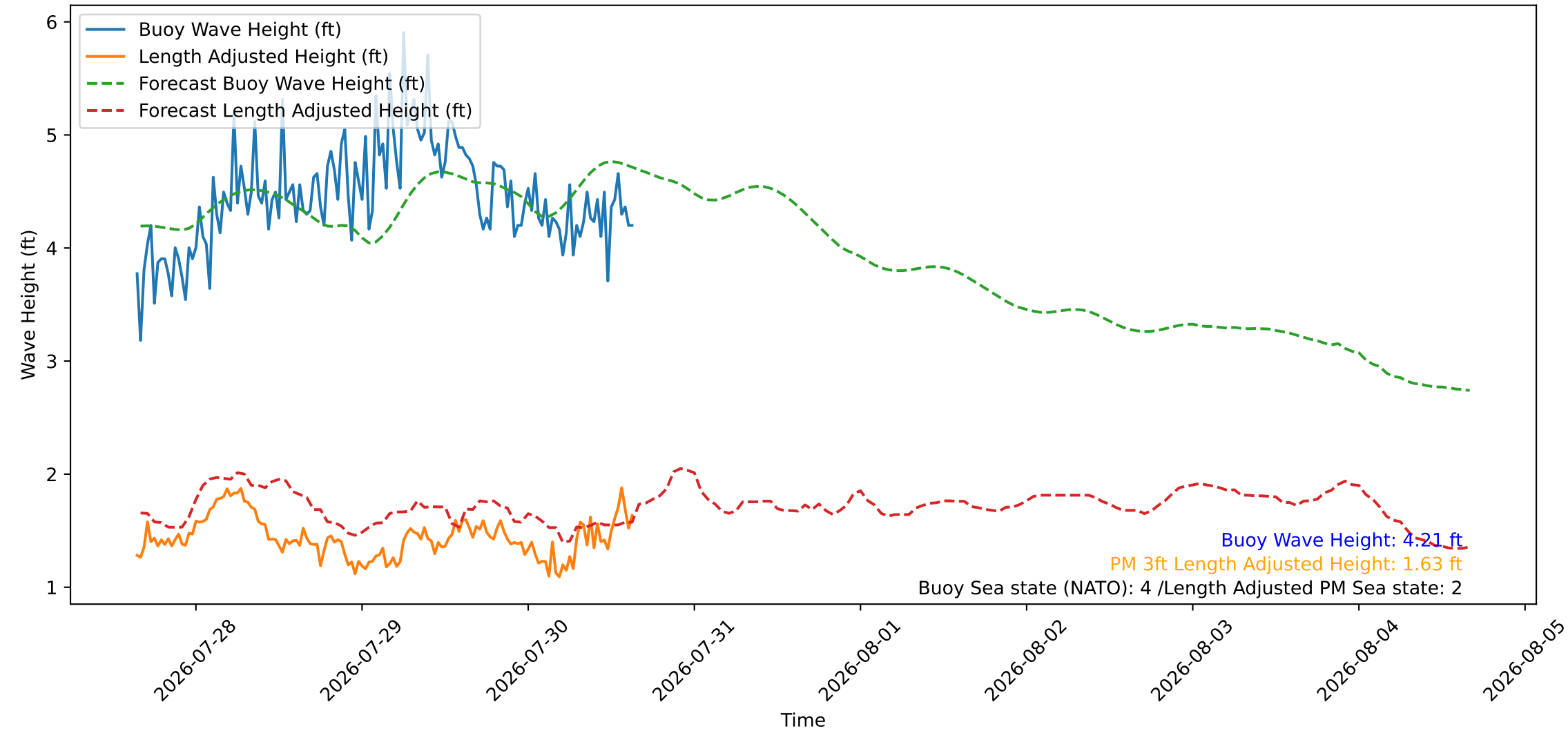
Wave Heights over Time for Oceanside Harbor at 2026-07-30 15:40:26
