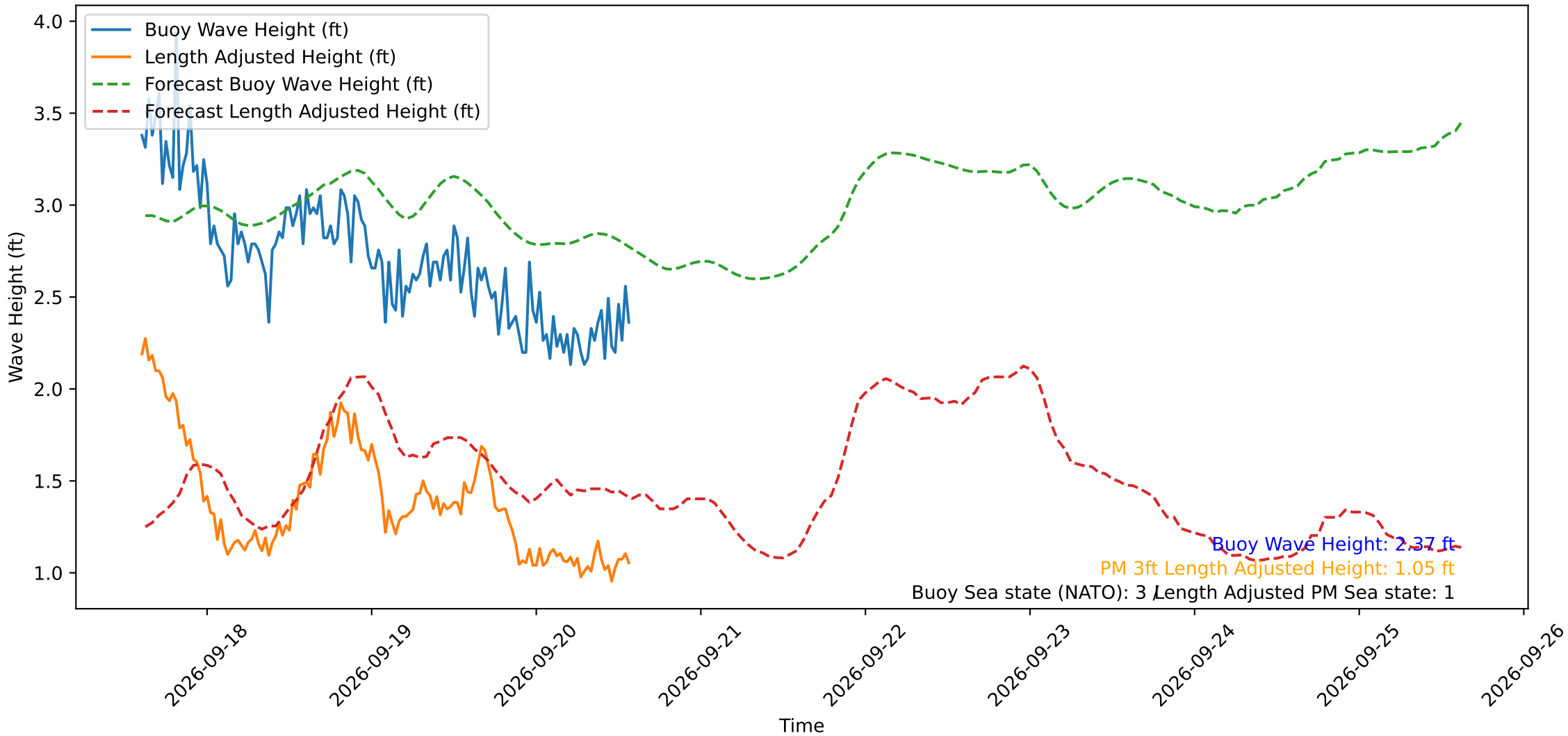
Wave Heights over Time for Oceanside Harbor at 2026-09-20 14:30:29
