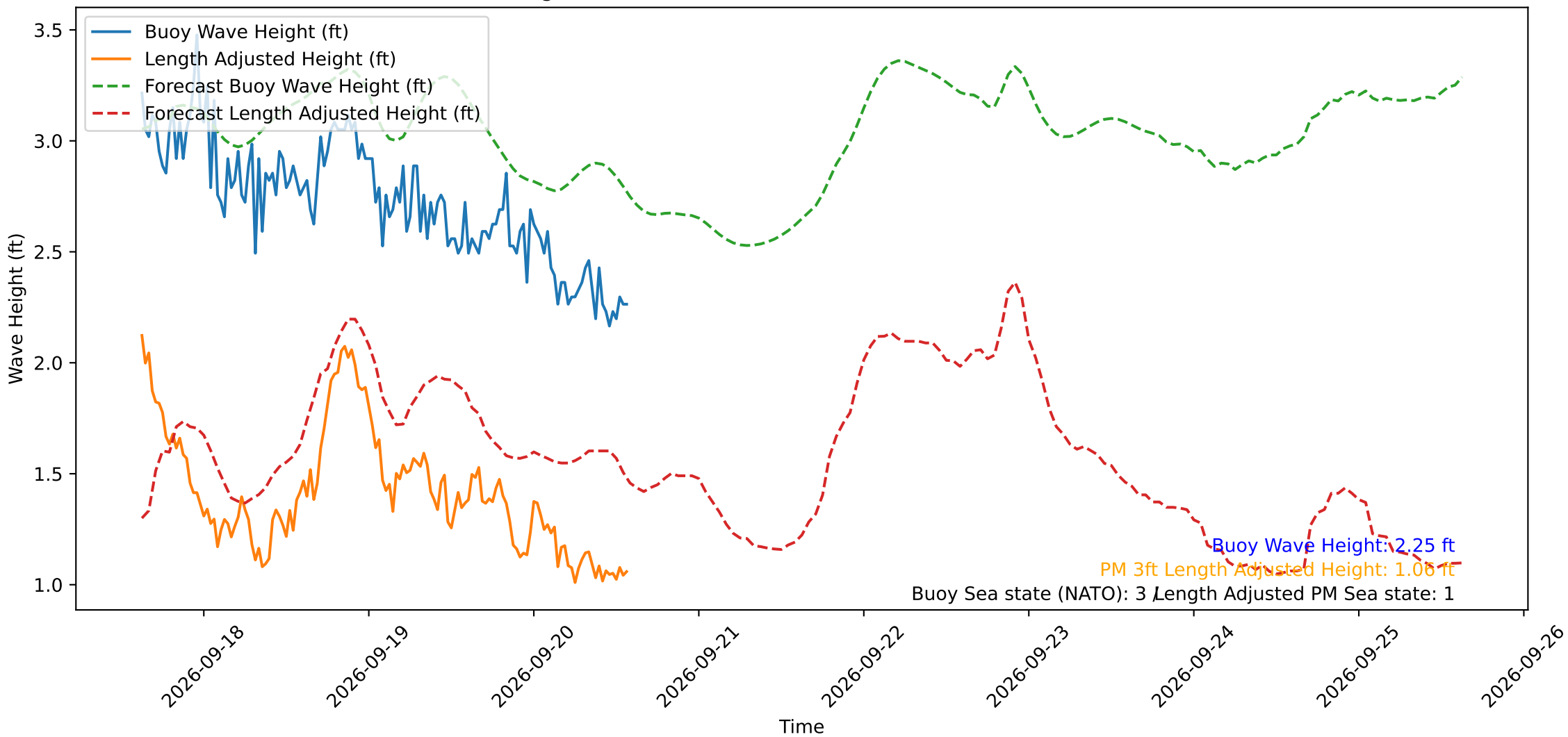
Wave Heights over Time for Green Beach at 2026-09-20 14:31:11
