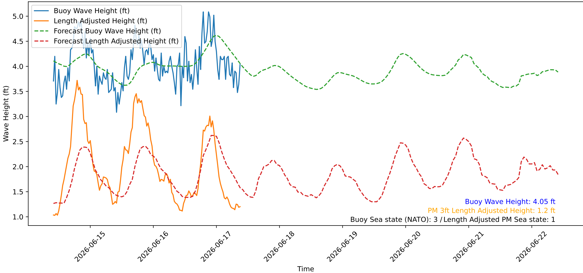
Wave Heights over Time for Green Beach at 2026-06-17 09:51:10
